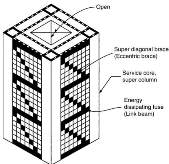
Figure 4.15. Eccentric bracing system for super-tall buildings.
