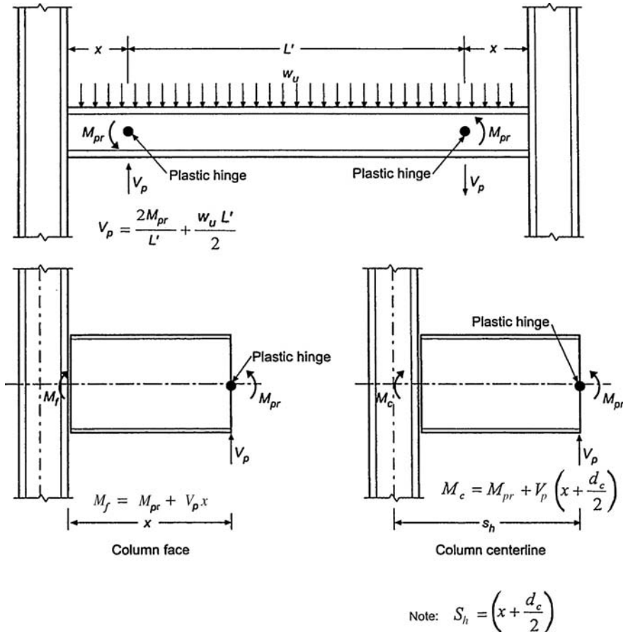
Figure 3.60. Calculation of shear and moment demands at critical sections of SMF.
