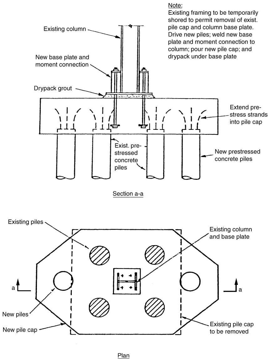
Figure 6.14. Upgrading of an existing pile foundation. Add additional piles or piers, remove, replace, or enlarge existing pile caps.
