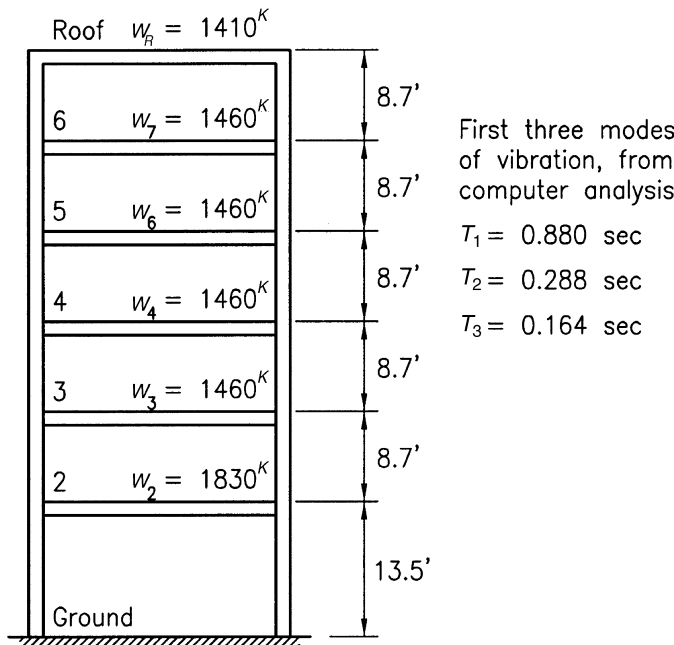
Figure 2.55. Seven-story building example; dynamic analysis.
