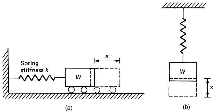
Figure 2.66. Analytical models for single-degree-of-freedom stem: (a) model in horizontal position; (b) model in vertical position.
