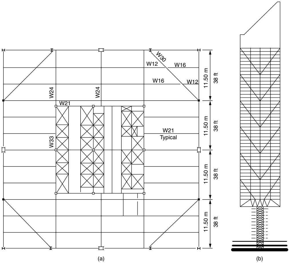
Figure 3.37. Citicorp Center (Structural Engineers, LeMessurier Consultants, Inc.): (a) typical floor framing plan; (b) elevation; (c) lateral bracing system.
