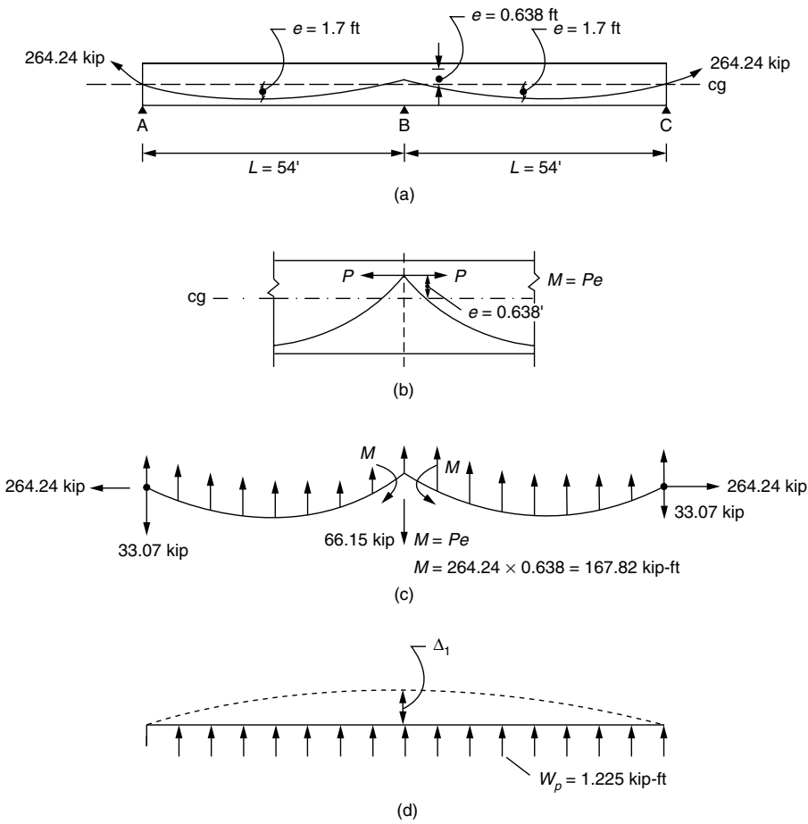
Figure 7.31C. Concept of secondary moments—example 3: (a) two-span continuous beam; (b) equivalent moment M = Pe at center of span; (c) equivalent loads and moments; (d) upward deflection \Delta_1 due to W_p ; (e) downward deflection \Delta_2 due to a load of 66.15 at center of span; (f) downward deflection \Delta_3 due to moments M = Pe at center of span; (g) load P_s corresponding to \Delta_1 - \Delta_2 - \Delta_3 ; (h) secondary moments.
