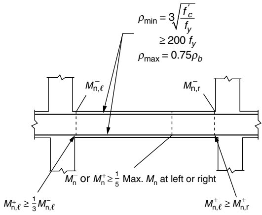
Figure 4.20. Intermediate moment-resisting frame (IMRF); flexural reinforcement requirements for frame beams.
