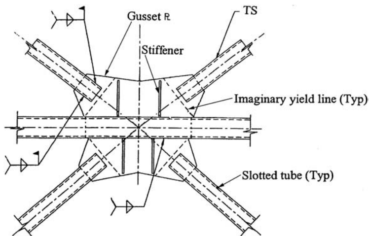
Figure 3.48. X-brace-to-beam connection. (Courtesy of Louis Choi, S.E., John A. Martin & Assoc. Structural Engineers, Los Angeles, CA.)
