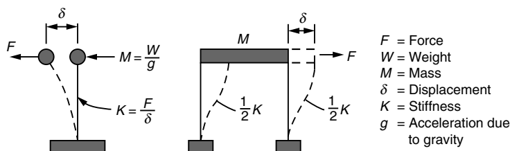
Figure 2.11. Idealized single-degree-of-freedom system.
