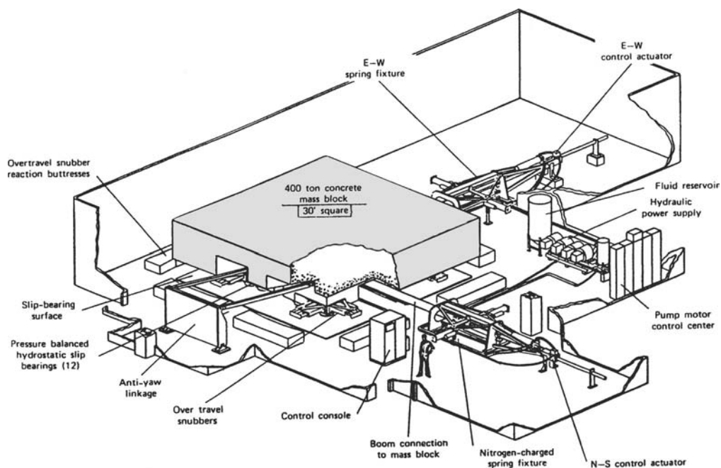
Figure 8.30c. Schematic view of a TMD operating on top of the Citicorp Center. The TMD consists of a 400-ton concrete block bearing on a thin film of oil. The structural stiffness of the TMD is aided by pneumatic springs tuned to the frequency of the building. The TMD damping system is aided by shock absorbers.
