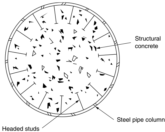
Figure 5.2. Concrete-filled composite pipe column.
