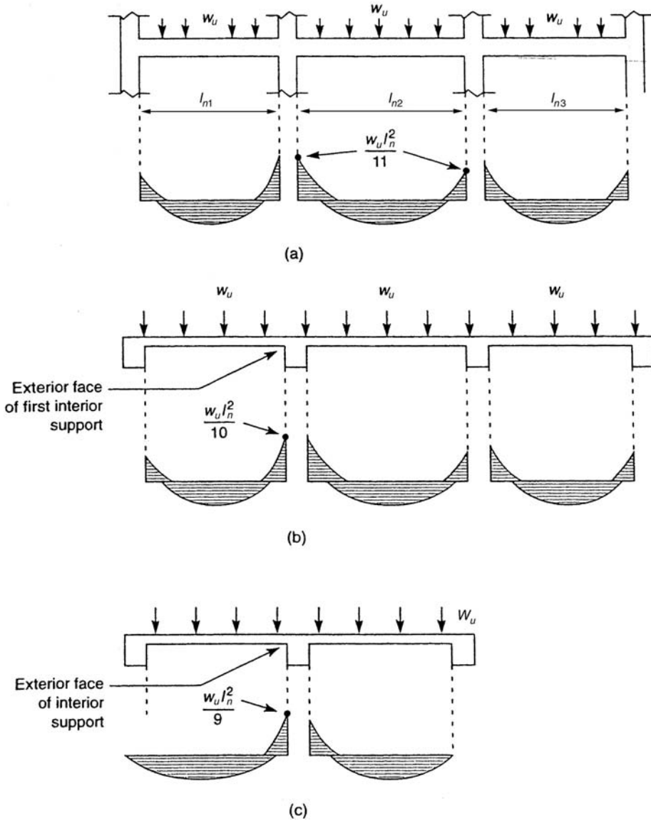
Figure 7.12. ACI coefficients for negative moments: (a) at interior supports; (b) at exterior face of first interior support, more than two spans; (c) at exterior face of first interior support, two spans.
