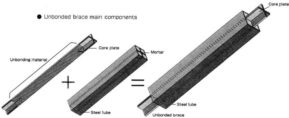
Figure 8.36a. Main components of unbonded brace.
