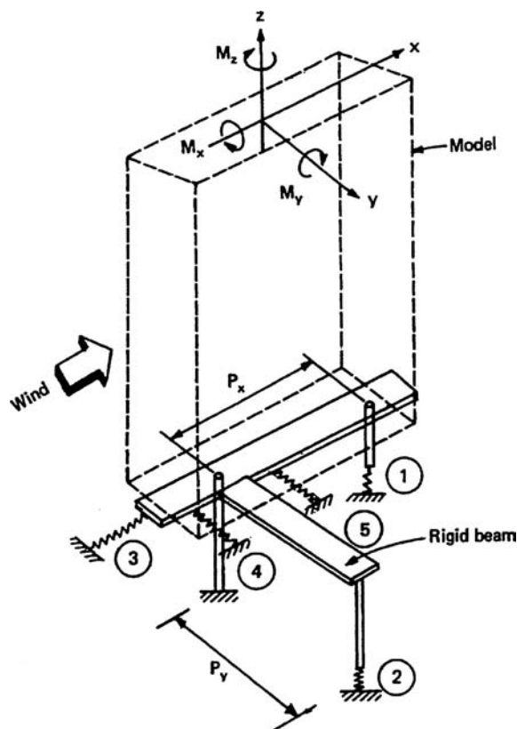
Figure 1.29. Schematic representation of five-component force balance model.
