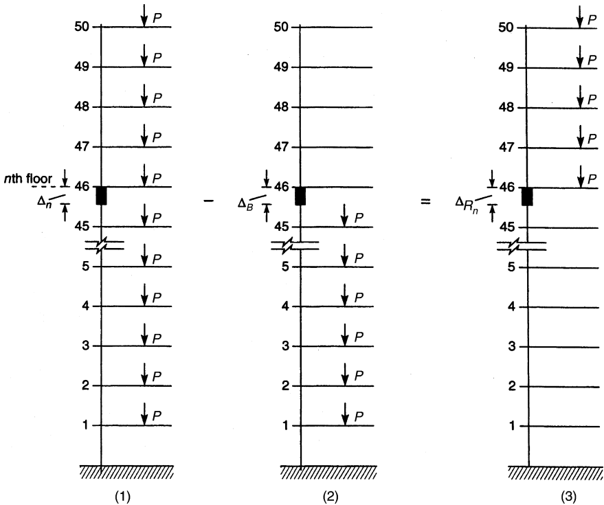
Figure 8.321. Physical interpretation of column overlength: (1) column shortening due to loads at all floors; (2) column shortening due to loads below the n th level; (3) column residual overlength \Delta_{R_n} = \Delta_n - \Delta_B .
