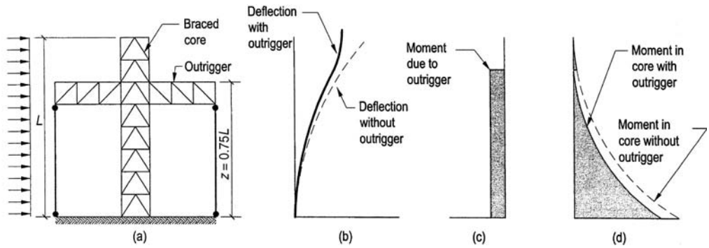
Figure 3.20. Outrigger, three-quarters up the height, z = 0.75L .
