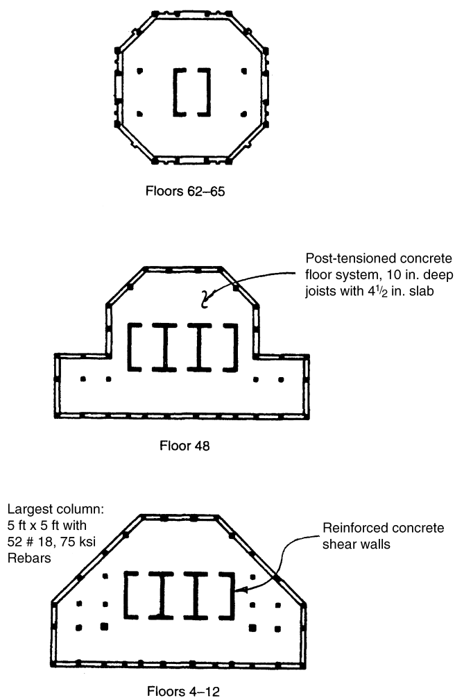
Figure 8.7. South Walker Tower, Chicago; schematic plans.
