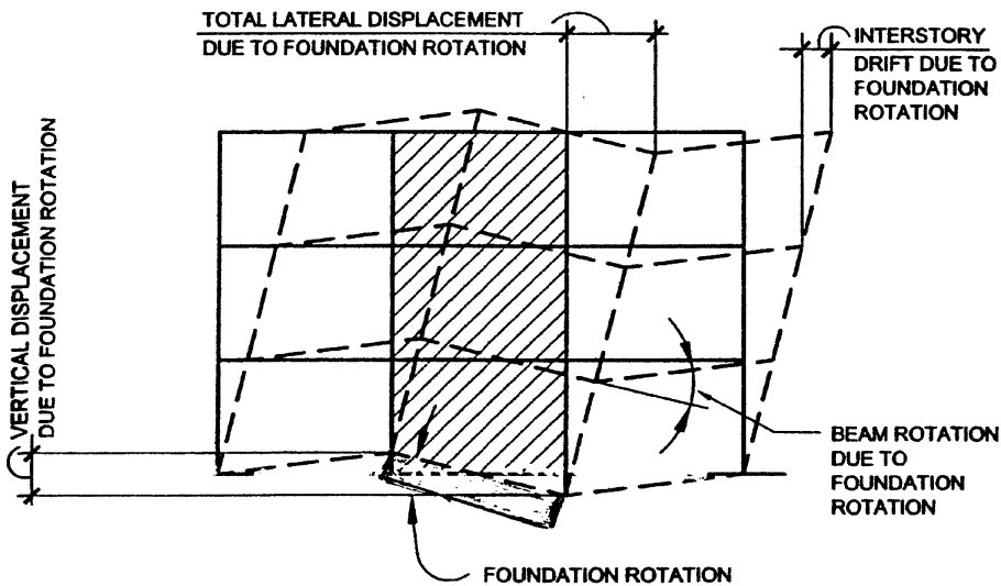
Figure 2.41. Deformation compatibility consideration of foundation flexibility. (Adapted from SEAOC Blue Book, 1999 Edition.)
