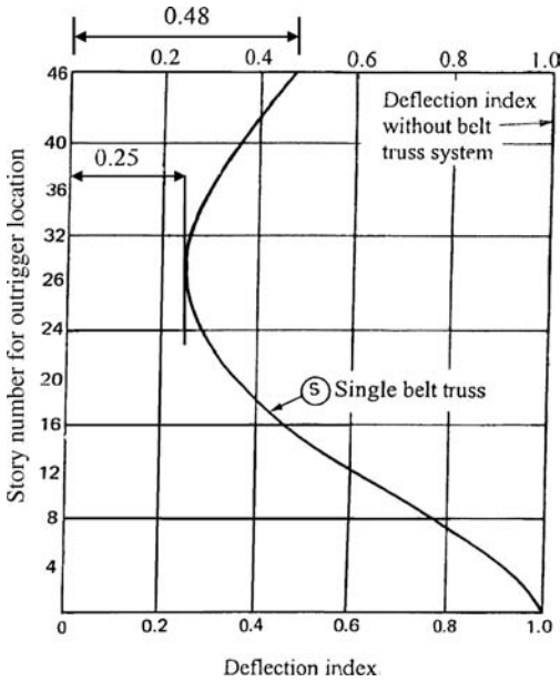
Figure 3.26. Deflection index versus level of outrigger location.
