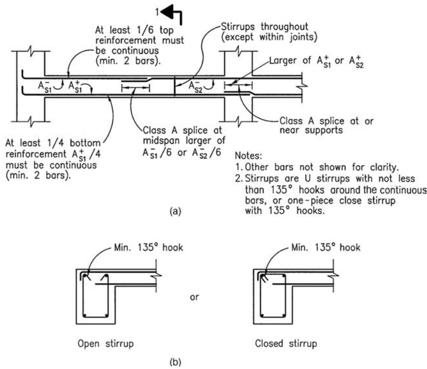
Figure 4.18. Integrity reinforcement in perimeter beams: (a) perimeter beam elevation; (b) Section 1.
