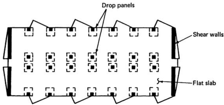
Figure 4.3. Shear wall–flat slab system.
