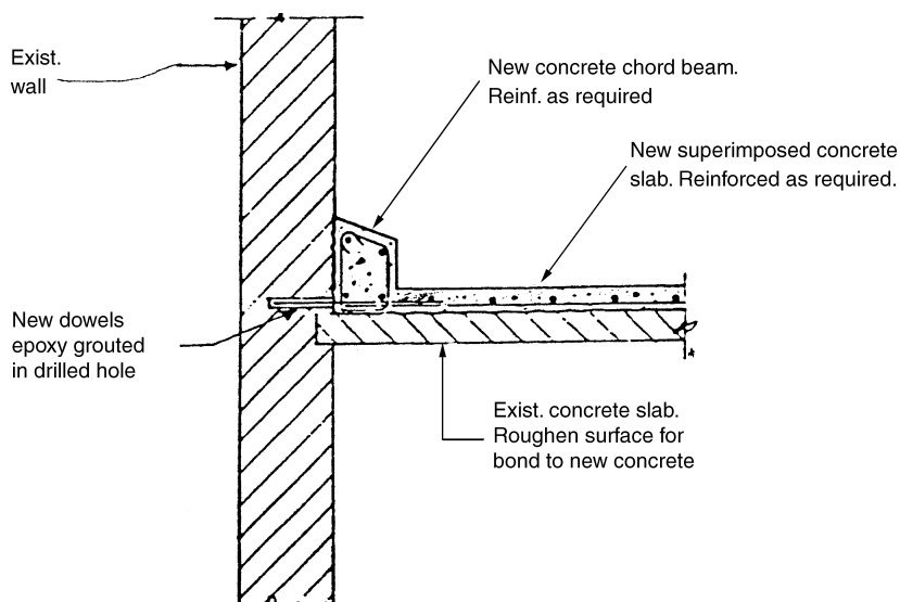
Figure 6.2. Superimposed diaphragm slab at an existing concrete wall.
