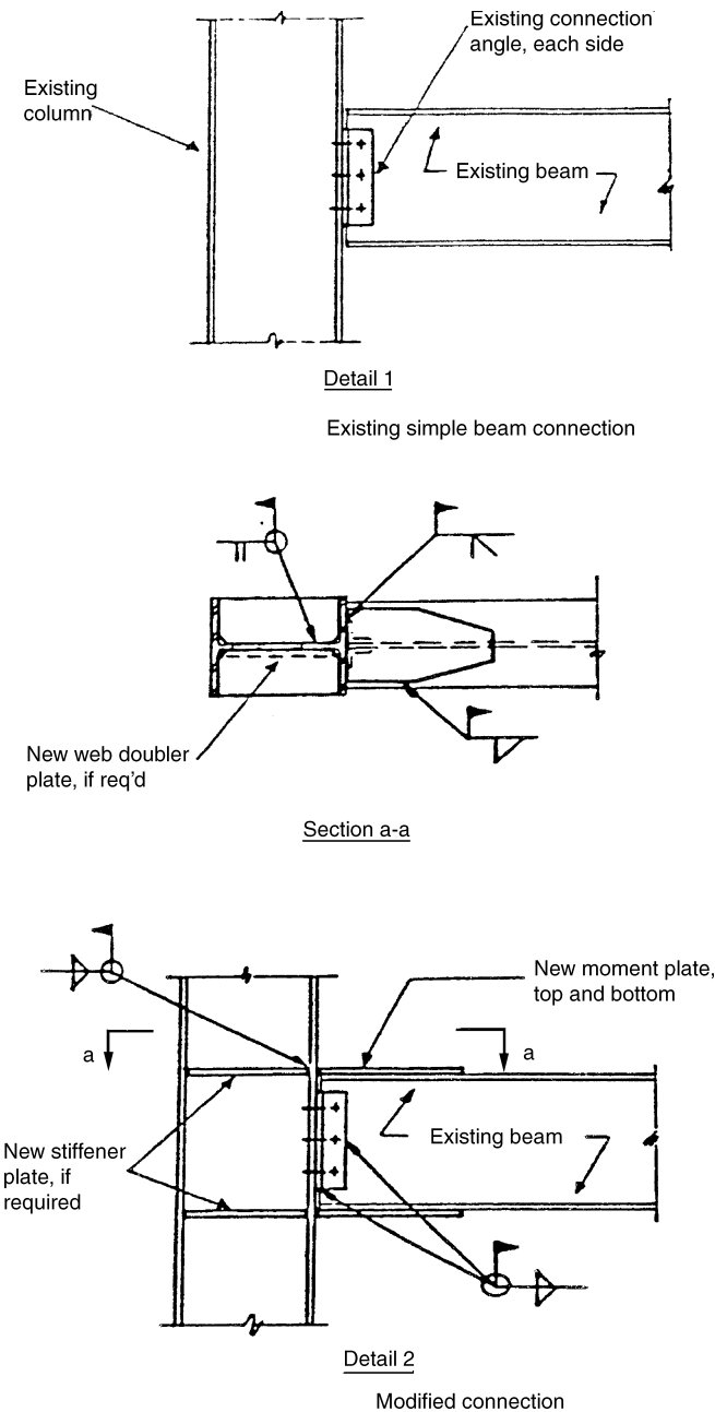
Figure 6.20. Modification of an existing simple beam connection to a moment connection.
