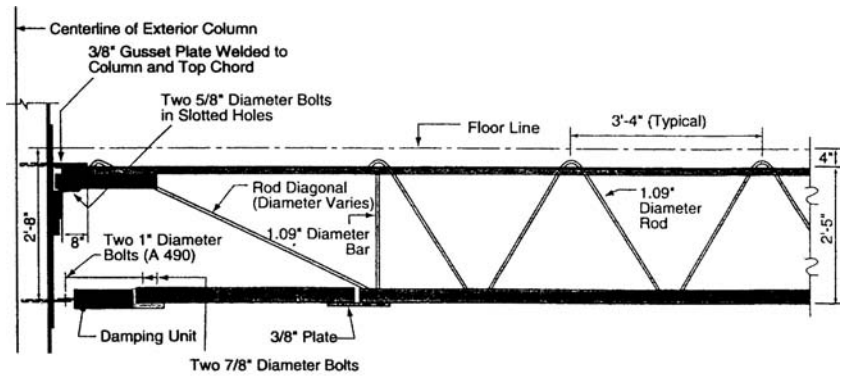
(i) Detail A - Exterior Wall End Detail
