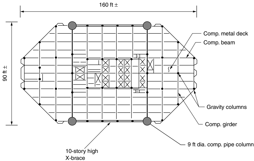
Figure 5.16. Gateway Tower; 62-story building.
