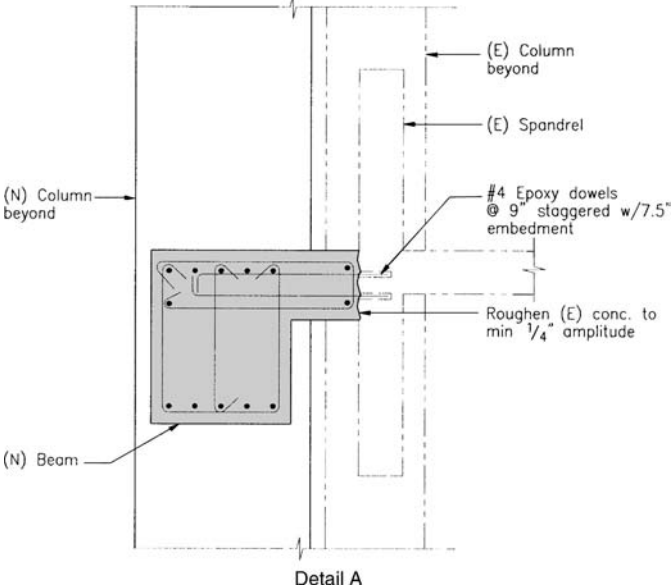
Figure 6.12e. Connection between (N) and (E) frame.
