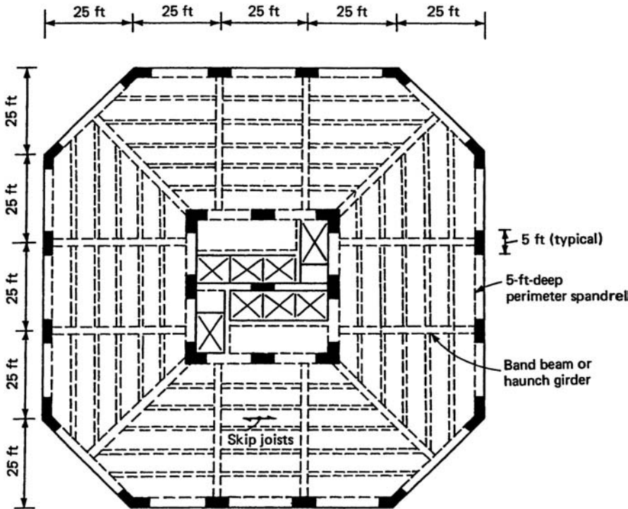
Figure 4.4. Tube building with widely spaced perimeter columns.
