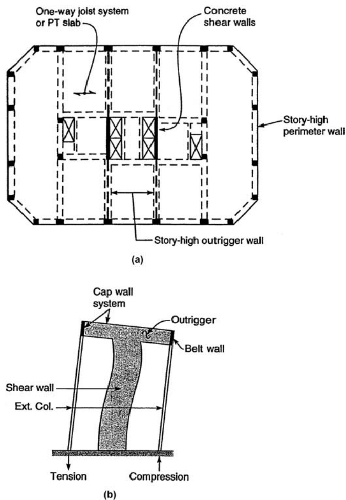
Figure 4.10. Building with cap wall: (a) schematic plan; (b) structural behavior.
