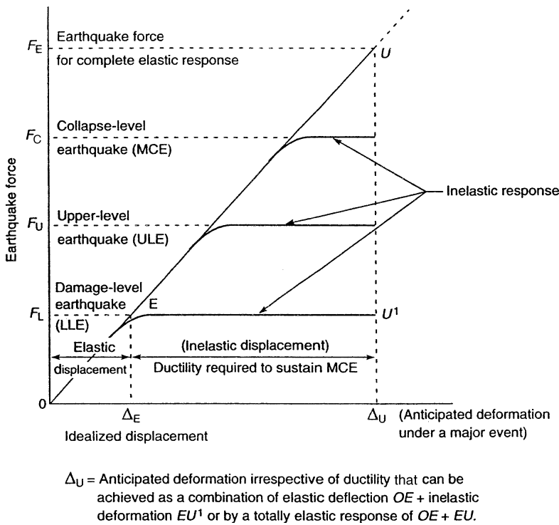
Figure 6.1. Idealized earthquake force-displacement relationships.
