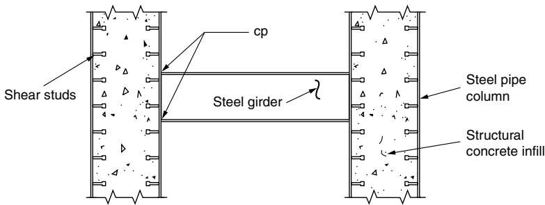
Figure 5.4. Composite column-to-steel girder moment connection.
