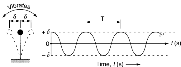
Figure 2.12. Undamped free vibrations of a single-degree-of-freedom system.
