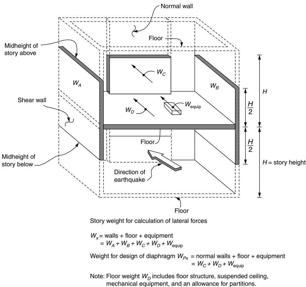
Figure 2.39. Tributary weights for seismic dead load calculation.
