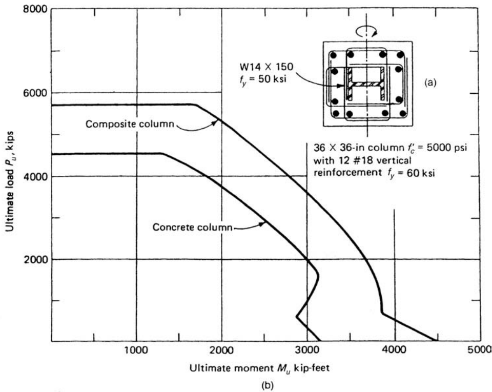
Figure 7.65. Comparison of interaction diagrams: (a) column detail; (b) load moment interaction diagram.
