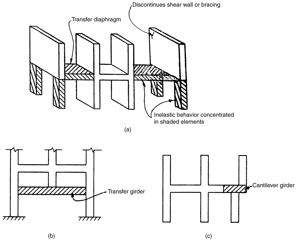
Figure 2.34. Irregularity due to out-of-plane offsets of vertical elements. This irregularity exists when there is discontinuity in the lateral-load-resisting path. In this figure, the columns and other elements such as the transfer girder and the cantilever girder support a discontinuous wall or a frame-column. They must be designed for special seismic load combination given in the 1997 UBC and ASCE 7-02.
