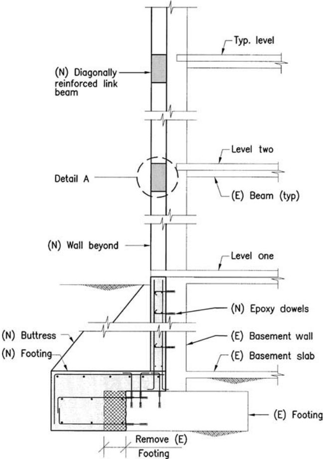
Figure 6.12d. Section through transverse wall.
