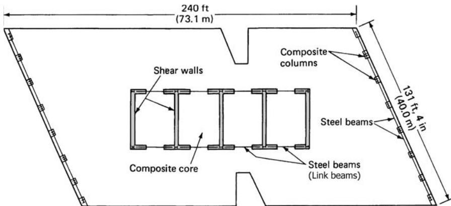
Figure 5.23. Composite elements.
