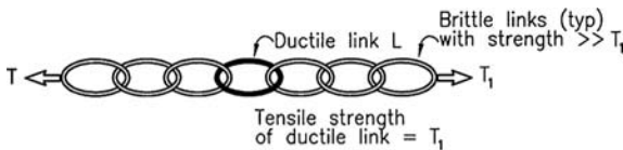
Figure 3.51a. Chain with ductile and brittle links.
