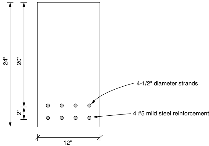
Figure 7.48a. Example 1: beam section.
