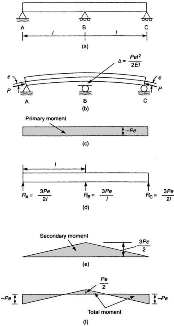
Figure 7.30. Concept of secondary moment: (a) two-span continuous beam; (b) vertical upward displacement due to PT; (c) primary moment; (d) reactions due to PT; (e) secondary moment; (f) final moments.
