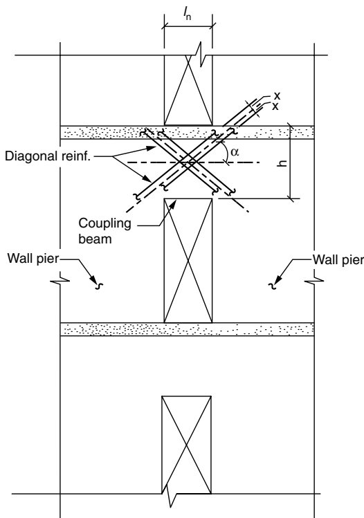
Figure 4.47. Geometry for calculating \alpha , the angle between diagonal reinforcement and the longitudinal axis of the coupling beam.
