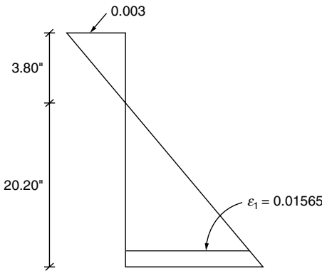
Figure 7.48i. Example problem 3: strain diagram; second trial.
