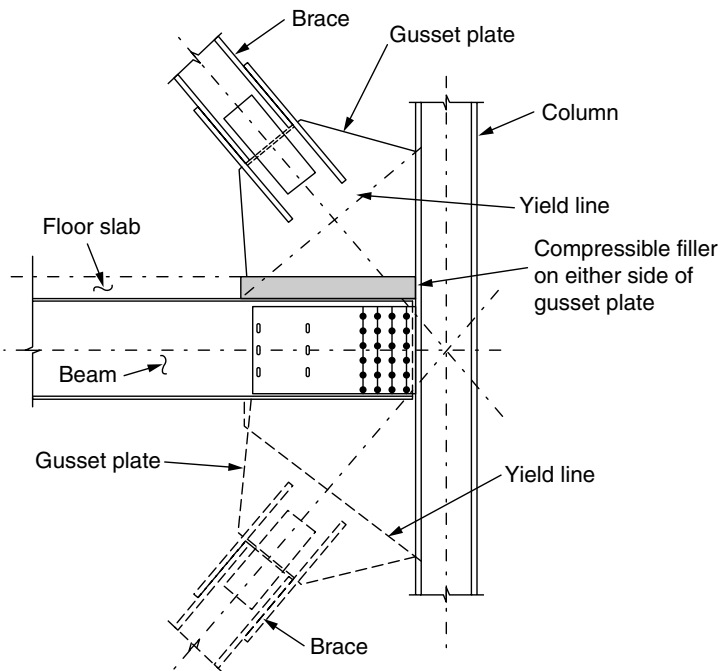
Figure 3.40b. Gusset plate isolation from floor slab.
