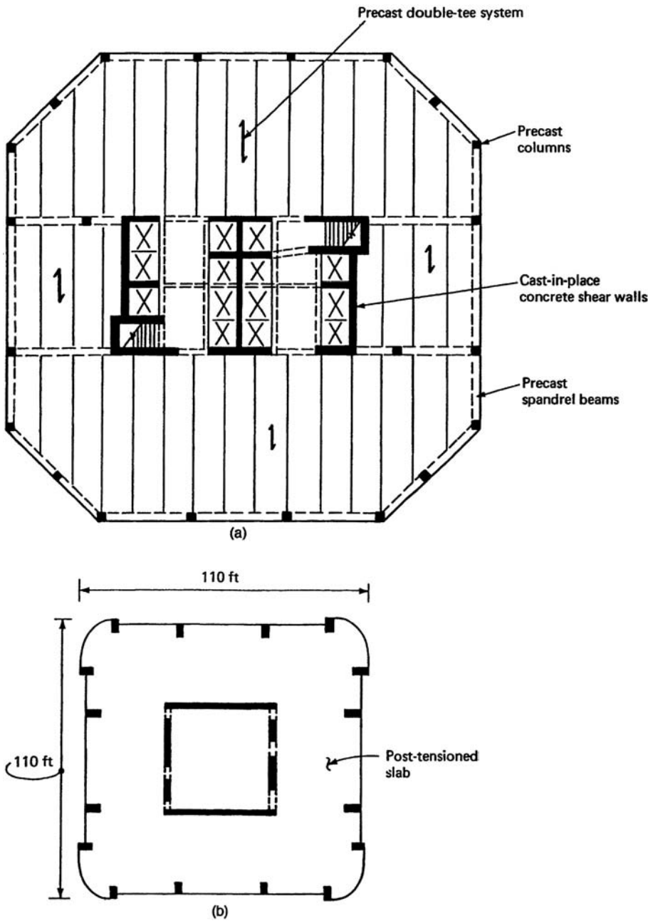
Figure 4.6. Examples of shear core buildings: (a) cast-in-place shear walls with precast surround; (b) shear walls with post-tensioned flat plate; (c) shear walls with one-way joist system.
