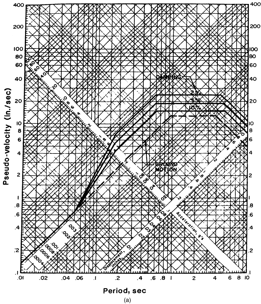
Figure 2.24. Tripartite site-specific response spectra: (a) earthquake A; (b) earthquake B; (c) earthquake C; (d) earthquake D.
