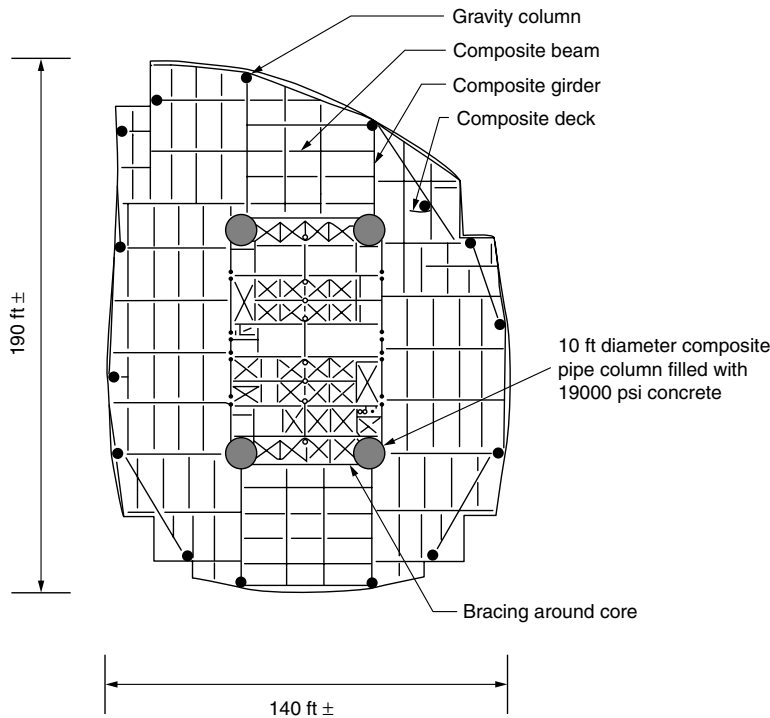
Figure 5.17. Two Union Square; 58-story building.
