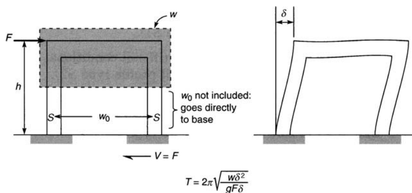
Figure 2.37. Period calculation for a single-degree-of-freedom system. Rayleigh's formula.
