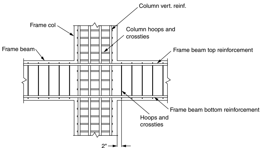
Figure 4.41. Beam-column joint; special moment frame. Transverse reinforcing in the joint is the same as for the frame column. A 50% reduction is allowed if the joint is confined on all the four faces. Maximum spacing of transverse reinforcement = 6 in.
