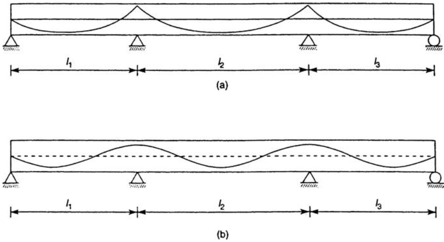
Figure 7.35. Tendon profile in continuous beams: (a) simple parabolic profile; (b) reverse curvature in tendon profile.
