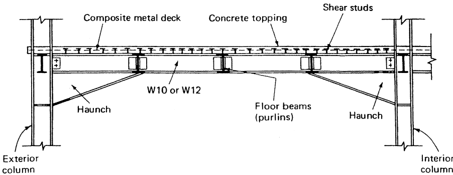
Figure 7.59. Composite girder with tapered haunch.
