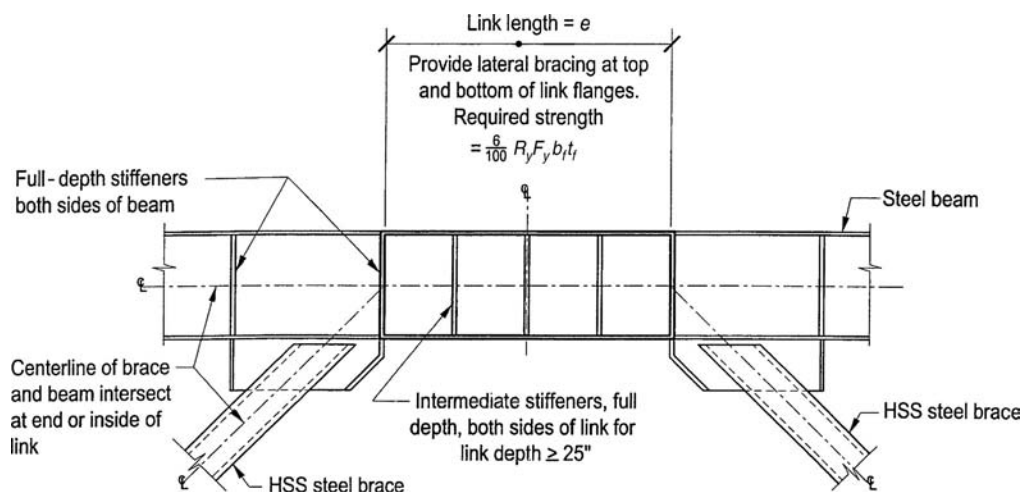
Figure 3.52. An EBF with HSS bracing; stiffener requirements.
