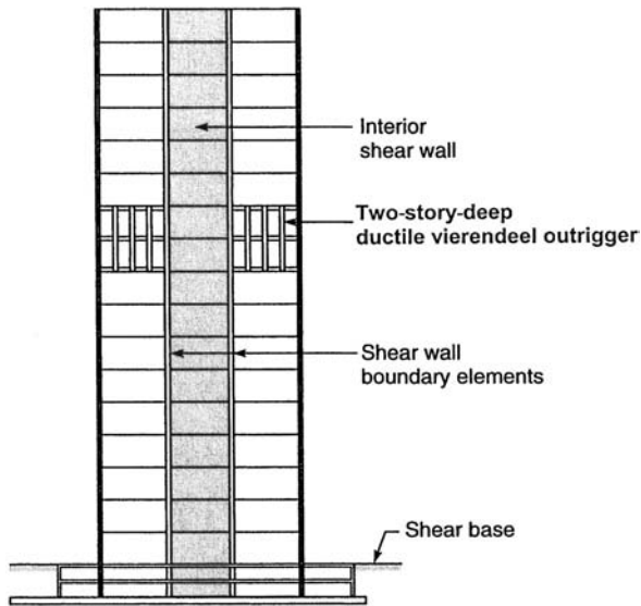
Figure 4.12. Outrigger system: seismic version.
