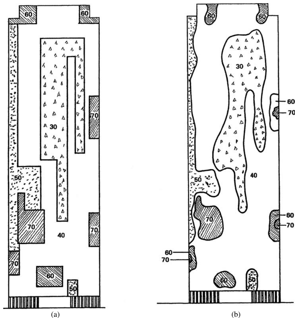
Figure 1.7. (a) Block pressure diagram, in psf; (b) Pressure contours in psf.
