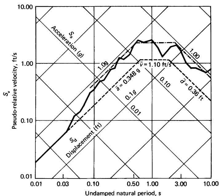
Figure 2.22. Tripartite response spectra for El Centro earthquake (5% damping, north-south component).
