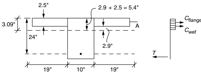
Figure 7.48g. Example problem 3: prestressed T-beam.
