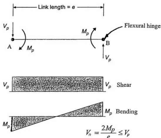
Figure 3.51b. Bending moments and shear forces in link beam. Flexural hinges form at A and B when both M_A and M_B reach the plastic moment M_p .
