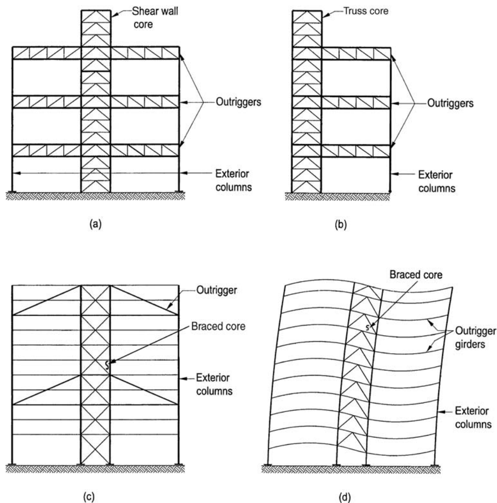
Figure 3.17. (a) Outrigger system with a central core; (b) outrigger system with offset core; (c) diagonals acting as outriggers; (d) floor girders acting as outriggers.
