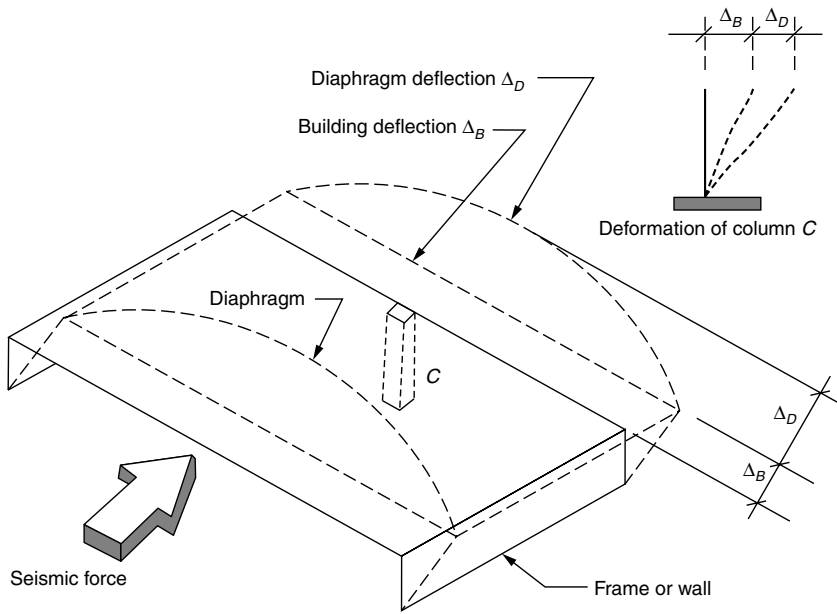
Figure 2.40. Column deformation for use in compatibility considerations. Deformation of column = building deflection \Delta_B + diaphragm deflection \Delta_D . (Adapted from SEAOC Blue Book, 1999 Edition.)
