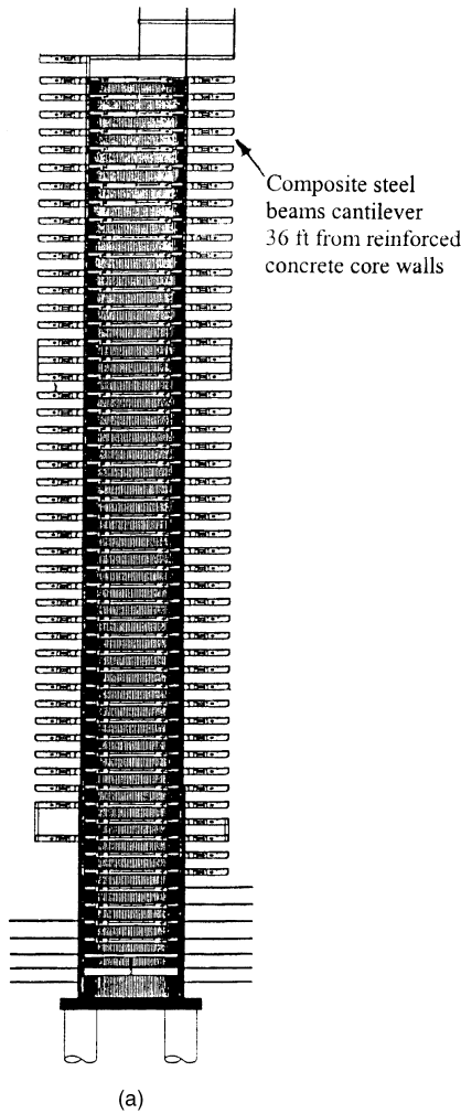
Figure 8.17. Singapore Treasury Building: (a) schematic section; (b) typical floor framing plan.
