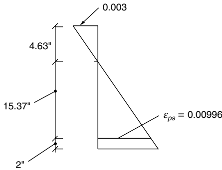
Figure 7.48f. Example 2: strain diagram, second trial.
