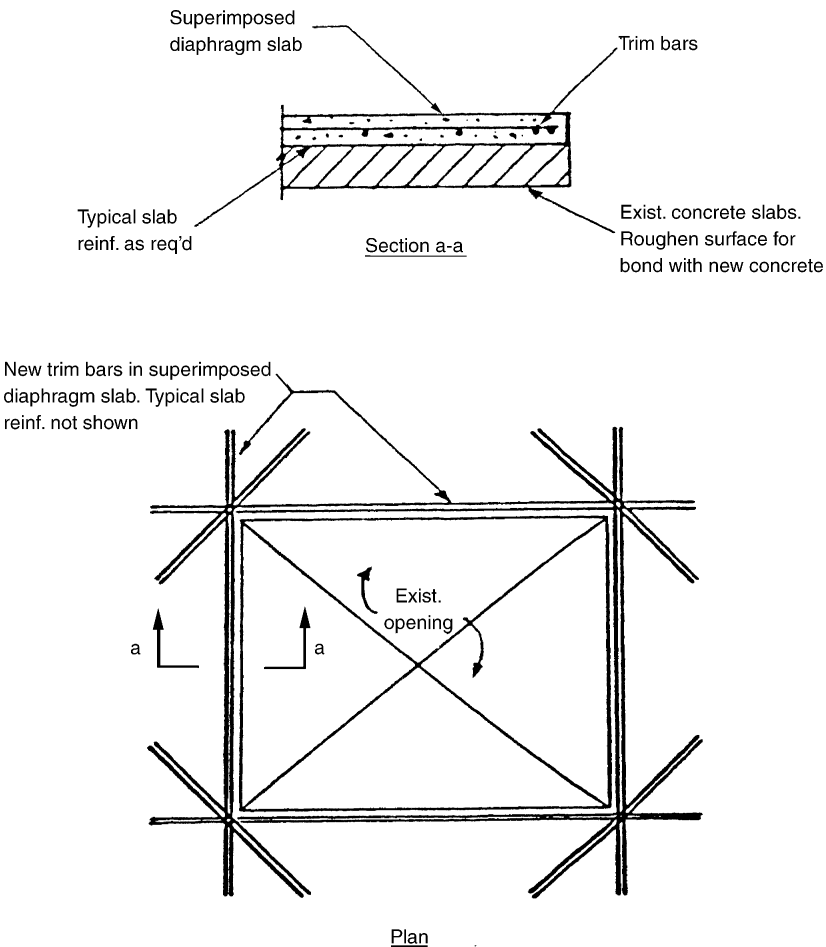
Figure 6.5. Strengthening of openings in a superimposed diaphragm.
