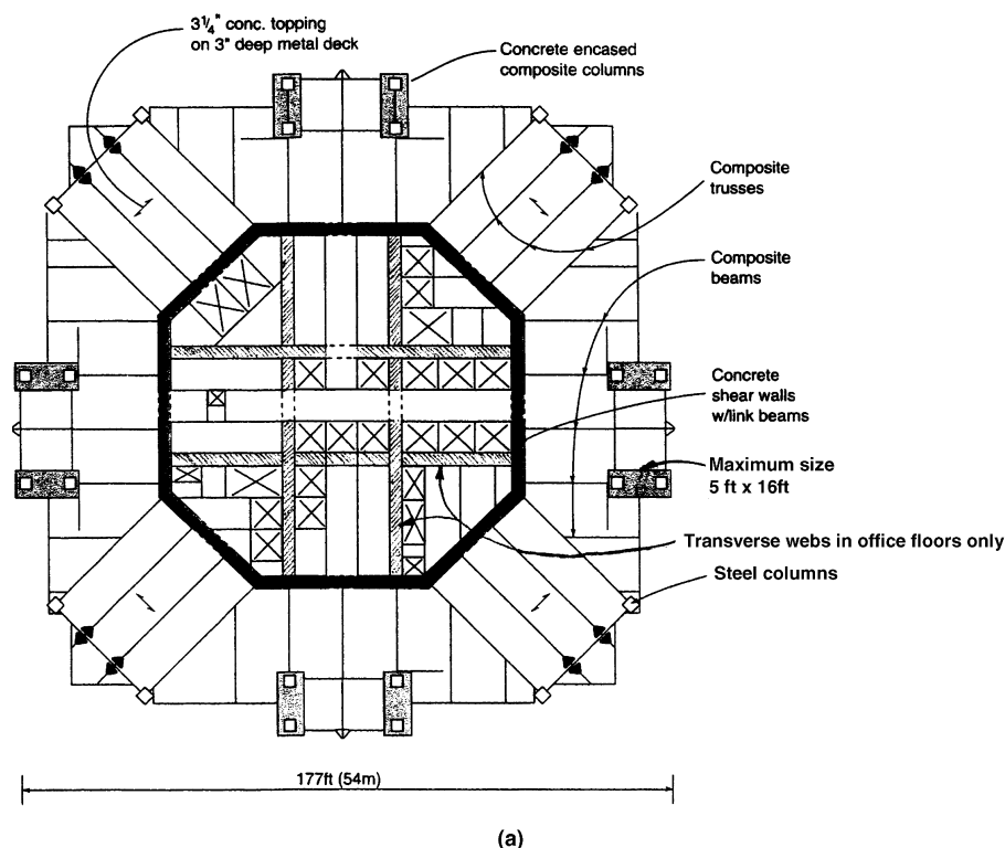
Figure 8.11. Jin Mao Tower, Shanghai, China: (a) typical office floor framing plan.
