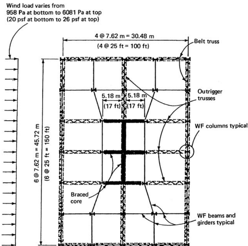
Figure 3.24. Schematic plan of a single outrigger building.
