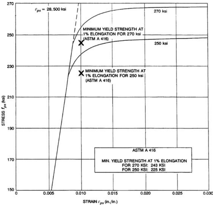
Figure 7.48. Typical stress-strain curve with seven-wire low-relaxation prestressing strand. These curves can be approximated by the following equations:
