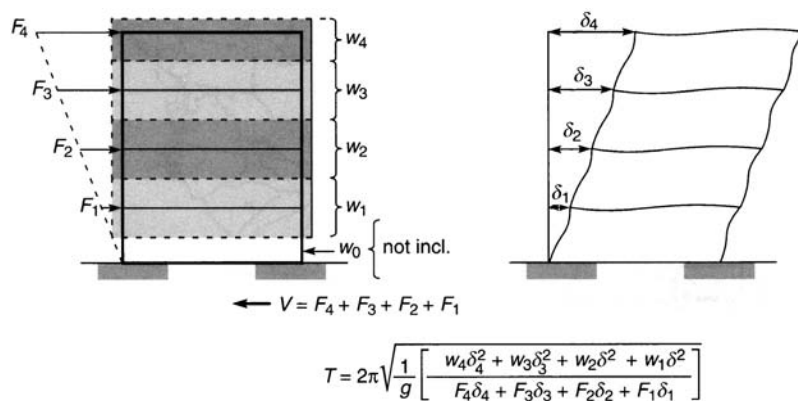
Figure 2.38. Period calculation for multidegree-of-freedom system. Rayleigh's formula.
