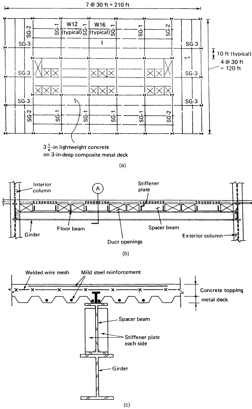
Figure 7.62. Stub girder framing: (a) framing plan; (b) elevation of stub girder SG-1; (c) section A through stub girder; (d) photograph showing stub girder framing prior to placement of metal deck.
