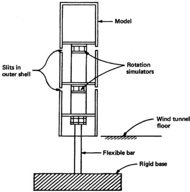
Figure 1.25. Rigid aeroelastic model with provisions for simulating torsion.
