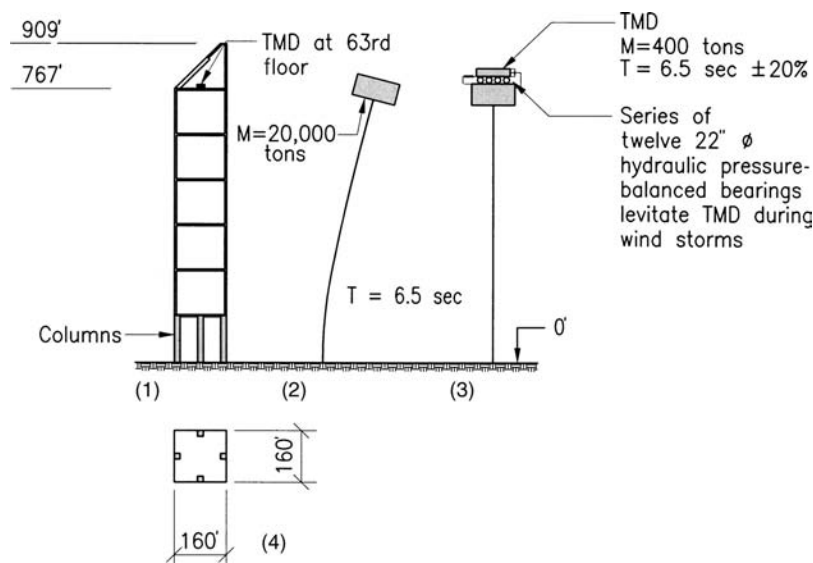
Figure 8.30b. Tuned mass damper for Citicorp Tower, New York: (1) building elevation; (2) plan; (3) first-mode response; (4) TMD atop the building.
