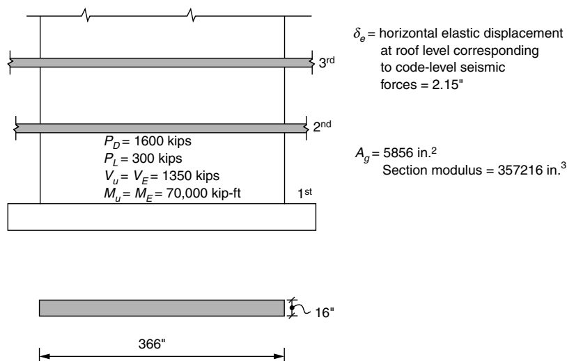
Figure 4.42. Design example; partial shear wall elevation and plan.
