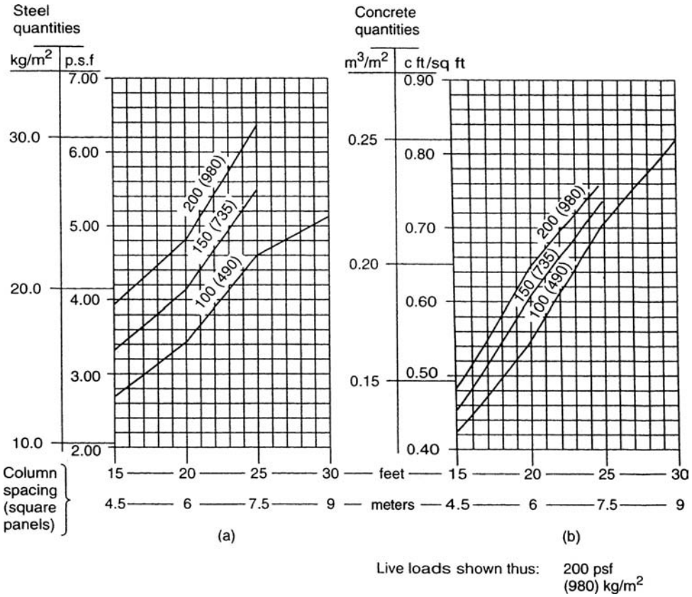
Figure 7.22. Two-way slab, unit quantities: (a) reinforcement; (b) concrete.
