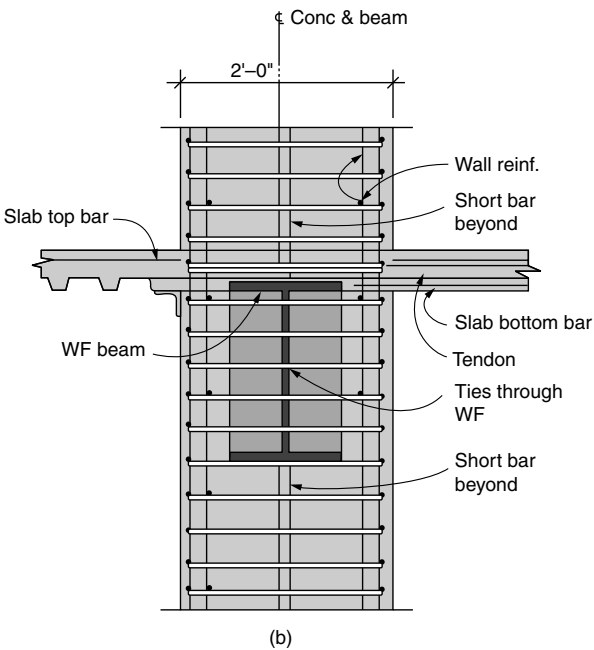
Figure 5.42. Renaissance project: (a) section through link beam at door opening; (b) coupling beam embedded in shear walls.
