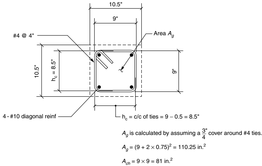
Figure 4.48. Parameters for calculating diagonal beam reinforcement.
