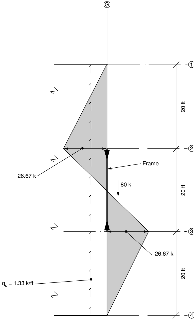
Figure 7.49b. Collector design forces.
