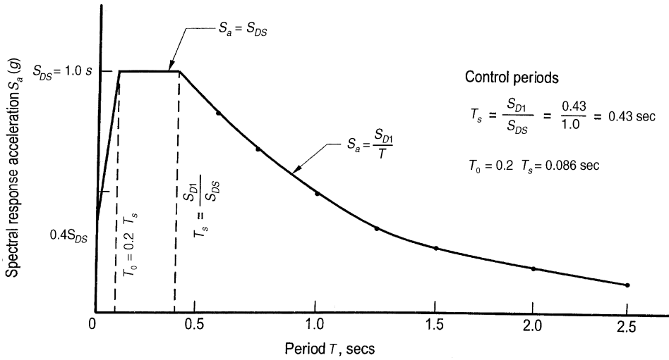
Figure 2.45c. General design response spectra; design example.
