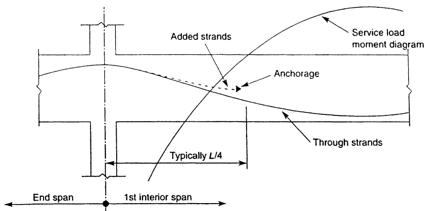
Figure 7.46. Anchorage of added tendons.
