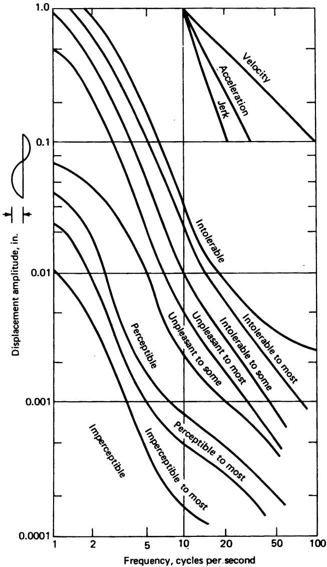
Figure 8.33a. Response to sustained harmonic vibration.
