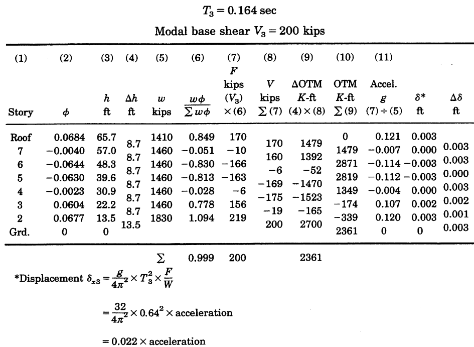
Figure 2.60. Seven-story building; third-mode forces and displacements.
