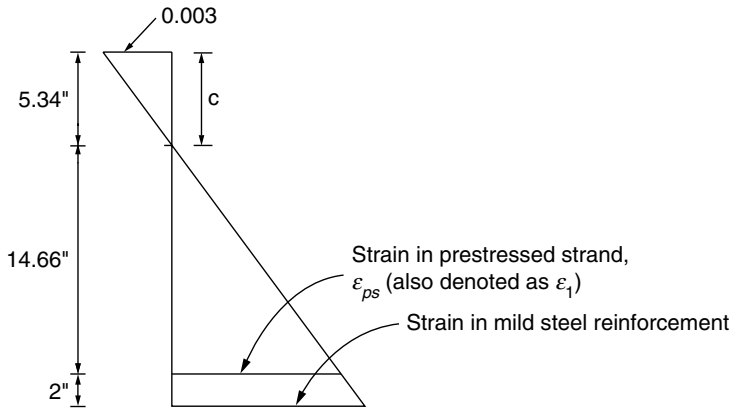
Figure 7.48c. Example 1: strain diagram, second trial.
