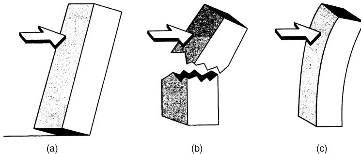
Figure 8.3. Bending resistance of building: (a) building must not overturn; (b) columns must not fail in tension or compression; (c) bending deflection must not be excessive.
