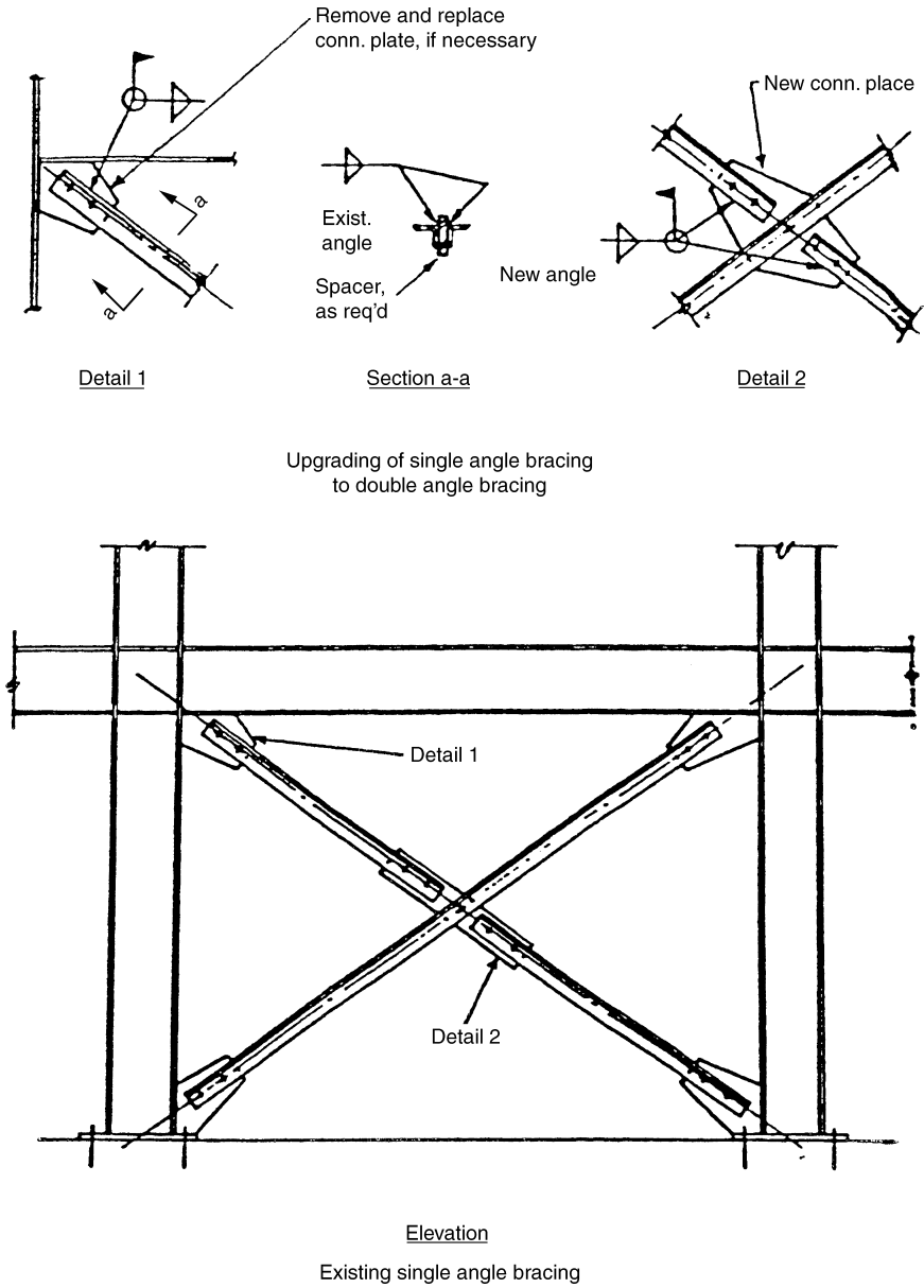
Figure 6.21. Strengthening of existing bracing.
