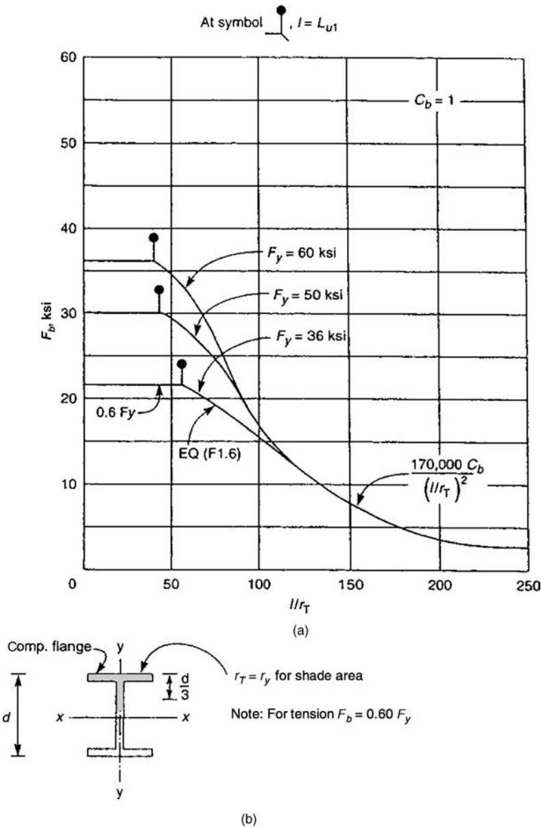
Figure 7.3. (a) Values of F_b for compact and noncompact I-sections: F_b versus l/r_T ; F_b controlled by warping torsion; (b) beam section showing area for the calculation of r_T ; (c) values of F_b for compact and noncompact I-sections: F_b controlled by St. Venant's torsion.
