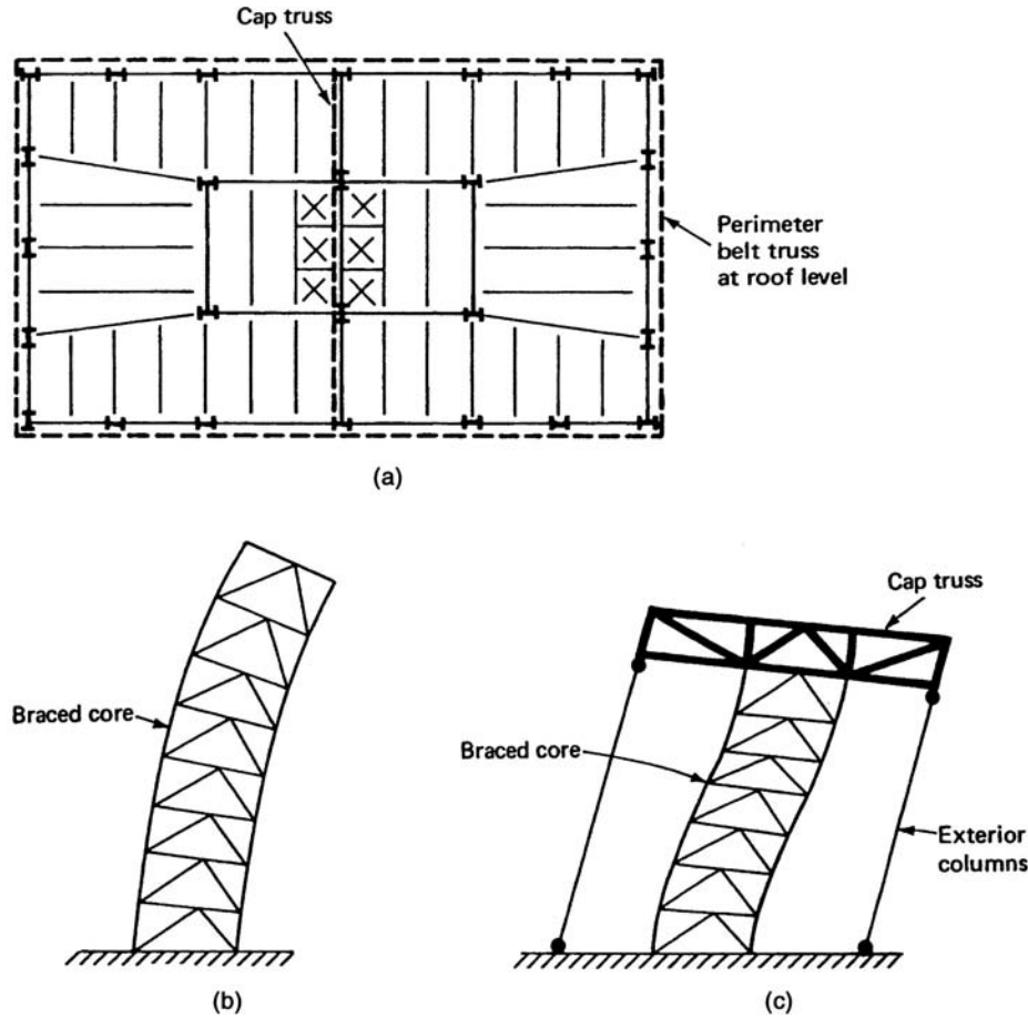
Figure 3.18. (a) Building plan with cap truss; (b) cantilever bending of core; (c) tie-down action of cap truss.
