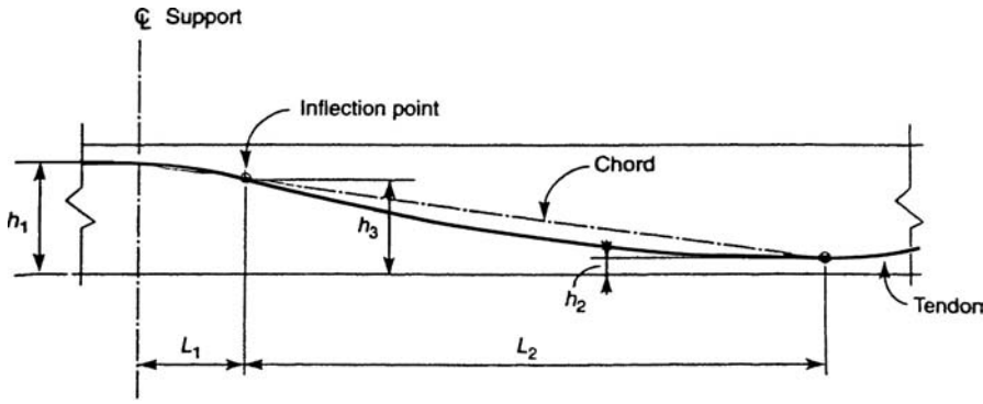
Figure 7.41. Dimensions for determining tendon drape.
