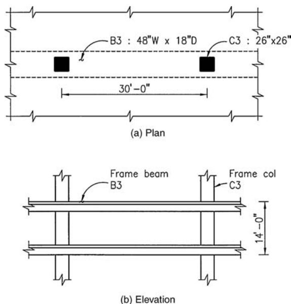
Figure 4.32. Frame beam and column example; ordinary moment frame: (a) plan; (b) elevation.
