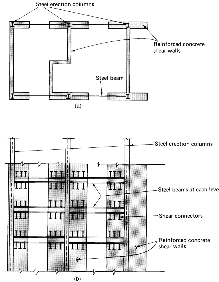
Figure 5.6. Composite shear wall with steel beams: (a) plan; (b) elevation.
