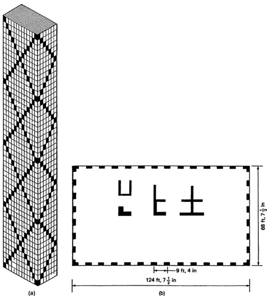
Figure 4.8. Exterior braced tube: (a) schematic elevation; (b) plan.
