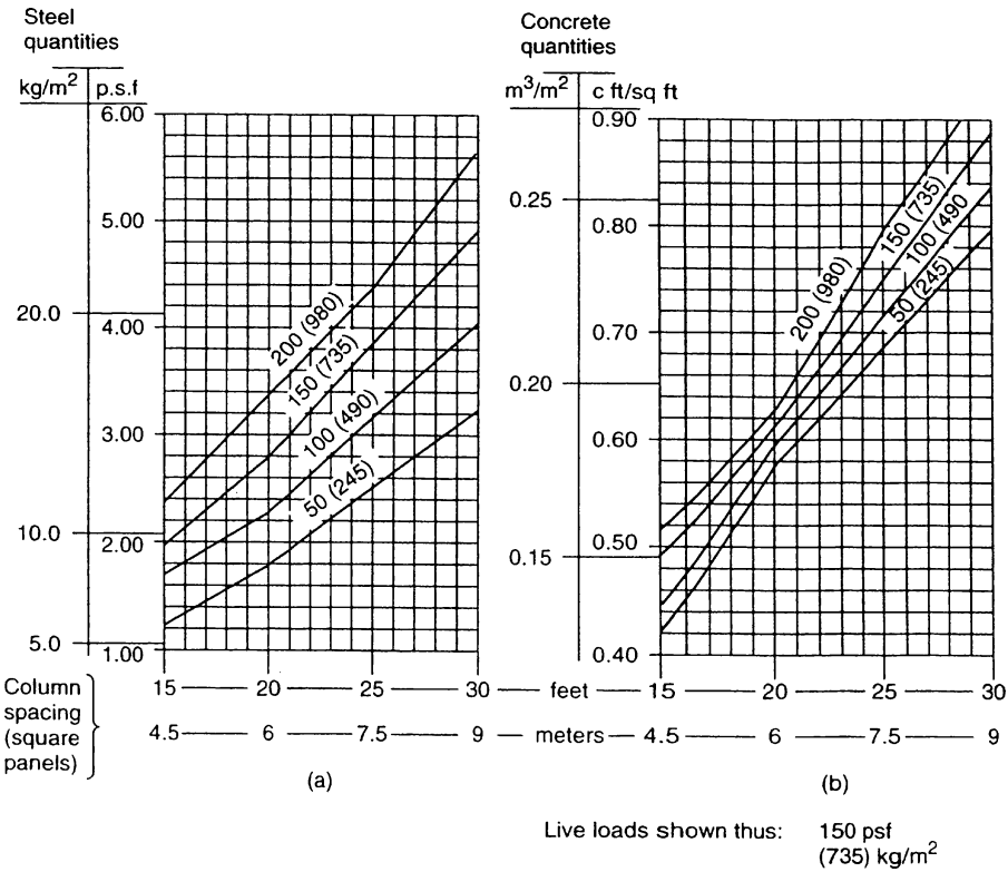
Figure 7.25. Flat slab, unit quantities: (a) reinforcement; (b) concrete.
