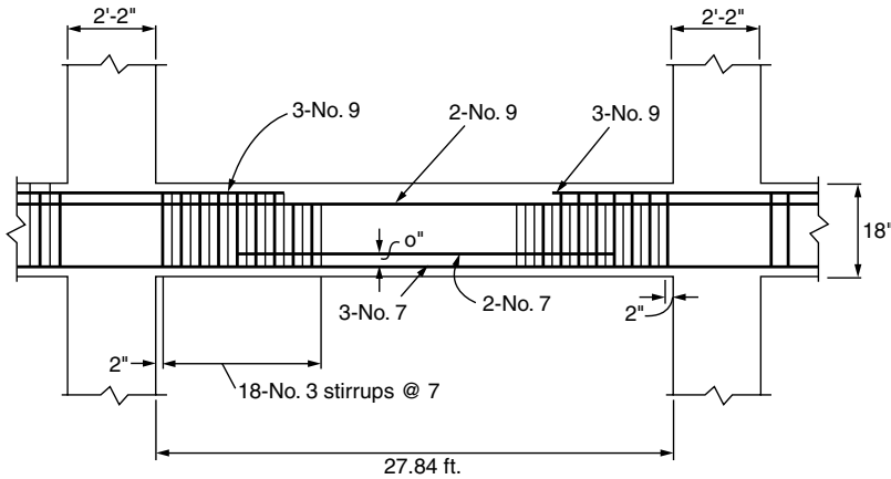
Figure 4.33. Design example, frame beam; ordinary moment frame. Although by calculations no shear reinforcement is required in the midsection of the beam, it is good practice to provide #3 four-legged stirrups at 15 in. spacing.
