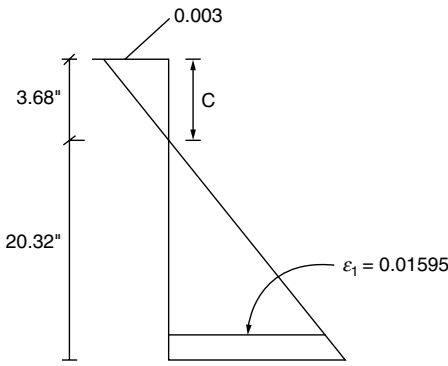
Figure 7.48h. Example 3: strain diagram; first trial.
