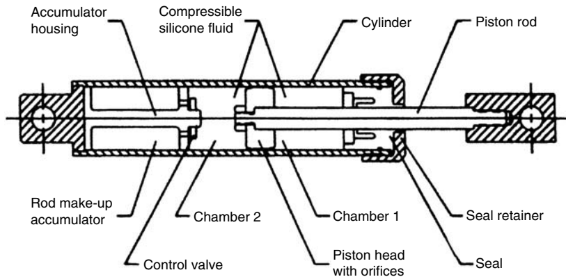
Figure 8.35b. Viscous fluid damper, consisting of a piston in a damping housing filled with a compound of silicone or similar type of oil. The piston contains small orifices through which the fluid passes from one side of the piston to the other. The damper thus dissipates energy through the movement of the piston in a highly viscous fluid.
