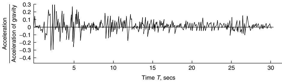
Figure 2.18. Recorded ground acceleration: El Centro earthquake.
