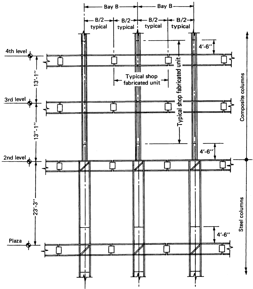
Figure 5.28. Typical frame fabrication unit.
