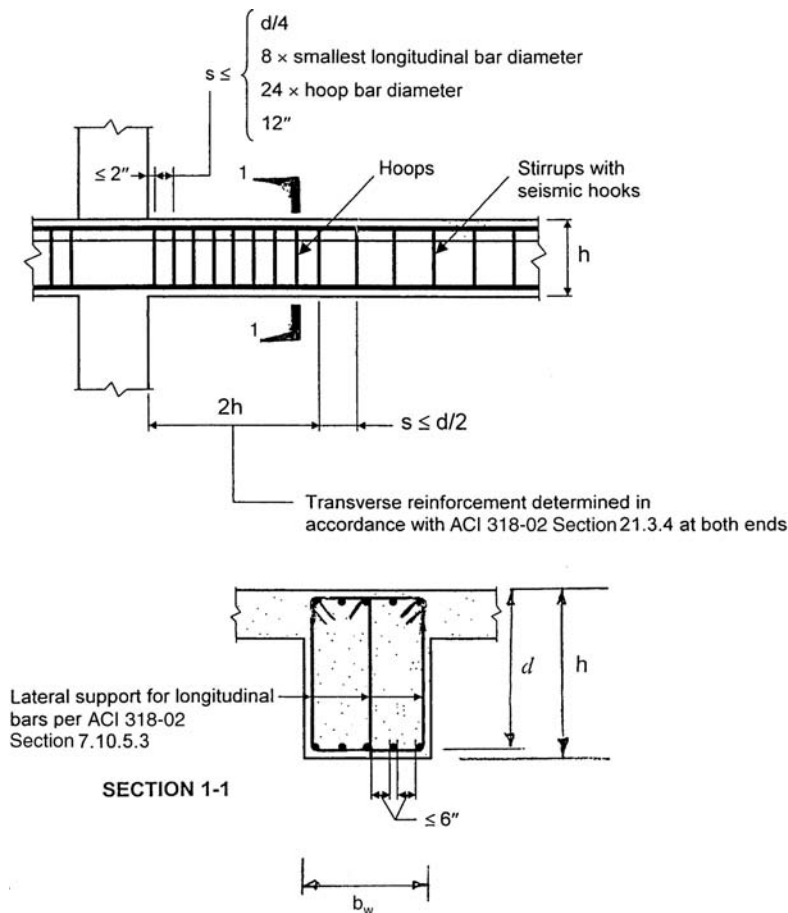
Figure 4.27. Frame beam; transverse reinforcement requirements, special moment frame.
