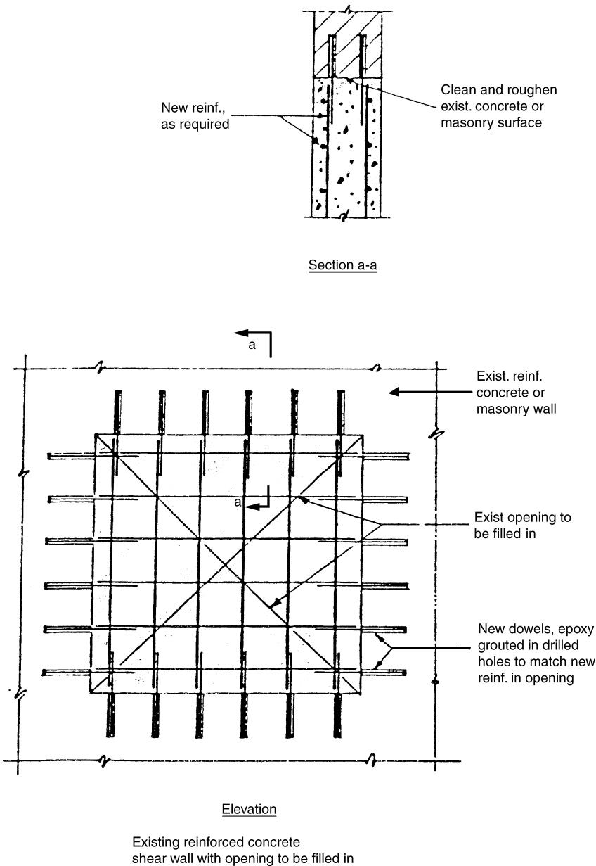
Figure 6.17. Strengthening of existing reinforced concrete walls by filling in of openings.
