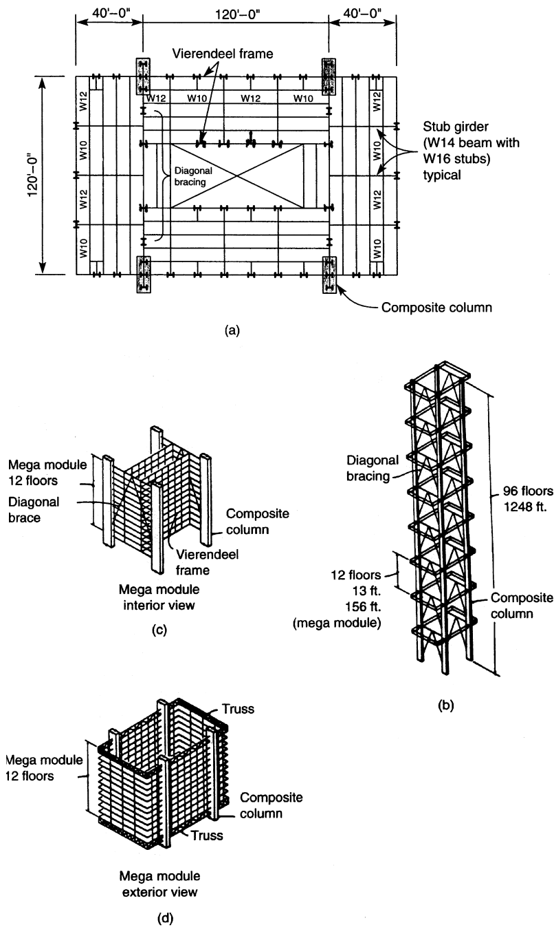
Figure 5.30. Structural concept for a super-tall building: (a) plan; (b) schematic elevation; (c) interior view of mega module; (d) exterior view of mega module.
