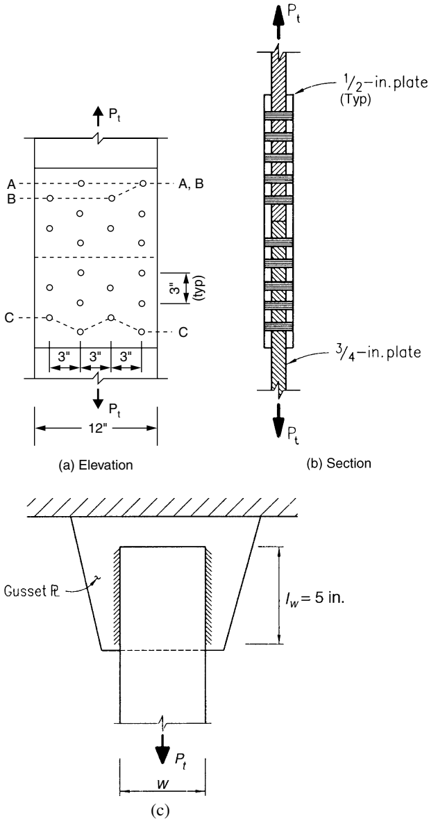
Figure 7.1. Bolted plate in tension: (a) elevation; (b) section; (c) welded plate in tension; design example.
