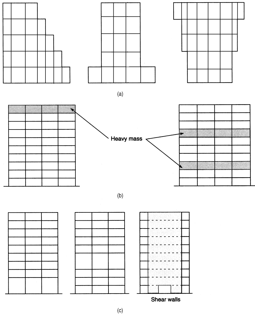
Figure 2.5. Elevation irregularities: (a) abrupt change in geometry; (b) large difference in floor masses; (c) large difference in story stiffnesses.
