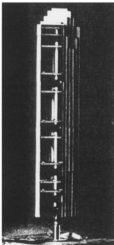
Figure 1.24. Cutaway view of an aeroelastic model of a tall building. (Photo courtesy of Dr. Peter Irwin, Rowan, Williams, Davis & Irwin, Inc.)
