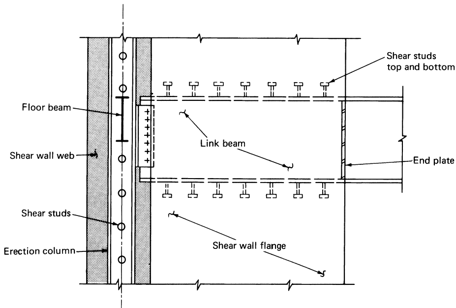
Figure 5.25. Arrangement of link beam in shear wall.
