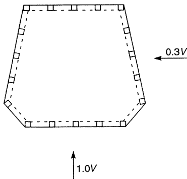
Figure 2.35. Irregularity due to nonparallel system. A nonparallel system irregularity exists when a lateral system is not parallel to or symmetric about the building's orthogonal axes.
