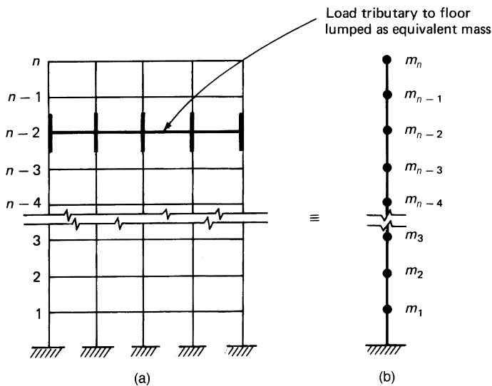
Figure 2.68. Multidegree-of-freedom system: (a) multistory analytical model with lumped masses.
