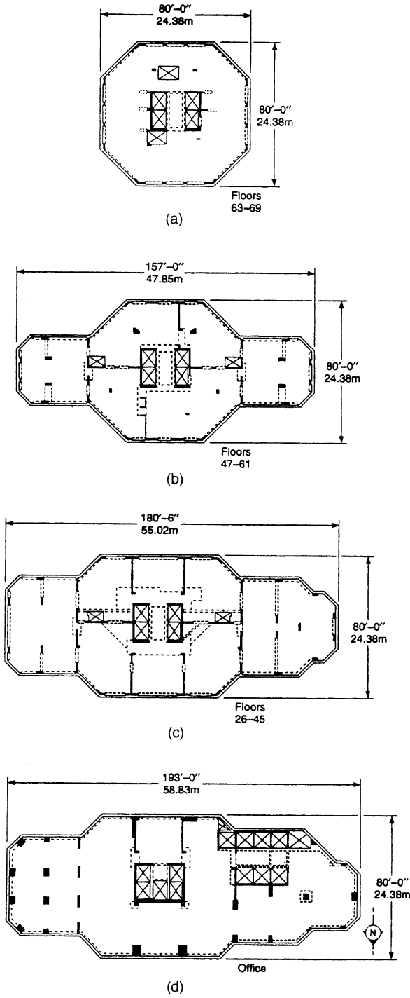
Figure 8.18. City Spire, New York; floor plans.
