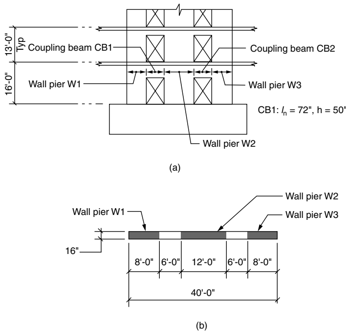
Figure 4.46. Coupled shear walls: (a) partial elevation; (b) plan.
