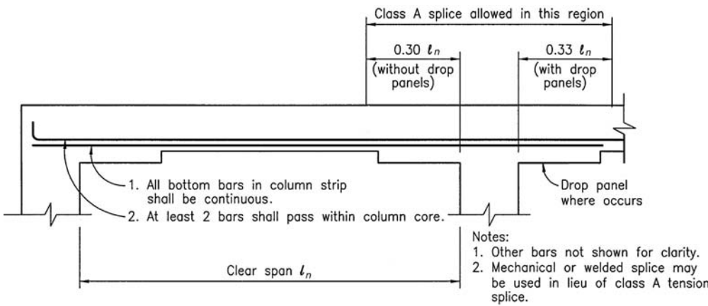
Figure 4.16. Structural integrity reinforcement in flat slabs without beams.
