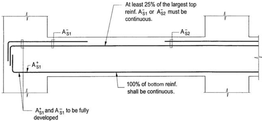
Figure 4.24. Seismic detailing requirements for two-way slabs in areas of moderate seismic risk; column strip.
