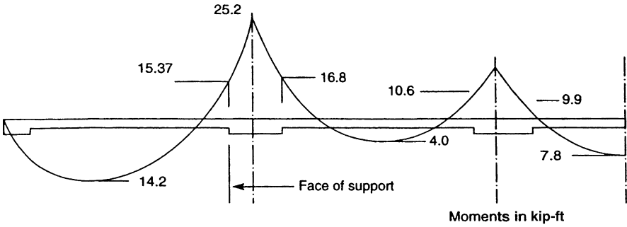
Figure 7.39. Example 1: one-way post-tensioned slab service load, ( D + L ), moment diagram.
