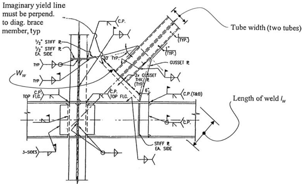
Figure 3.47. Typical bracing-to-column connection, SCBF.
