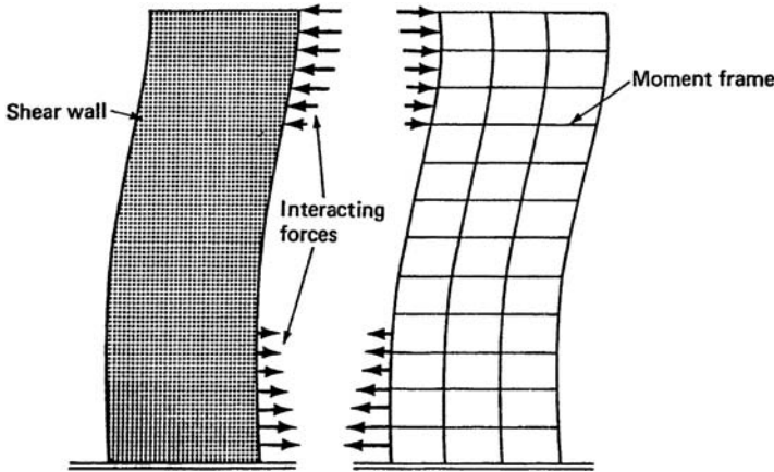
Figure 4.7. Shear wall–frame interaction.
