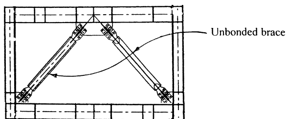
Figure 8.36c. Buckling-restrained brace frame, BRBF, with chevron braces. Since the braces yield both in tension and compression, a chevron configuration does not penalize design of the beam connected to the braces.
