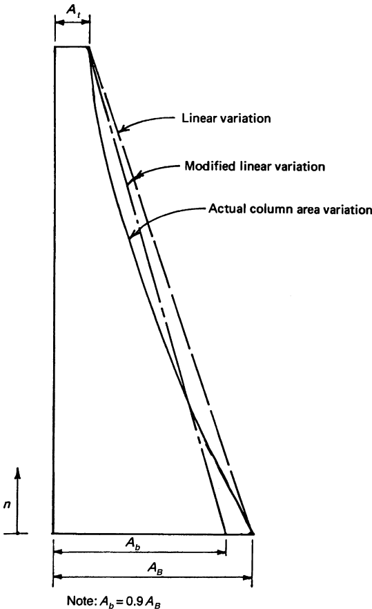
Figure 8.32e. Idealized column cross-sectional areas.
