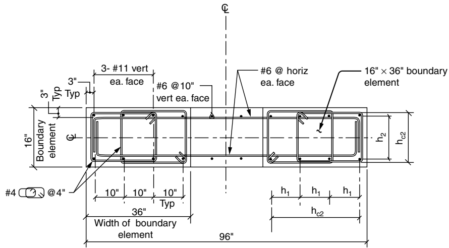
Figure 4.52. Schematic reinforcement layout for wall pier, example 2.
