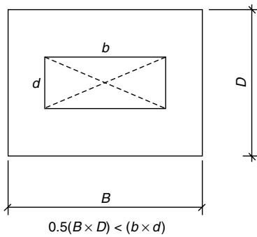
Figure 2.33. Irregularity due to diaphragm discontinuity. This irregularity exists if: 1) the area b \times d of the opening is more than 50% of the area B \times D of the diaphragm; or 2) the change in diaphragm stiffness is more than 50% from one story to the next.
