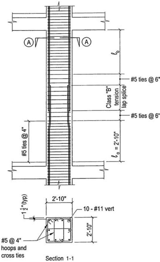
Figure 4.40. Design example, frame column; special moment frame.
