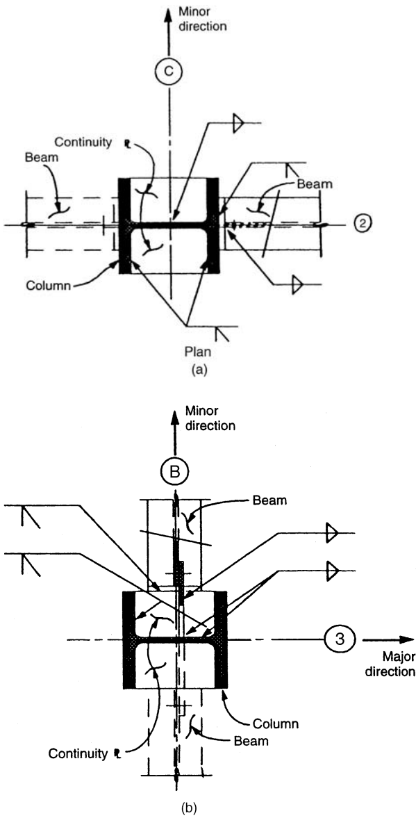
Figure 7.5. Beams framing into columns in one direction: (a) Beam framing into column flange; (b) beam framing into column web.
