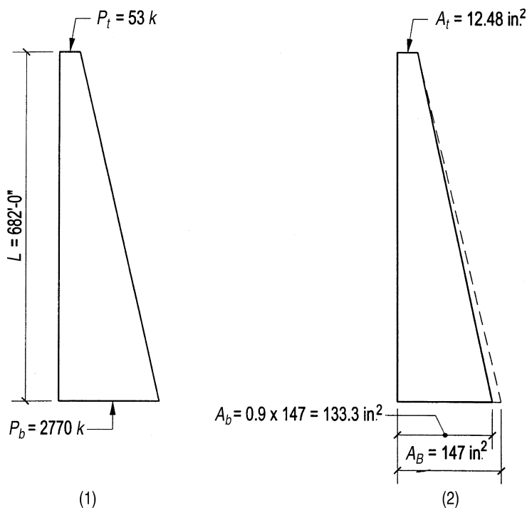
Figure 8.32g. Example 1, column-shortening calculations: (1) axial load variation; (2) actual and assumed variation in column cross-sectional areas.
