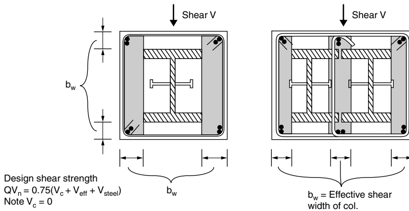
Figure 5.31. Encased composite column; design shear strength parameters.
