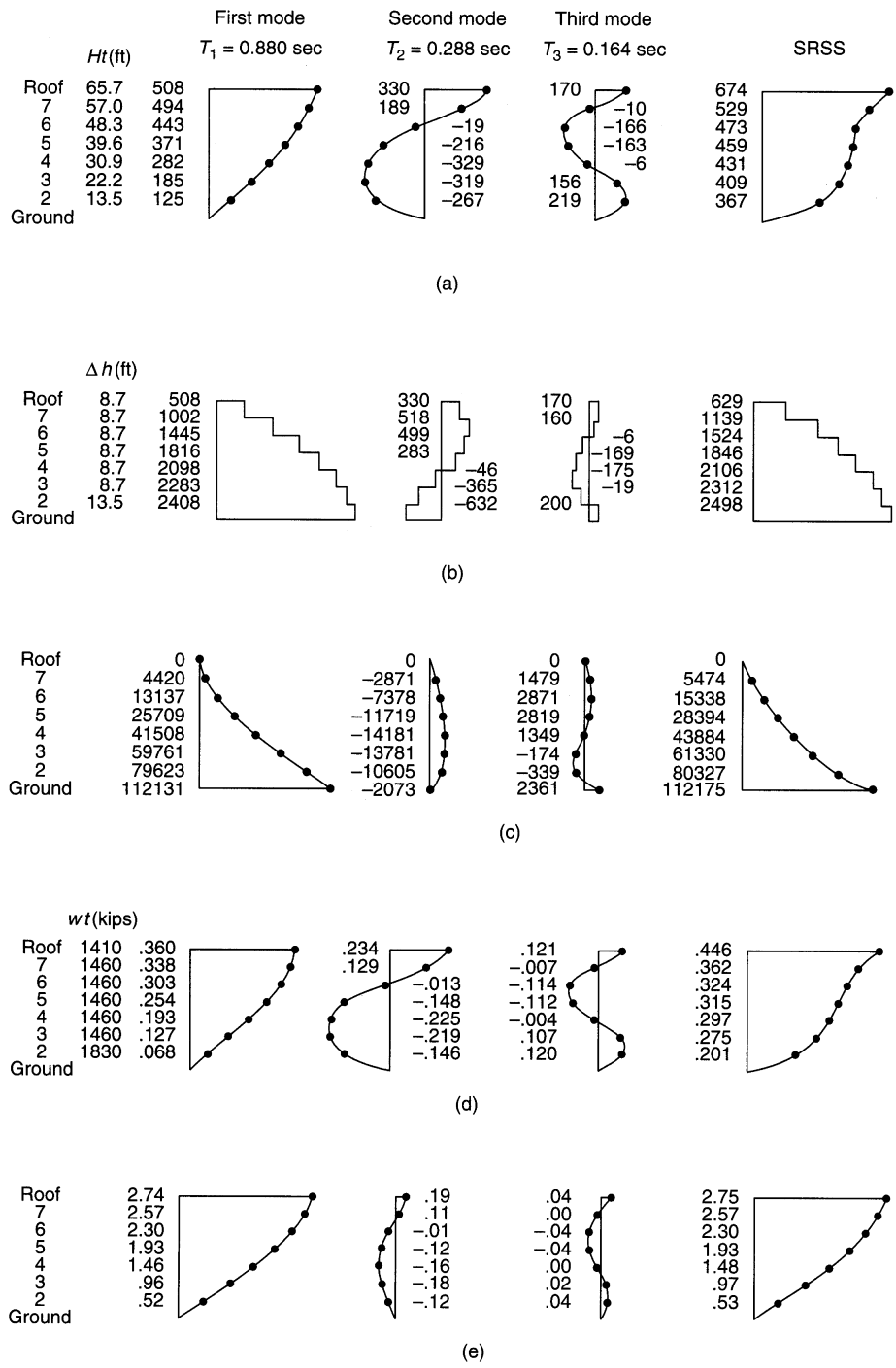
Figure 2.61. Seven-story building. Modal analysis summary: (a) modal story forces (kips); (b) modal story shears (kips); (c) modal story overturning moments (kip-ft); (d) modal story acceleration (g's); (e) modal lateral displacements (in.).
