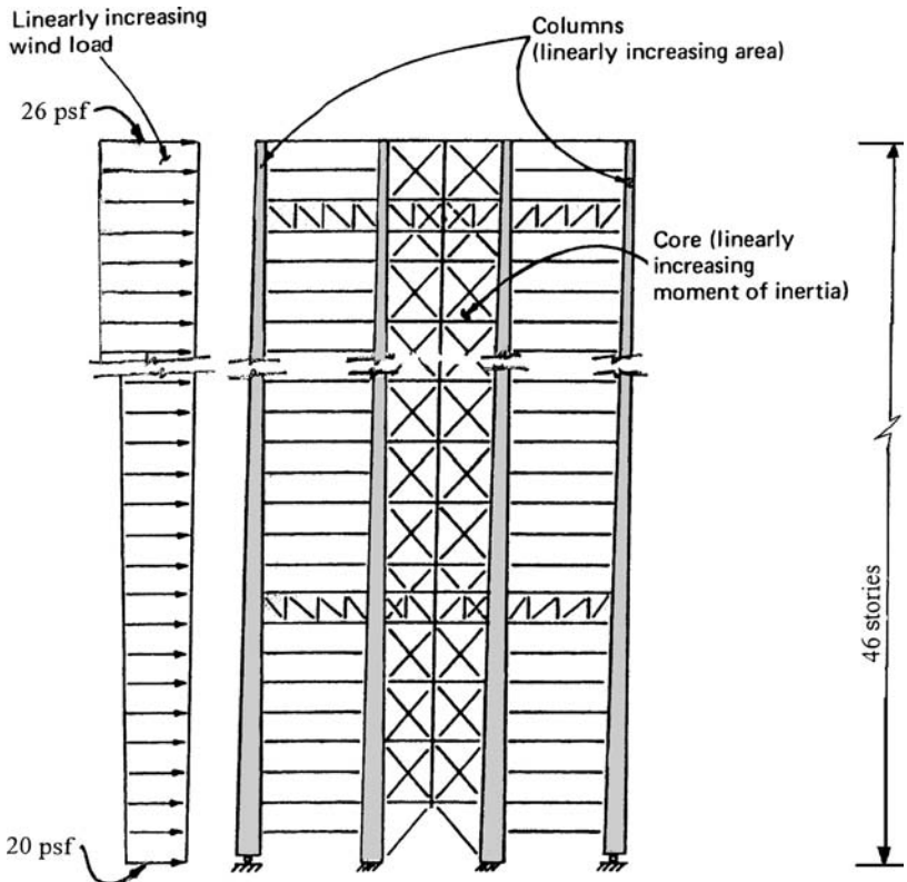
Figure 3.28. Conceptual analytical model and loading diagram for a building with two outriggers and belt trusses.
