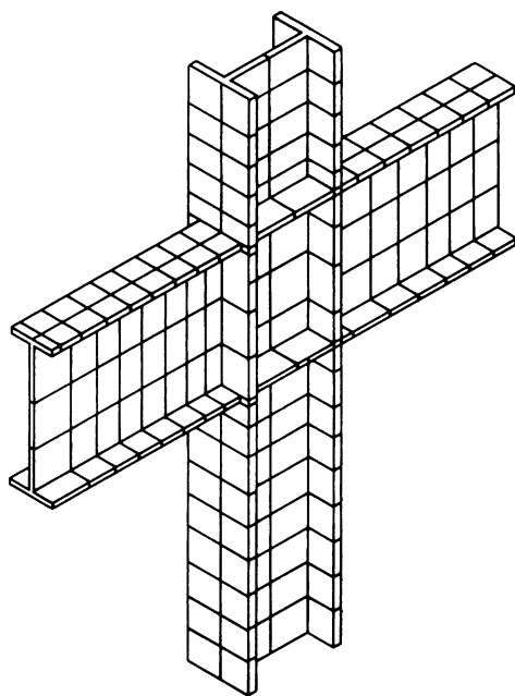
Figure 8.31d. Finite element idealization of typical frame unit.
