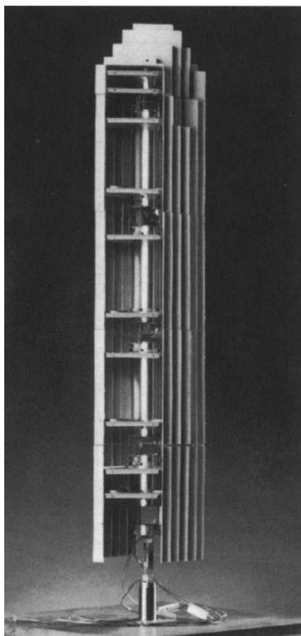
Figure 1.27. High-frequency force balance model of a medium-rise building. (Photo courtesy of Dr. Peter Irwin, Rowan, Williams, Davis & Irwin, Inc.)
