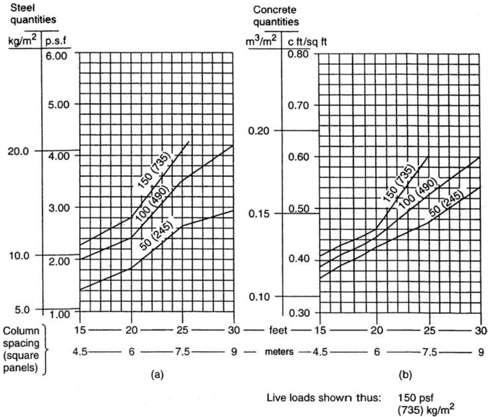
Figure 7.21. One-way pan joist, unit quantities: (a) reinforcement; (b) concrete.
