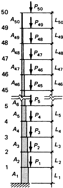
Figure 8.32a. Axial shortening computations for a practical column.
