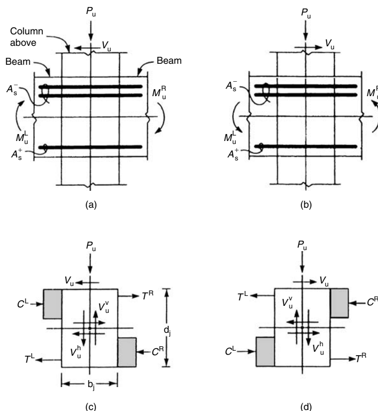
Figure 4.40b. Beam-column joint analysis: (a) forces and moments, case 1; (b) forces and moments, case 2; (c) resolved forces, case 1; (d) resolved forces, case 2.
