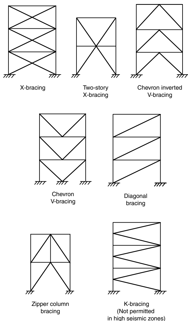
Figure 3.40a. Braced frame configurations.
