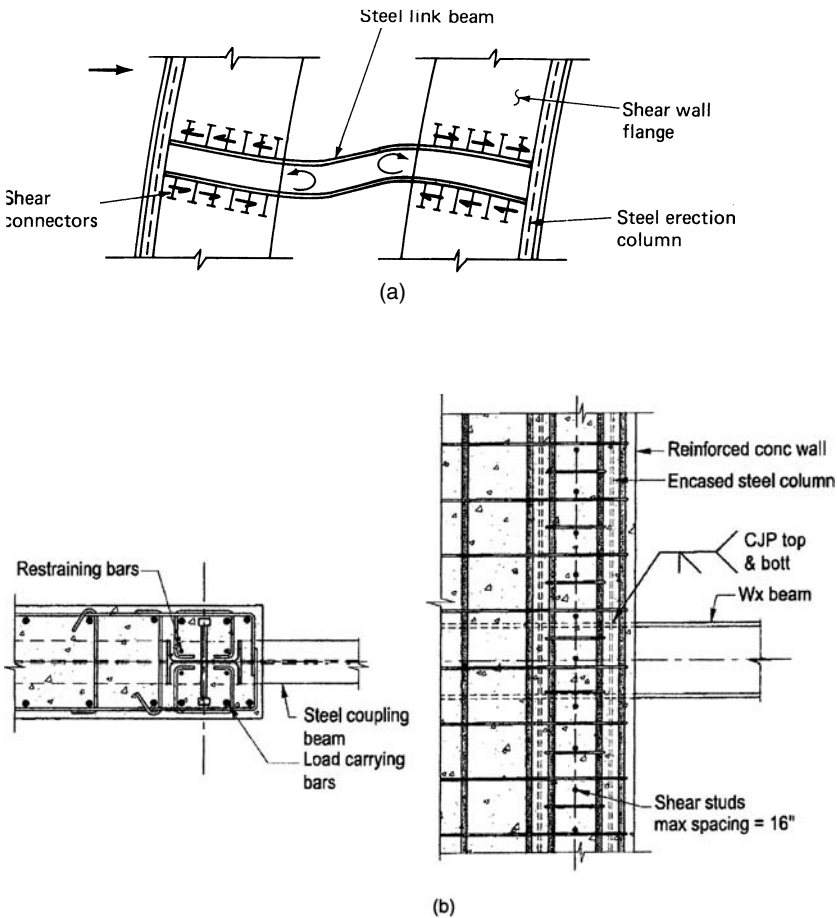
Figure 5.7. Moment transfer between steel beam and concrete wall.
