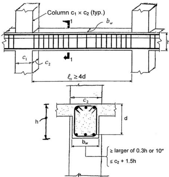
Figure 4.26. Frame beam; general requirements, special moment frame.
