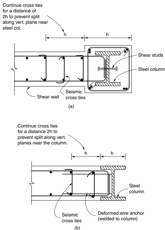
Figure 5.39. Composite shear walls with steel boundary elements.
