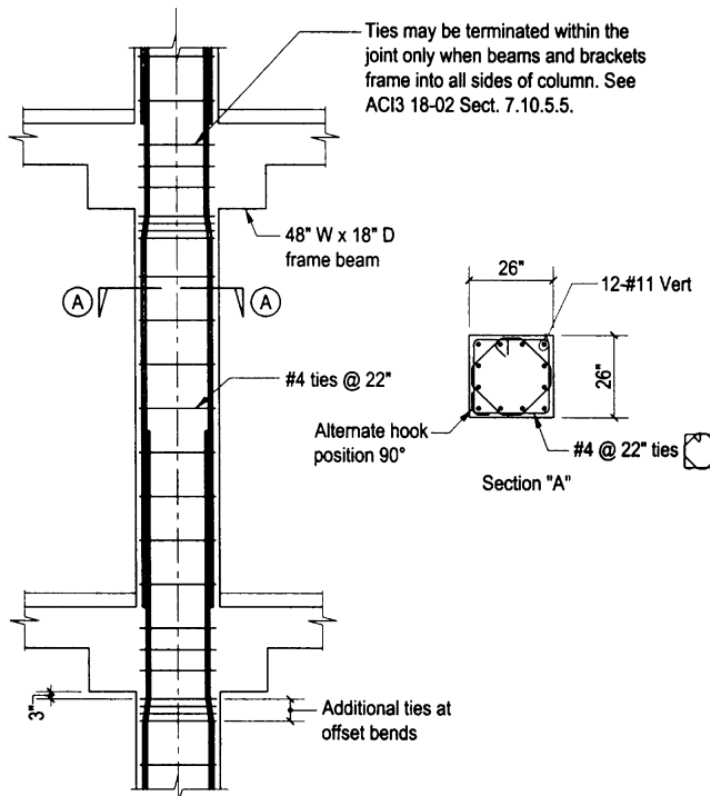
Figure 4.34. Design example, frame column; ordinary moment frame.
