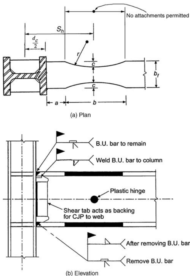
Figure 3.57. Prequalified reduced beam section (RBS) connection.
