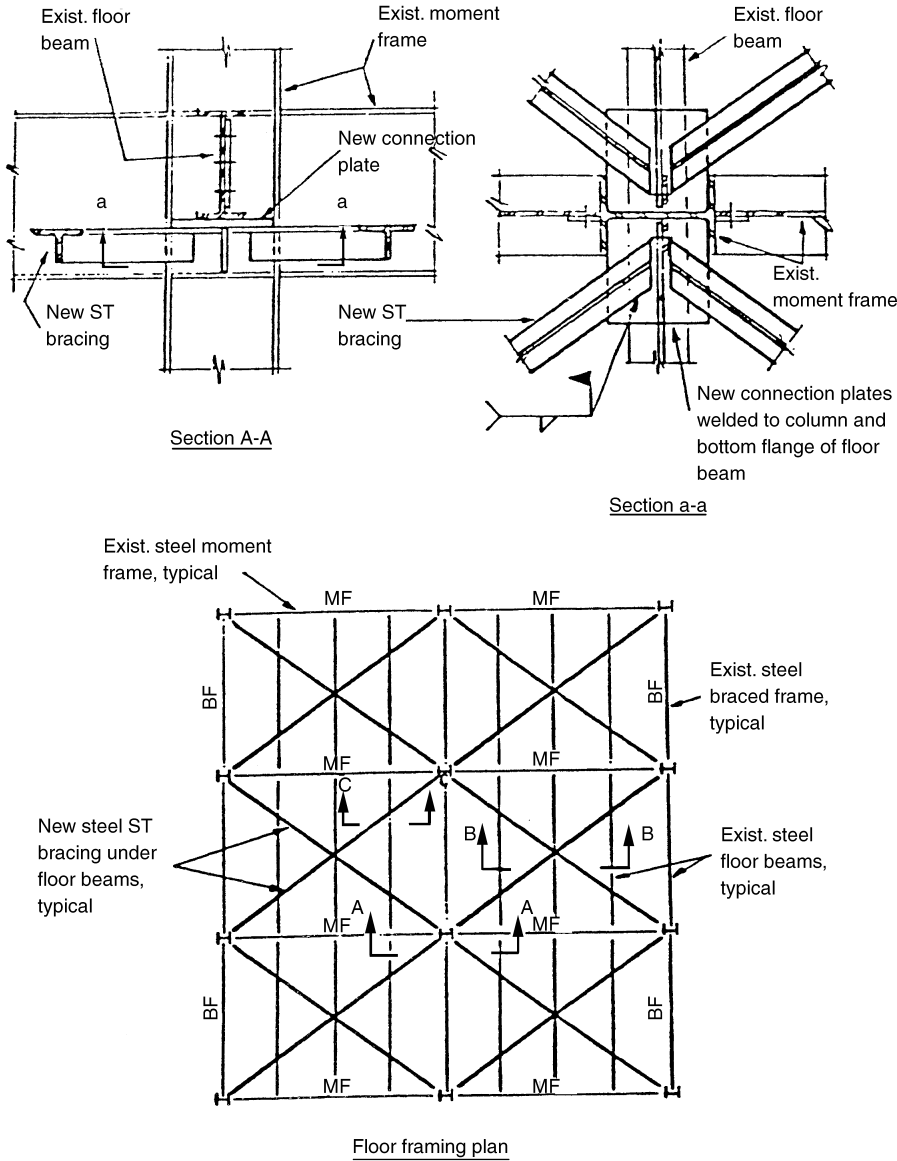
Figure 6.8. Strengthening of an existing steel frame building with horizontal bracing.
