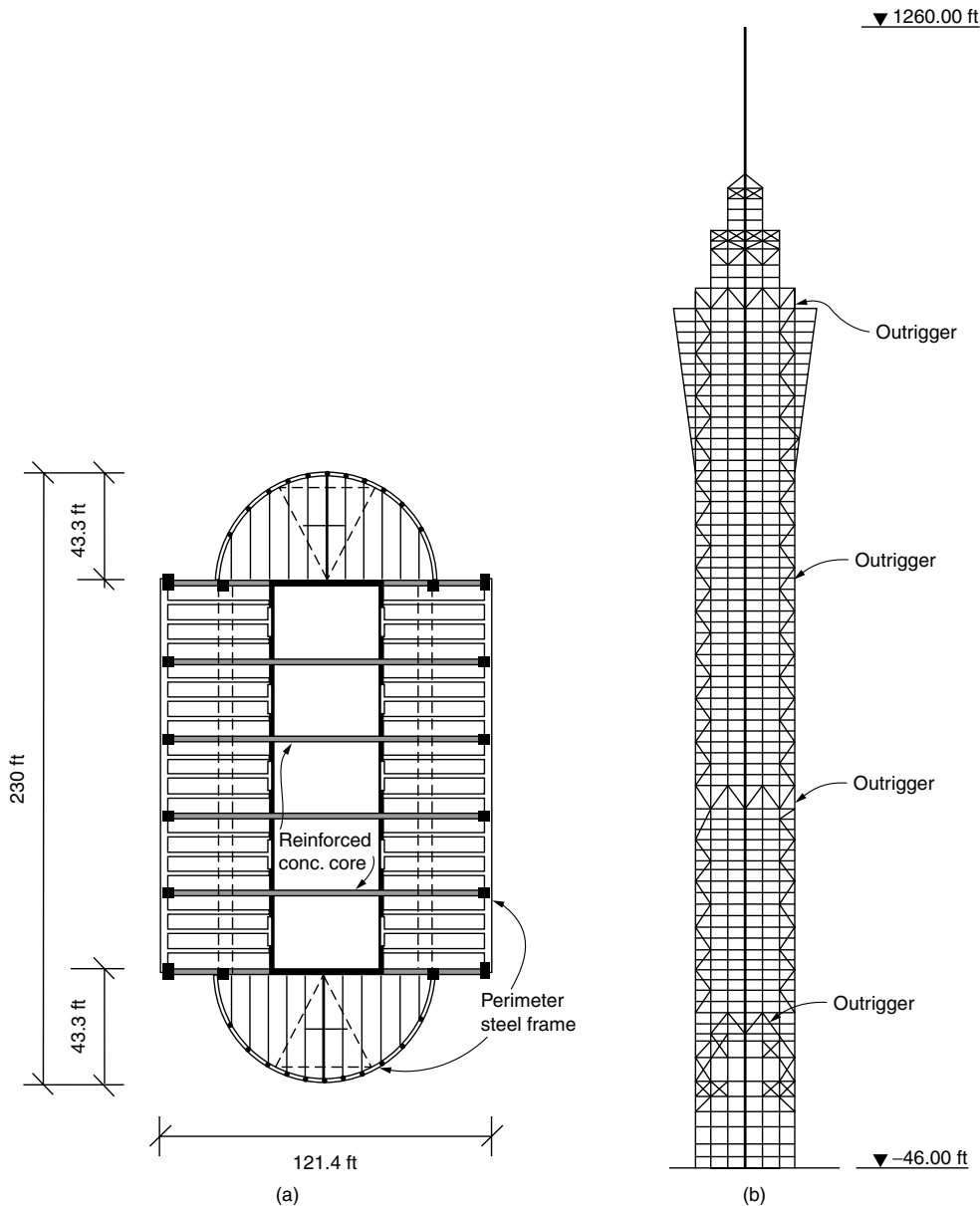
Figure 5.45. Di Wang Building, Shenzhen City, China: (a) schematic plan; (b) schematic elevation; (c) photograph of rendering. (Photograph and sketches courtesy of Chaoying Luo, P.E., John A. Martin & Associates, Structural Engineers, Los Angeles, CA.)
