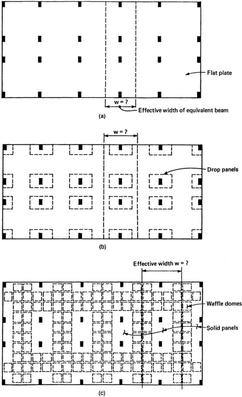
Figure 4.2. Lateral systems using slab and columns: (a) flat plate; (b) flat slab with drop panels; (c) two-way waffle system.
