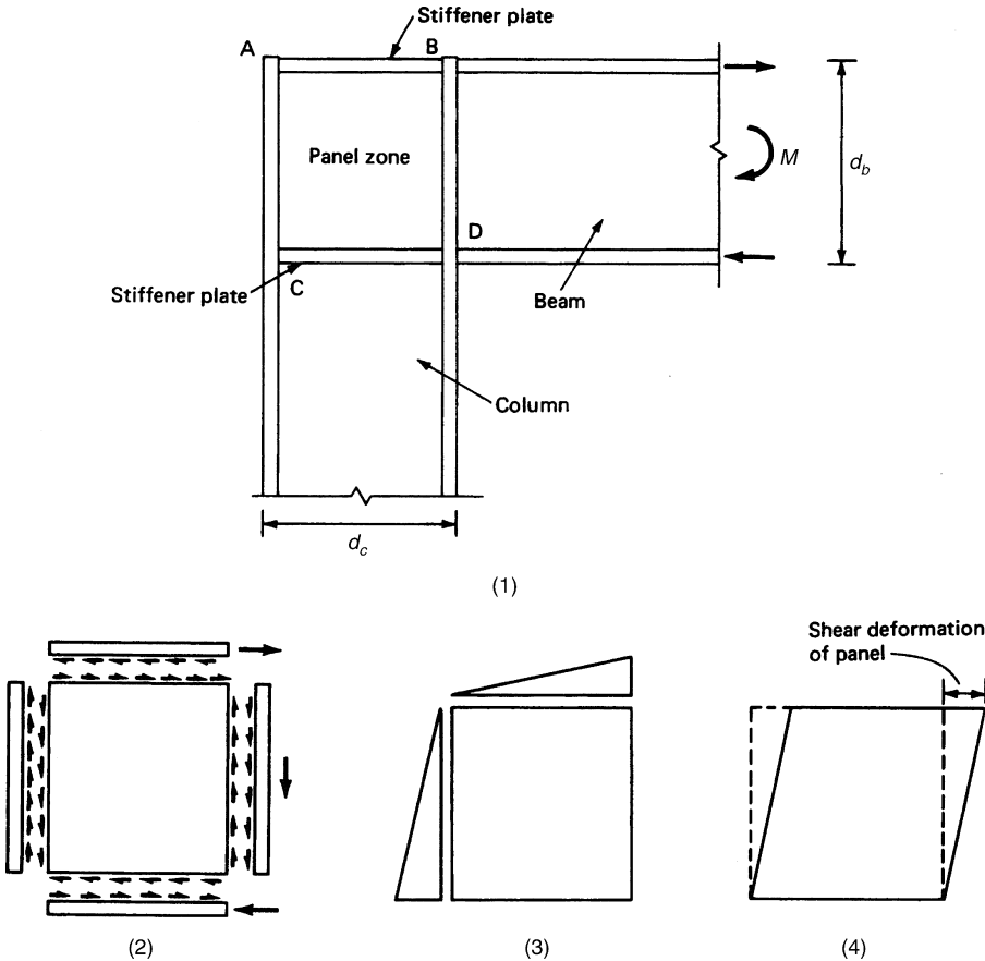
Figure 8.31b. Panel zone behavior: (1) corner panel; (2) schematic representation of shear forces in panel zone; (3) linear distribution of tensile stresses; (4) shear deformation of panel zone.
