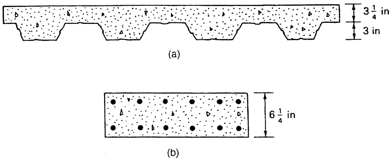
Figure 7.64. Equivalent slab section.
