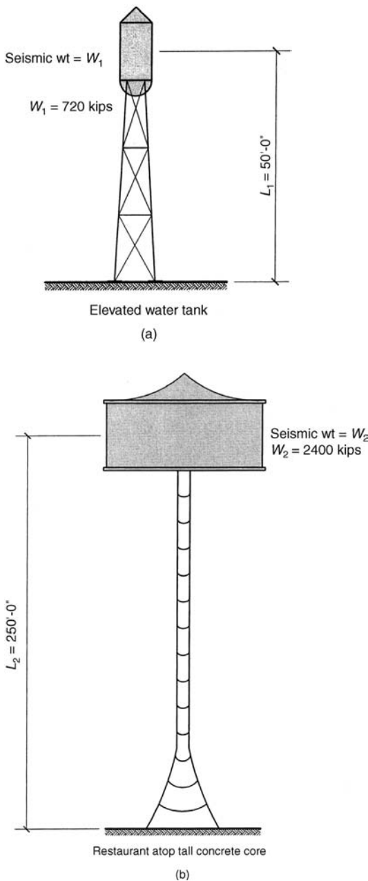
Figure 2.17a. Examples of single-degree-of-freedom systems: (a) elevated water tank (b) restaurant atop tall concrete core. Note from Fig. 2.17, the acceleration = 26.25 \text{ ft/s}^2 for T = 0.5 \text{ s} and \beta = 0.05 (water tank) and the acceleration = 11.25 \text{ ft/s}^2 for T = 1.00 and \beta = 0.10 (restaurant).
