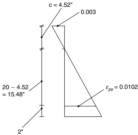
Figure 7.48e. Example 2: strain diagram, first trial.
