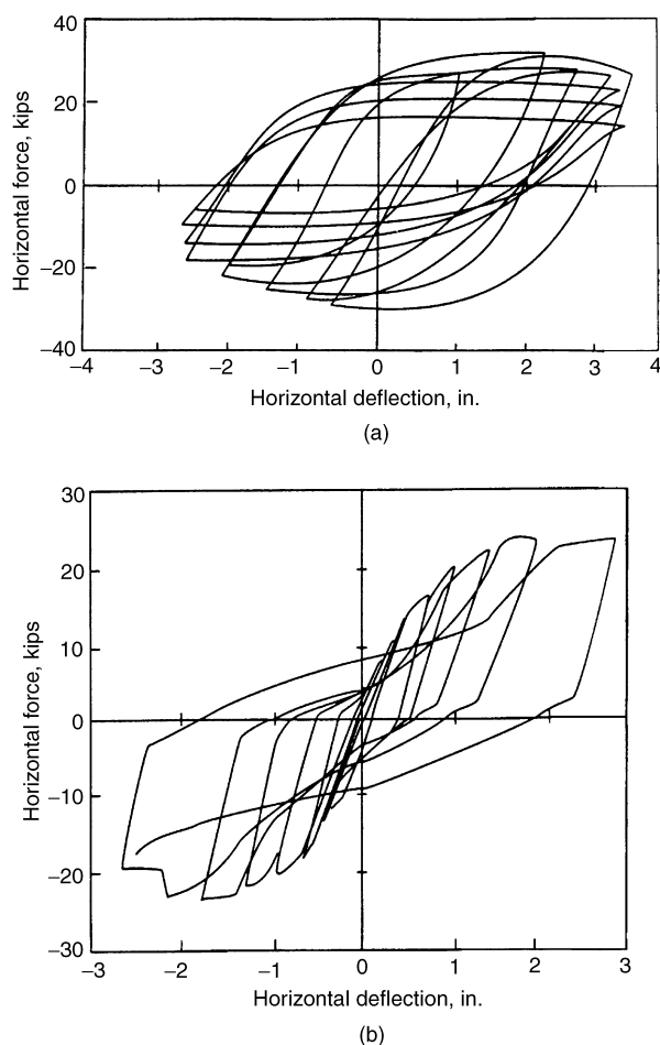
Figure 2.9. Hysteretic behavior: (a) curve representing large energy dissipation, (b) curve representing limited energy dissipation.
