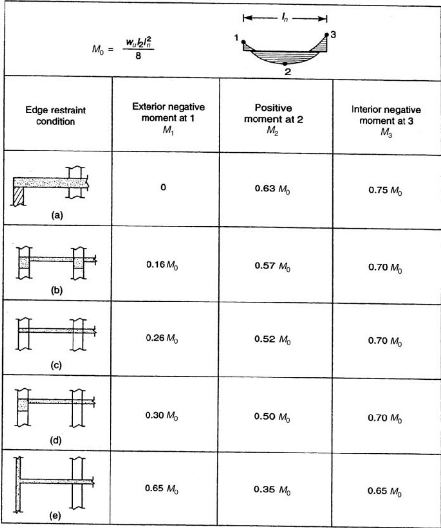
Figure 7.18. Assignment of moments to critical sections—exterior span (ACI 318-02).
