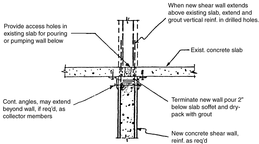
Figure 6.15. (Continued) Section 9-9 (when new wall extends above existing slab).
