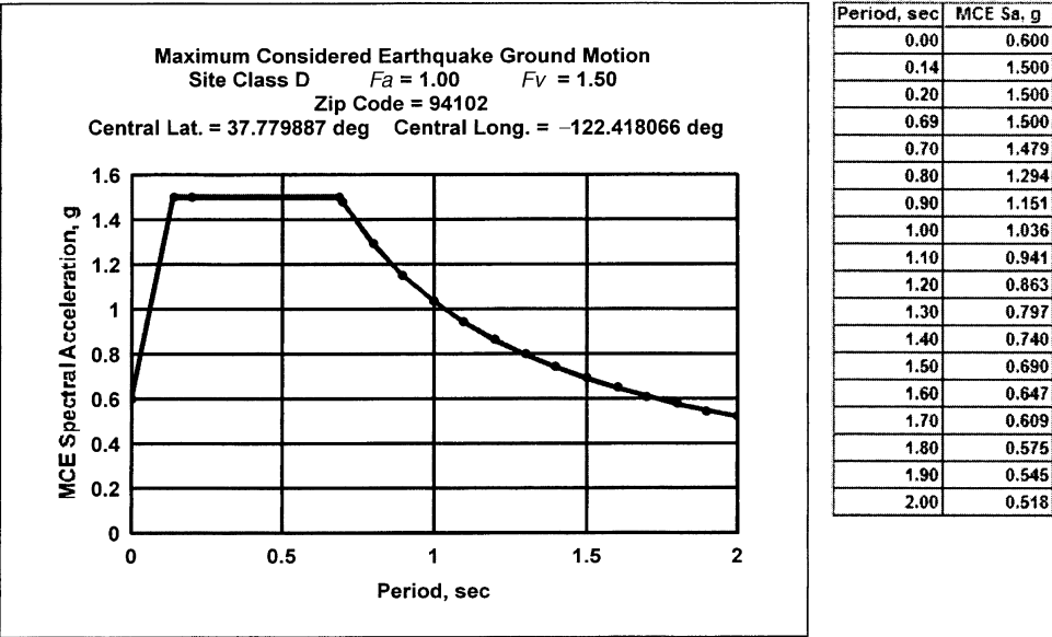
Figure 2.44. Maximum considered earthquake ground motions; 2% probability of exceedence in 50 years, corresponding to a return period of 2475 years, typically rounded to 2500 years.
