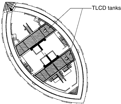
Figure 8.30e. Mechanical penthouse cross section of the Wall Center, a 48-story building in Vancouver, British Columbia. Two specially shaped tanks containing 50,000 gallons of water provide the mass for the building’s TLCD. Structural engineering by Glotman Simpson Consulting Engineers, Vancouver, British Columbia, Canada; TLCD by Rowan, Williams, Davies, & Irwin, Inc., and Motion Engineering, Inc., Guelph, Ontario, Canada.
