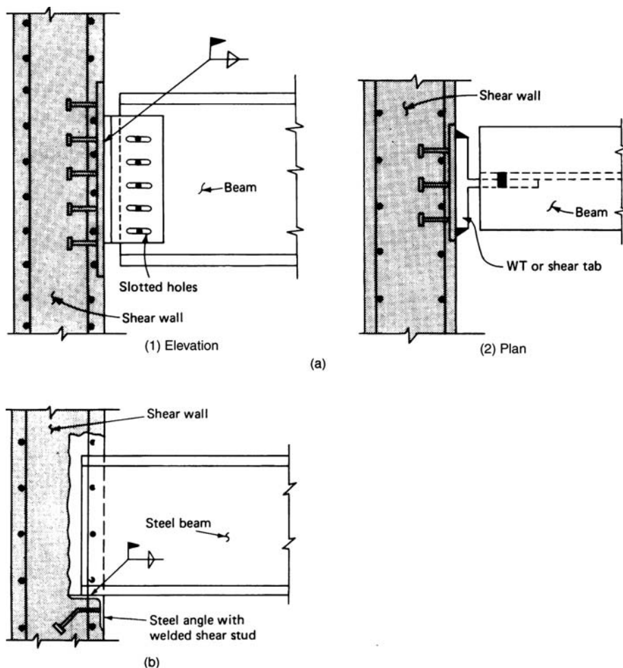
Figure 5.10. Beam-to-shear wall connection: (a) embedded plate detail; (b) pocket detail.
