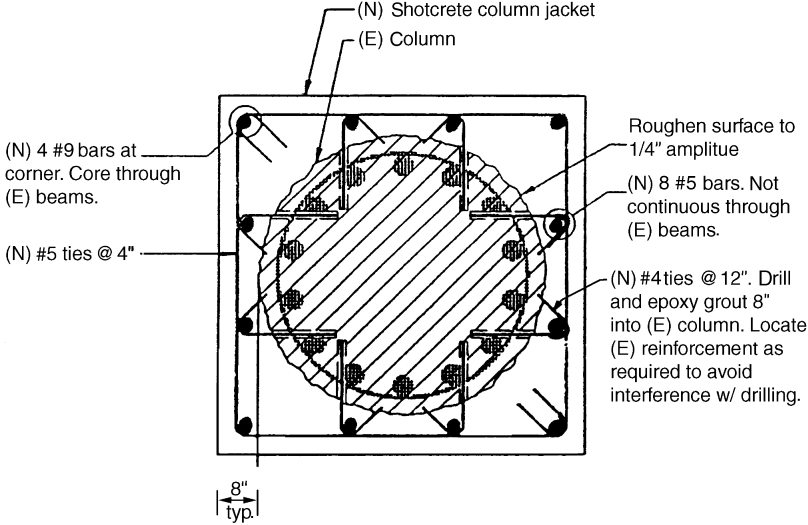
Figure 6.18. Jacketing of circular column.
