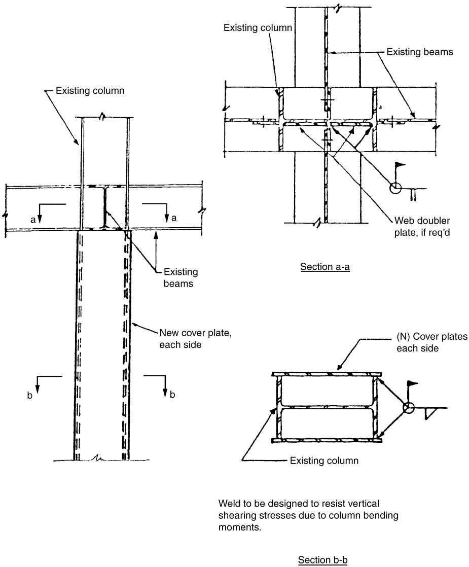
Figure 6.23. Strengthening of existing columns.
