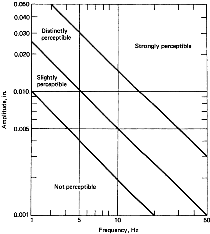
Figure 8.33b. Reiher-Meister vibration criteria.
