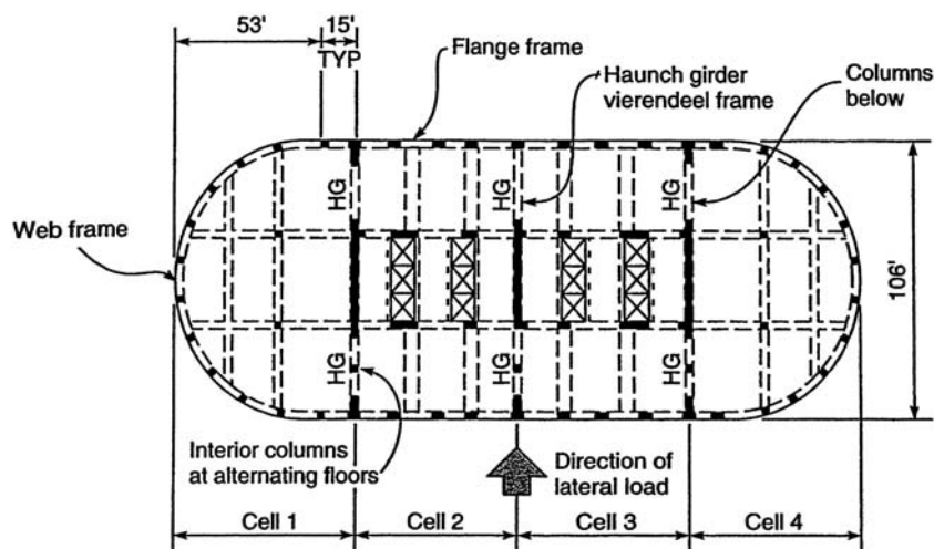
Figure 4.13. Cellular tube with interior vierendeel frames.
