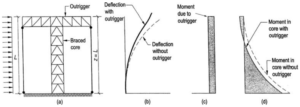
Figure 3.19. Outrigger at top, z = L .
