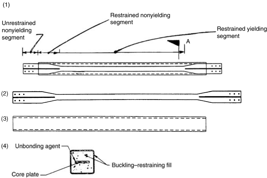
Figure 8.36b. Components of unbonded brace. (1) buckling restrained brace; (2) core; (3) sleeve; (4) section. The yielding of core plates in compression without buckling results in a stable hysteretic loop with excellent energy-dissipating characteristics.
