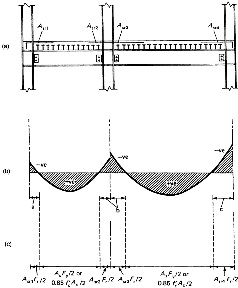
Figure 7.55. Continuous composite beam subjected to uniformly distributed load: (a) elevation; (b) moment diagram; (c) horizontal shear resisted by studs in the positive and negative moment regions.
