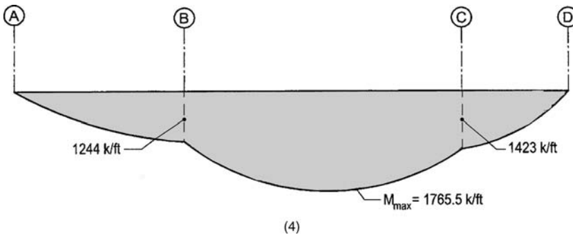
Figure 7.49a. (Continued.) Bending moment diagram.
