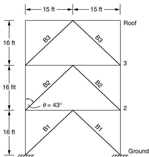
Figure 3.41. Special concentric brace frame (SCBF) example.
