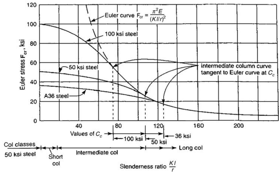
Figure 7.4. Euler stress, P_{cr}/A versus Kl/r .
