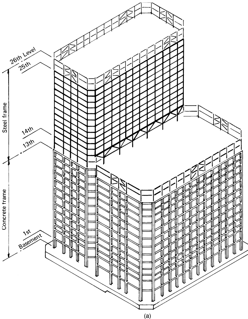
Figure 5.14. Vertically mixed system: (a) schematic perframing; (b) schematic bracing concept.
