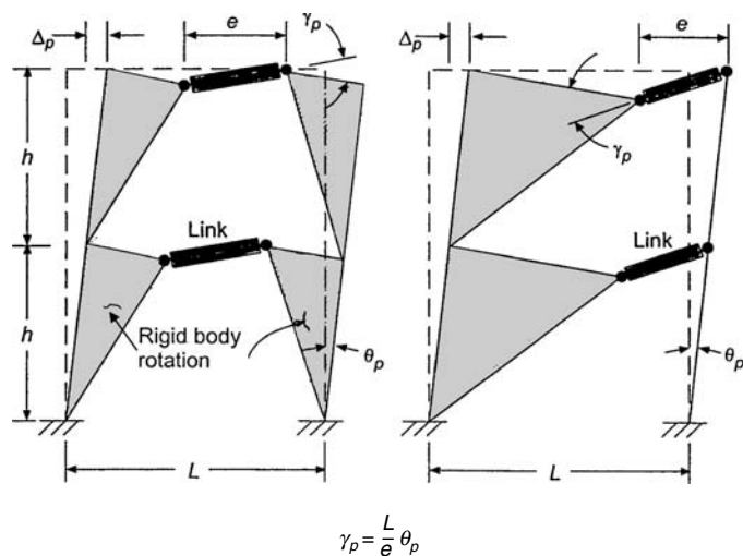
Figure 3.54. Link rotation angle \gamma_p . The link rotation angle \gamma_p is estimated by assuming the EBF bay rotates as a rigid body. By geometry, \gamma_p is related to plastic story drift angle \theta_p , which in turn is related to plastic story drift = \Delta_p/h . Conservatively, \Delta_p may be taken to equal design story drift. Refer to AISC 341-02, C15.2 for additional information.
