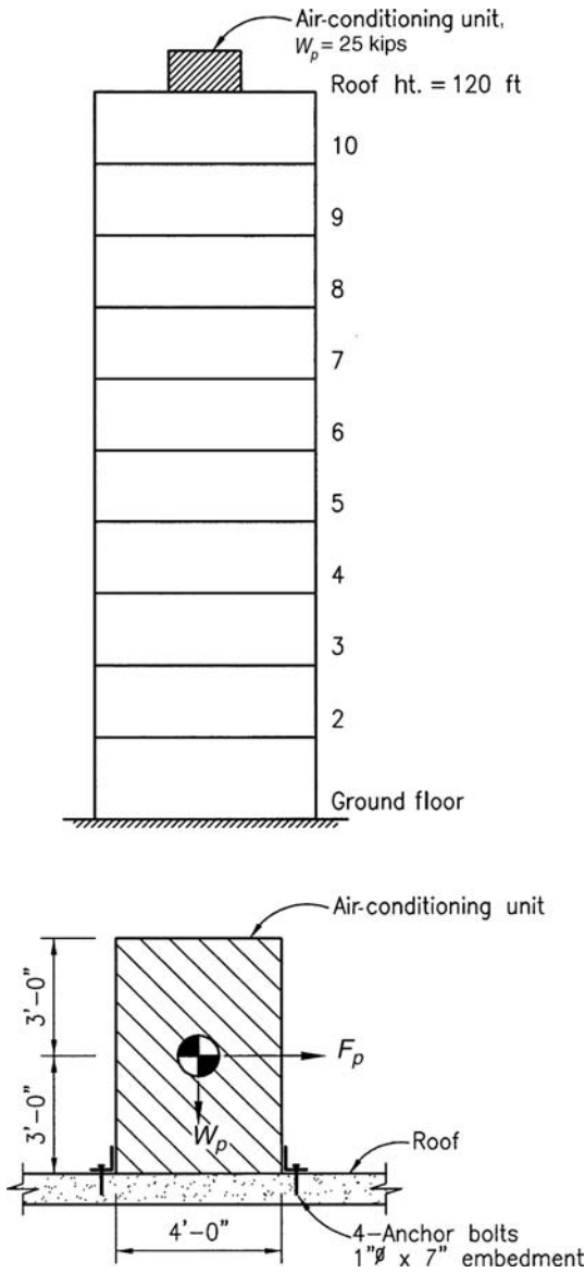
Figure 2.63. Equipment anchorage design; air-conditioning unit example.
