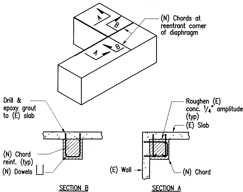
Figure 6.7. New chords at reentrant corners.
