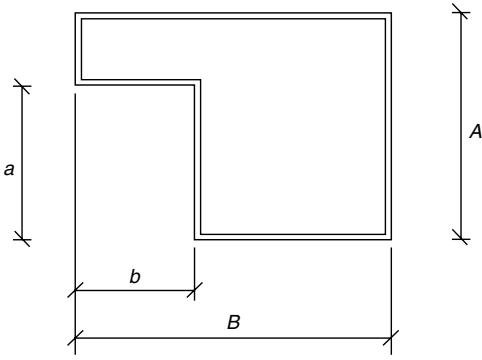
Figure 2.32. Irregularity due to reentrant corners. This irregularity exists when plan configuration of the building and its lateral system have projections greater than 15% of the plan dimension in the corresponding direction. b > 0.15B or a > 0.15A .
