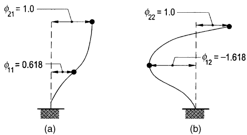
Figure 2.48. Vibration modes; two-story example: (a) first mode; (b) second mode.
