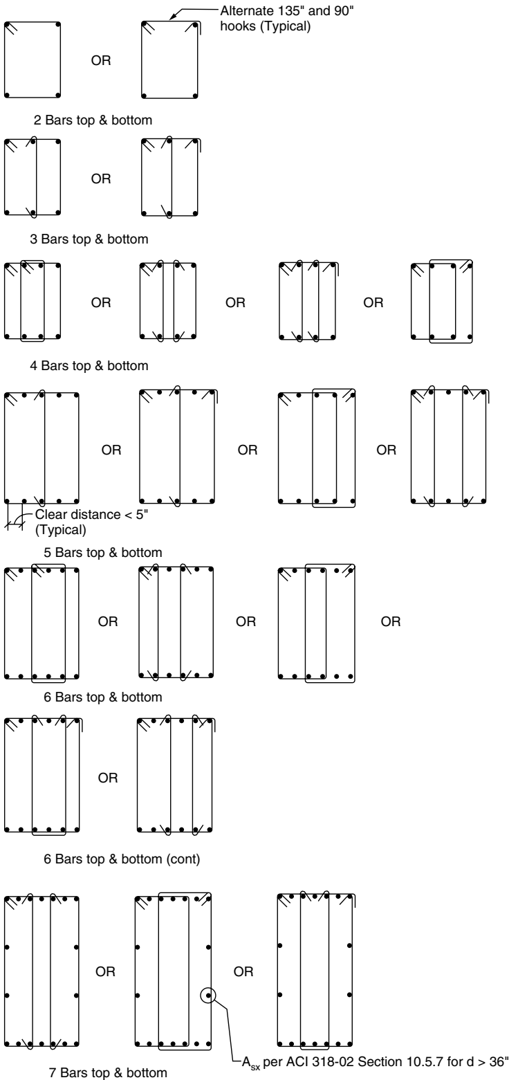
Figure 4.28. Arrangement of hoops and cross-ties; frame beams; special moment frame.
