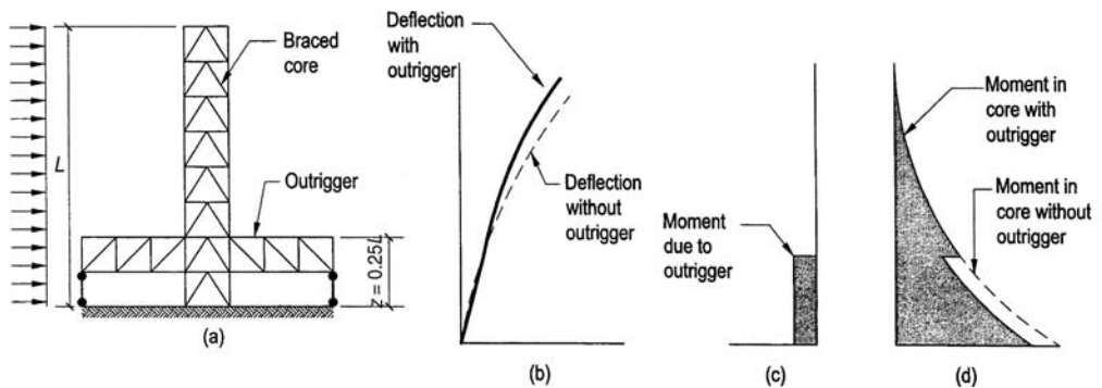
Figure 3.22. Outrigger at quarter-height, z = 0.25L .
