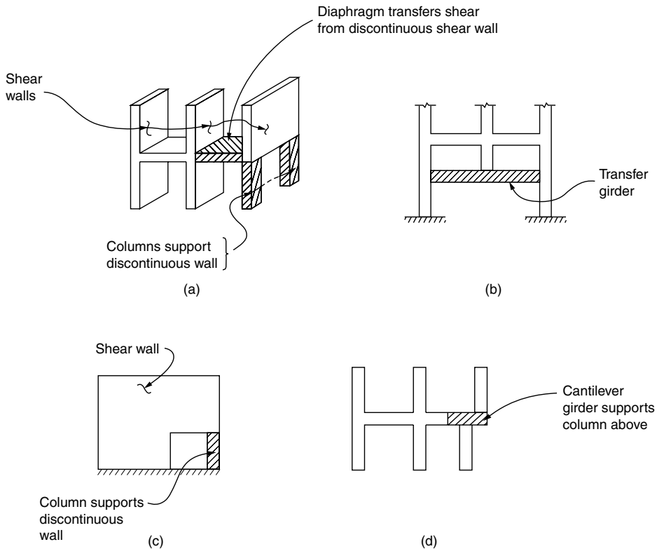
Figure 2.42. Examples of nonuniform ductility in structural systems due to vertical discontinuities. (Adapted from SEAOC Blue Book, 1999 Edition.)
