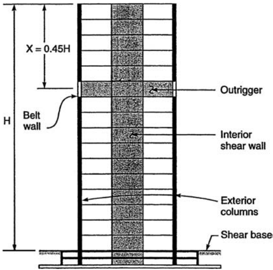
Figure 4.11. Single outrigger system: optimum location.
