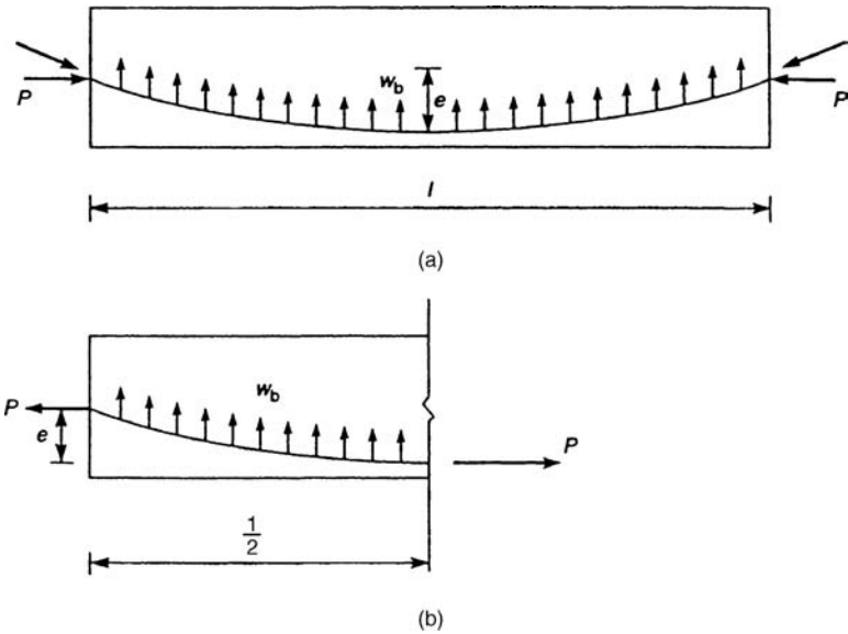
Figure 7.33. Load balancing concept: (a) beam with parabolic tendon; (b) free-body diagram.
