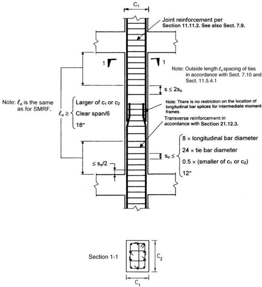
Figure 4.22. Intermediate moment-resisting frame; transverse reinforcement requirements for frame columns.
