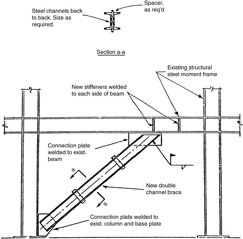
Figure 6.22. Strengthening of an existing building with eccentric bracing.
