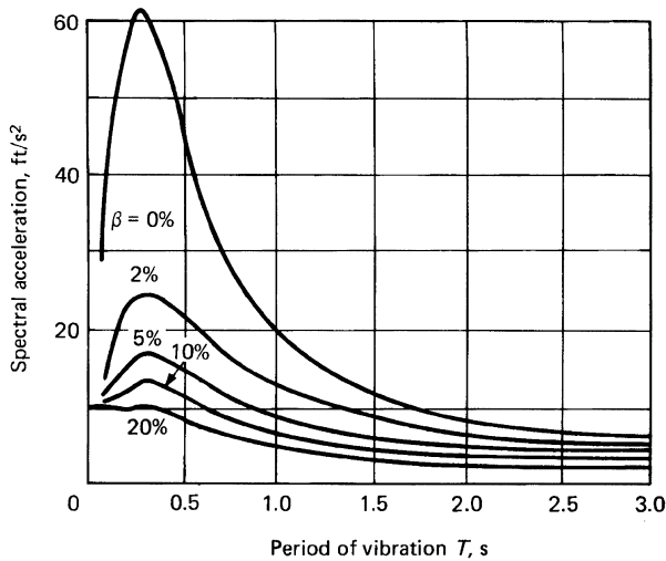
Figure 2.19. Smoothed acceleration spectra for the El Centro earthquake.
