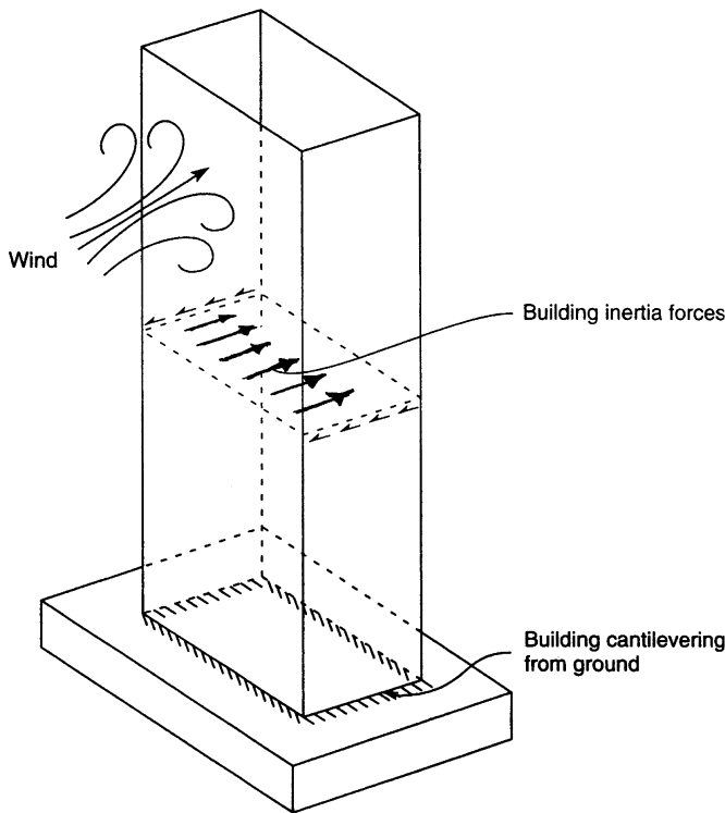
Figure 8.1. Structural concept of a building subjected to lateral forces.
