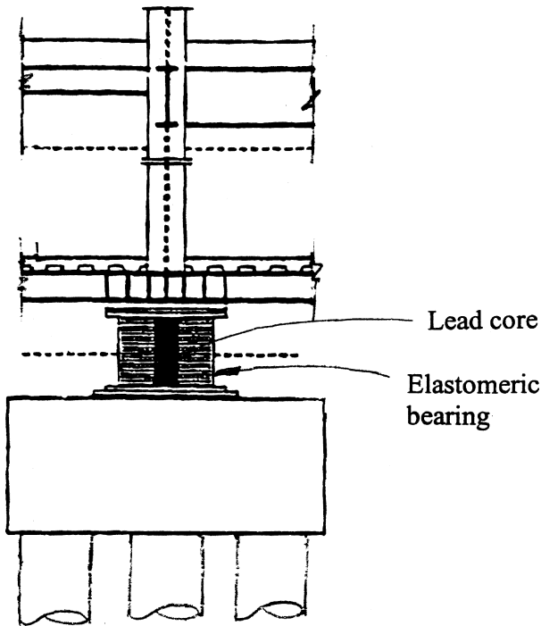
Figure 8.34f. Installation of a lead-rubber bearing under interior columns. A lead-rubber bearing (LRB) consists of one or more lead plugs inserted into holes preformed in low-damping rubber bearings. The lead core provides for energy dissipation by deforming plastically at a stress of 1500 psi (10 Mpa).
