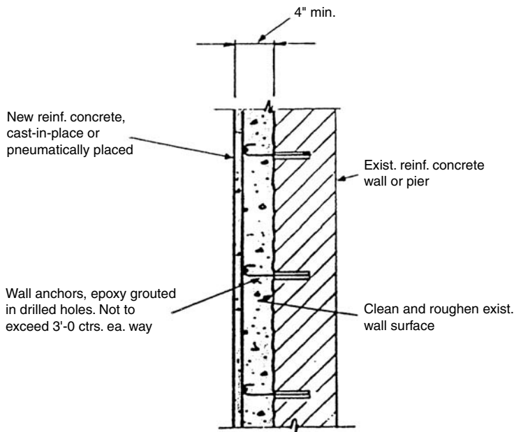
Figure 6.16. Strengthening of existing reinforced concrete walls or piers.
