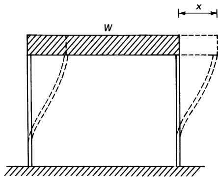
Figure 2.65. Single-bay single-story portal frame.
