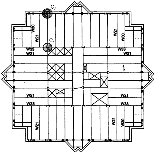
Figure 8.32k. Framing plan. Column C_1 , designed for gravity loads only, shortens more than C_2 , designed for both gravity and lateral loads. Compensating for relative elevation difference between these two categories of columns is of importance in tall buildings.
