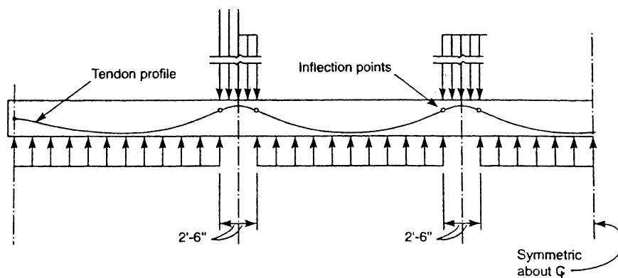
Figure 7.37. Equivalent loads due to prestress.
