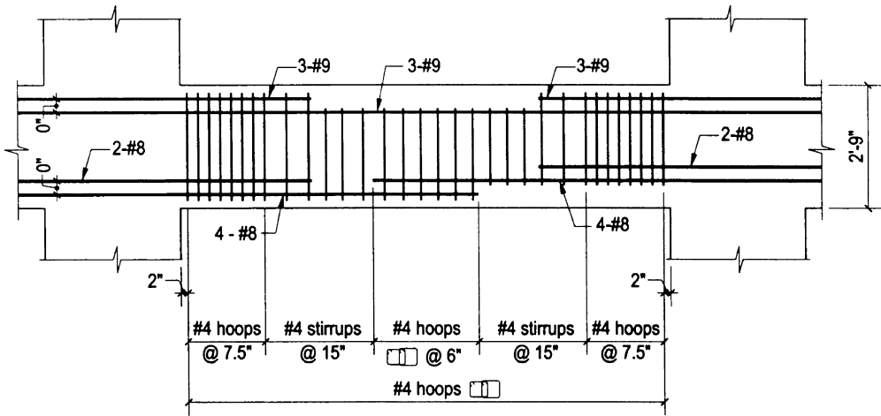
Figure 4.39. Design example, frame beam; special moment frame.
