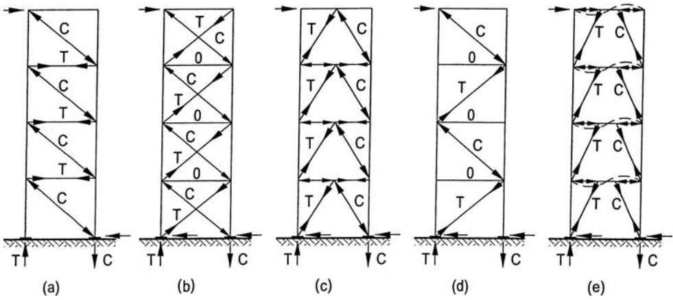
Figure 3.6. Load path for horizontal shear through web members: (a) single diagonal bracing; (b) X-bracing; (c) chevron bracing; (d) single-diagonal, alternate direction bracing; (e) knee bracing.
