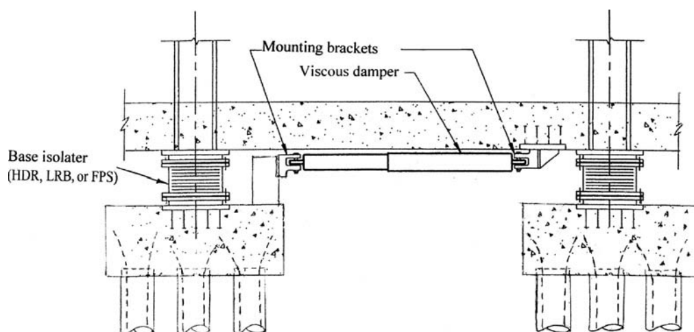
Figure 8.34k. Base isolator operating in concert with a viscous damper.
