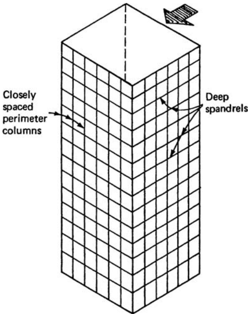
Figure 3.32. Isometric view of framed tube.
