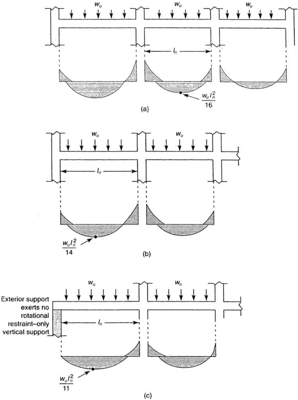
Figure 7.11. ACI positive moment coefficients: (a) interior span; (b) exterior span, discontinuous end integral with supports; (c) exterior span, discontinuous end unrestrained.
