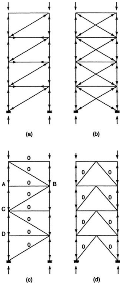
Figure 3.7. Gravity load path: (a) single diagonal single direction bracing; (b) X-bracing; (c) single diagonal alternate direction bracing; (d) chevron bracing.
