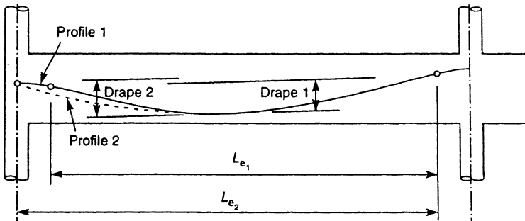
Figure 7.45. End bay tendon profiles.
