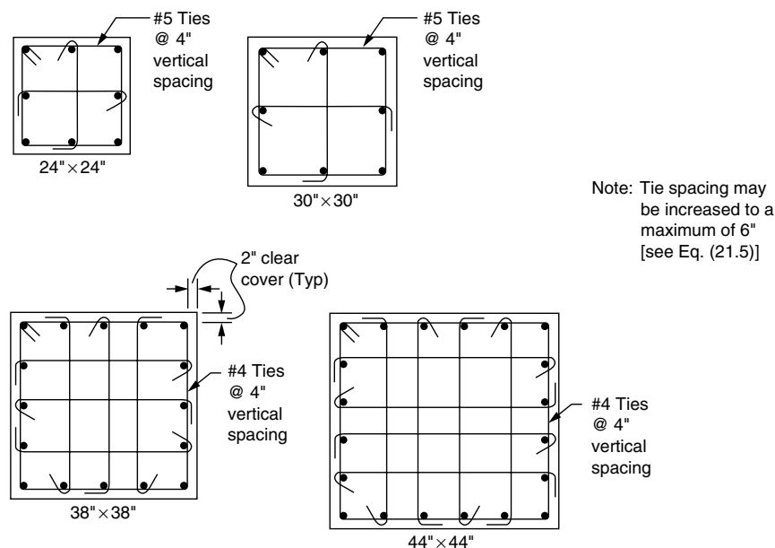
Figure 4.30. Examples of minimum transverse reinforcement in frame columns of SMRF (Eqs. 21.3 and 21.4).
