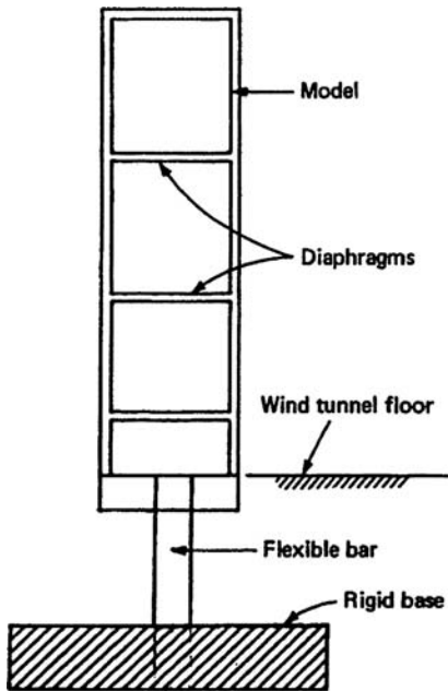
Figure 1.23. Rigid aeroelastic model mounted to flexible steel bar.
