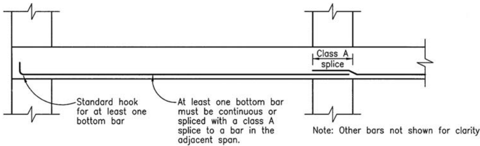
Figure 4.17. Structural integrity reinforcement in joists.
