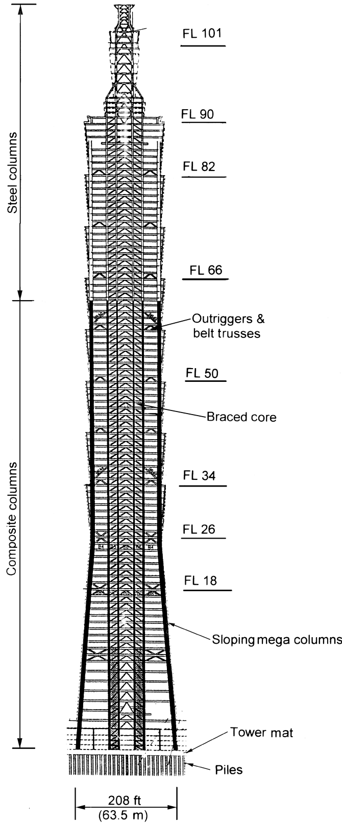
Figure 8.27c. Taipei 101 Office Building schematic cross section.
