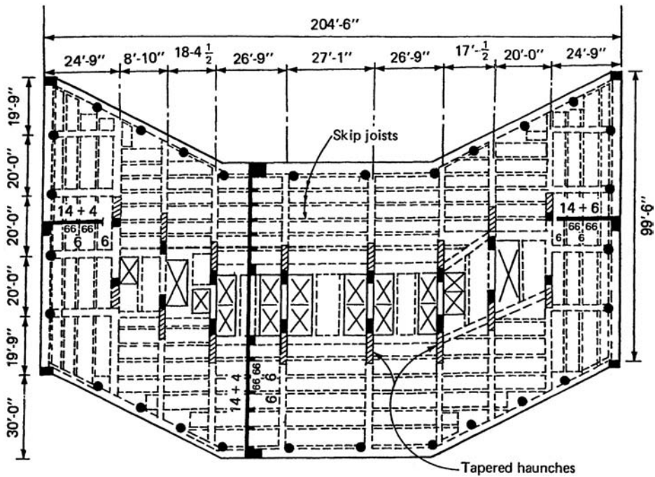
Figure 4.5. A 28-story haunch girder building: typical floor framing plan.
