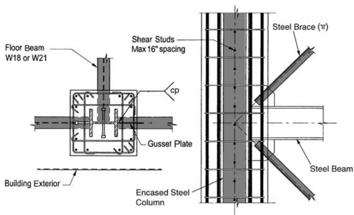
Figure 5.35. Concrete-encased composite column-to-steel concentric brace connection.
