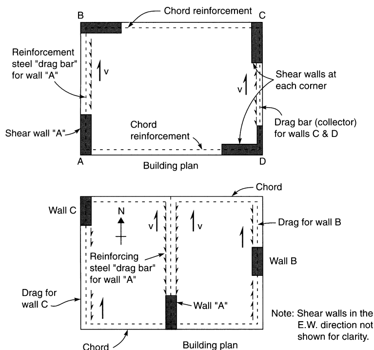
Figure 2.7. Diaphragm drag and chord reinforcement for north-south seismic loads.
