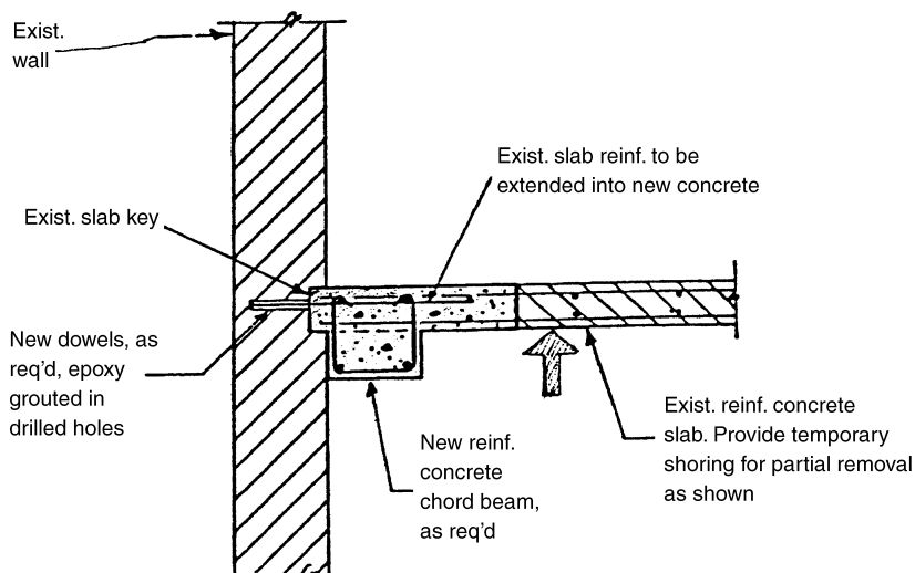
Figure 6.3. Diaphragm chord for existing concrete slab.
