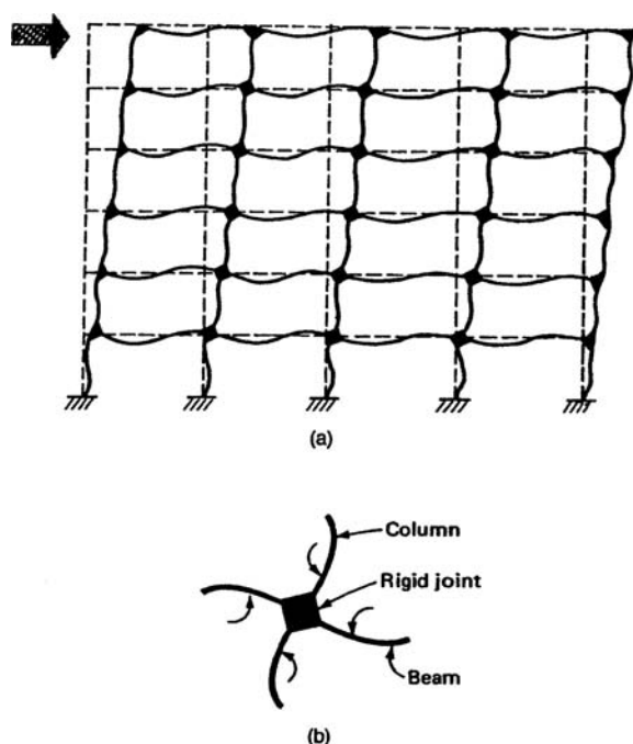
Figure 3.2. (a) Response of rigid frame to lateral loads; (b) flexural deformation of beams and columns due to nondeformability of connections.
