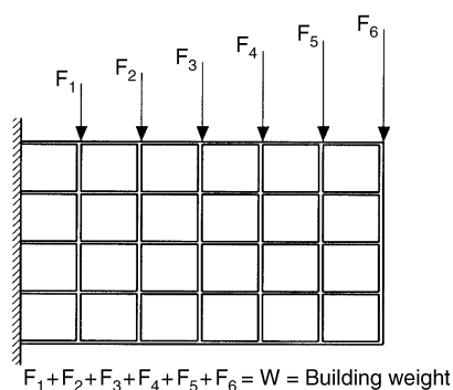
Figure 2.3. Concept of 100% g . A building subjected to an acceleration of 100% g conceptually behaves as if it cantilevers horizontally from a vertical surface.
