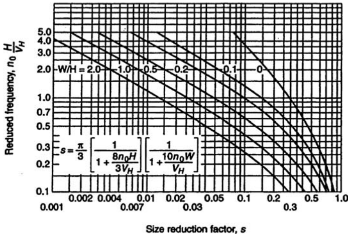
Figure 1.17. Size reduction factor as a function of width, height, and reduced frequency of structure. (From NBCC 1995.)
