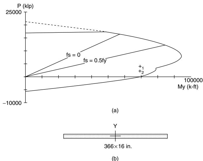
Figure 4.43. (a) Shear wall interaction diagram; (b) cross section of wall.
