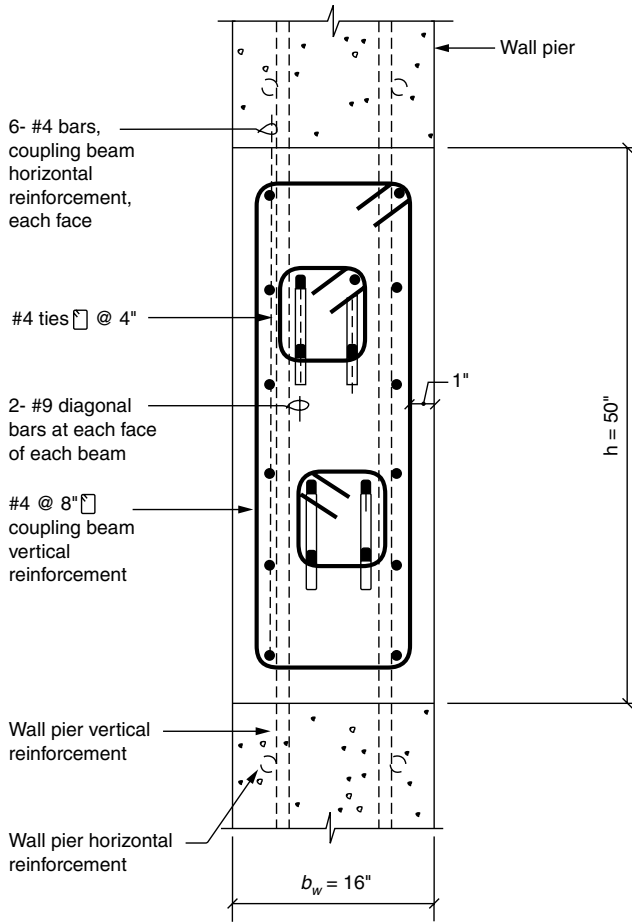
Figure 4.50. Section 1-1. Schematic section through coupling beam. The purpose of this sketch is to ensure that the wall is thick enough for the proper placement of wall and diagonal beam reinforcement and concrete.
