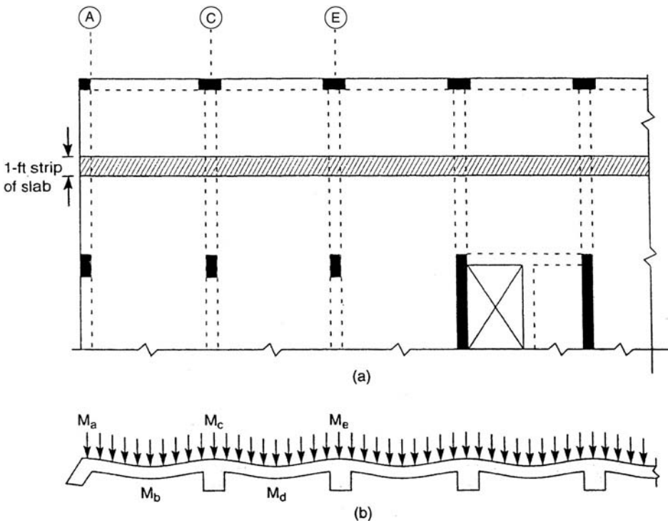
Figure 7.13. Design example, one-way slab: (a) partial floor plan; (b) section.
