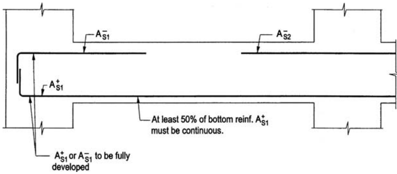
Figure 4.25. Seismic detailing requirements for two-way slabs in areas of moderate seismic risk; middle strip.
