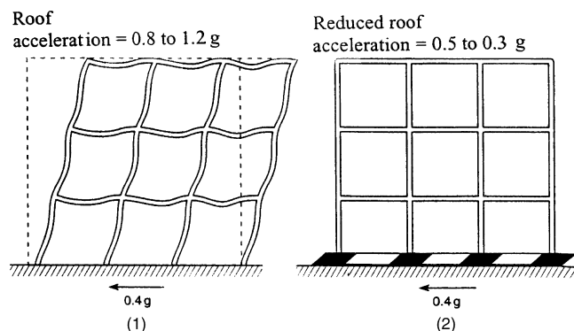
Figure 8.34b. Comparison of response of a fixed-base and a base-isolated building: (1) fixed-base; (2) base-isolated. Base isolation typically reduces roof acceleration of low-rise buildings by about 60 to 80%.
