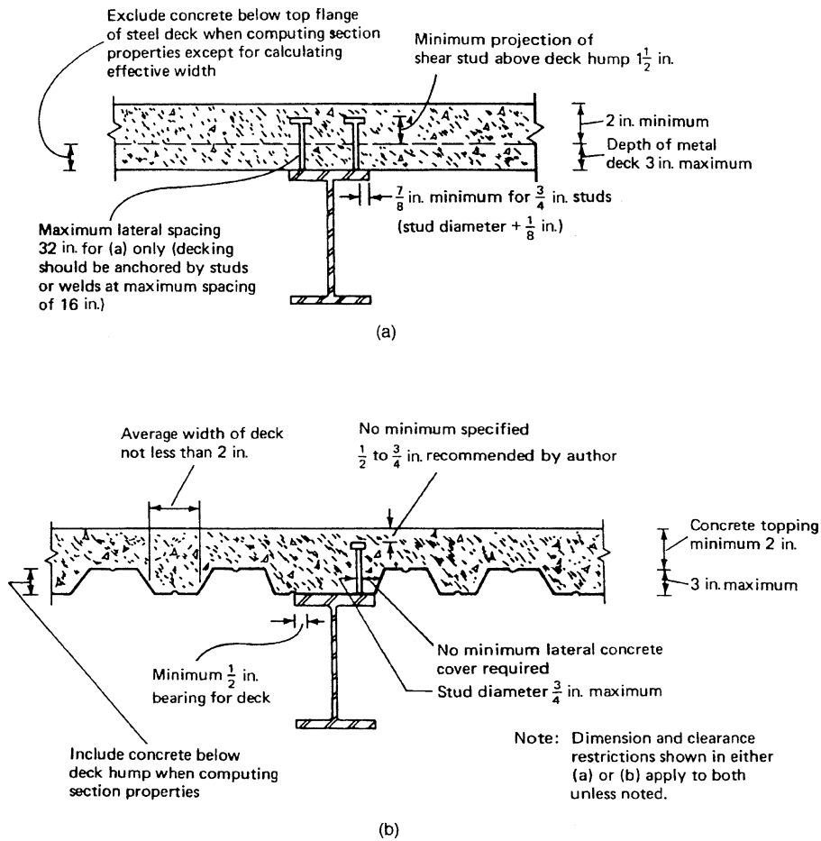
Figure 7.53. Composite beam, AISC requirements: (a) deck perpendicular to beam; (b) deck parallel to beam.
