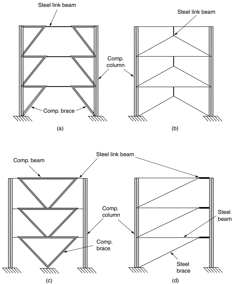
Figure 5.36. Examples of composite eccentrically braced frames.
