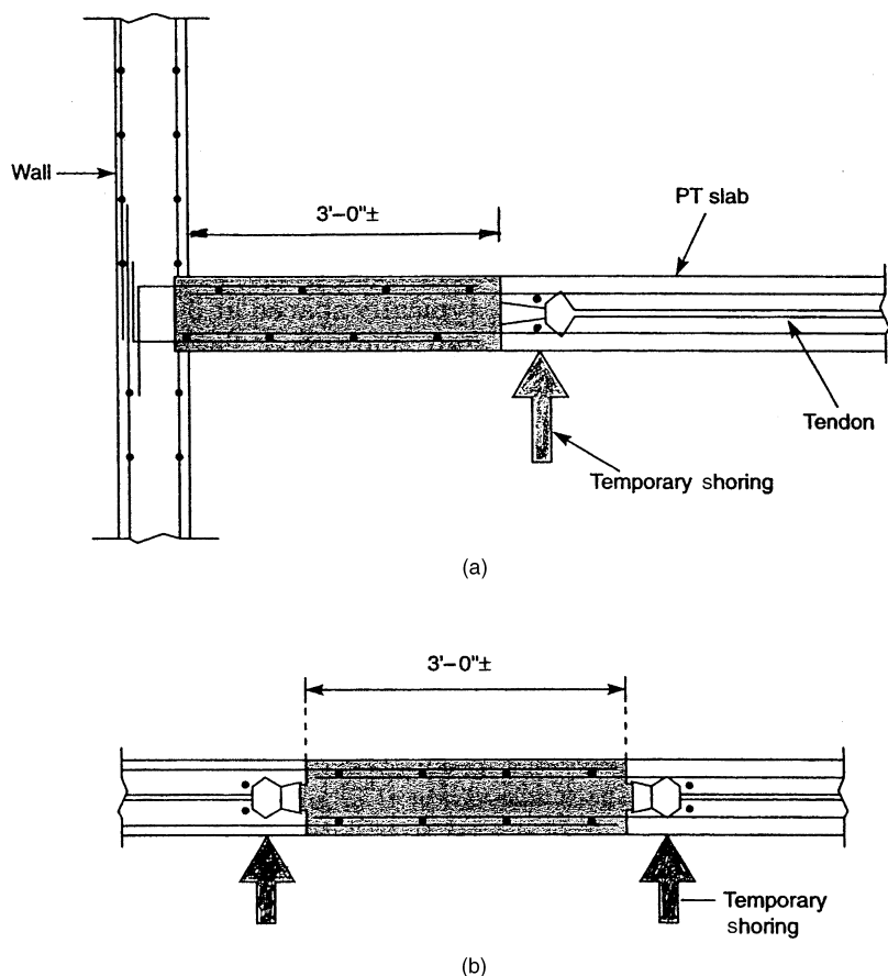
Figure 7.29. Temporary pour strip: (a) at perimeter of building; (b) at interior of slab.
