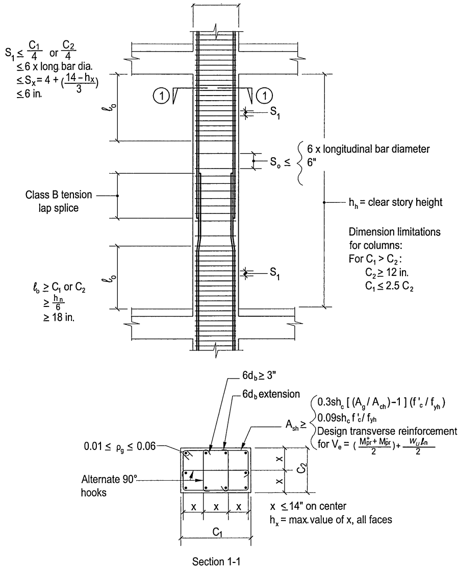
Figure 4.29. Frame column; detailing requirements, special moment frame.
