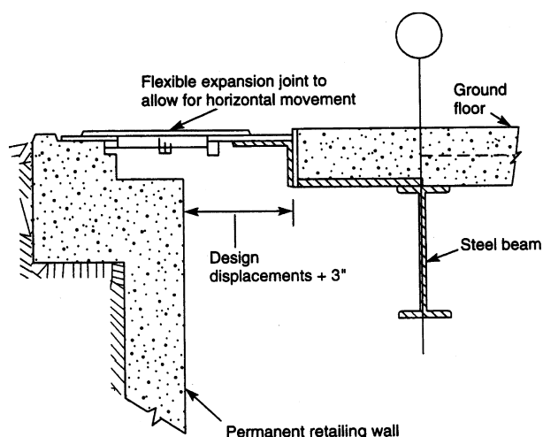
Figure 8.34d. Moat detail at ground level.
