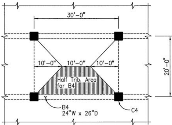
Figure 4.35. Frame beam and column example; intermediate moment frame.
