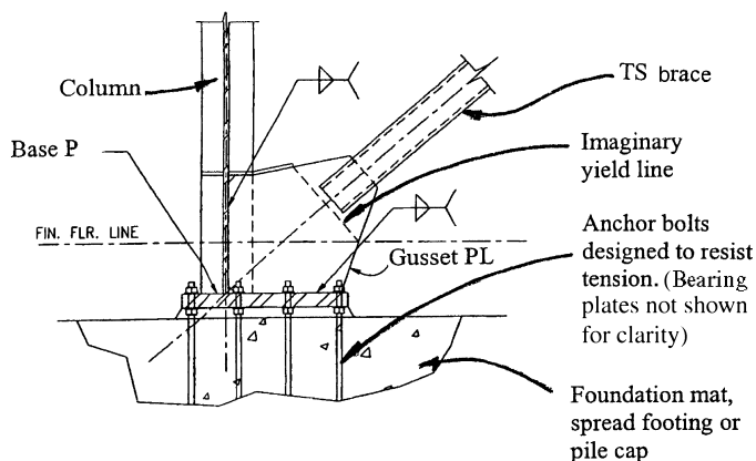
Figure 3.49. Column and brace connection at foundation. (Courtesy of Louis Choi, S.E., John A. Martin & Assoc. Structural Engineers, Los Angeles, CA.)
