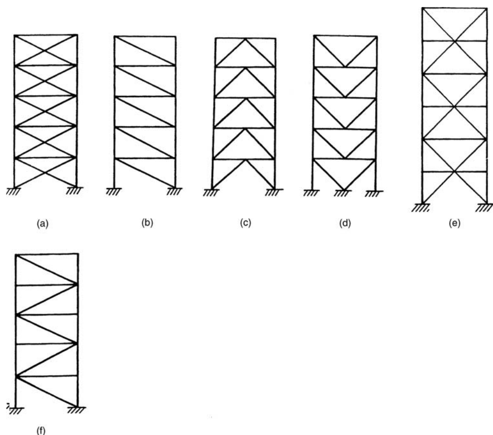
Figure 3.8. Typical concentric braced frame (CBF) configurations: (a) one-story X-bracing; (b) single-diagonal bracing; (c) and (d) chevron bracing; (e) two-story X-bracing; (f) single-diagonal, alternate-direction bracing.
