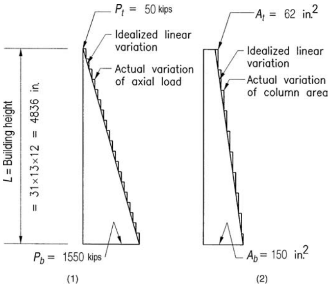
Figure 8.32j. Example 2, exterior column H.3-6: (1) axial load variation; (2) variation of cross-sectional areas.
