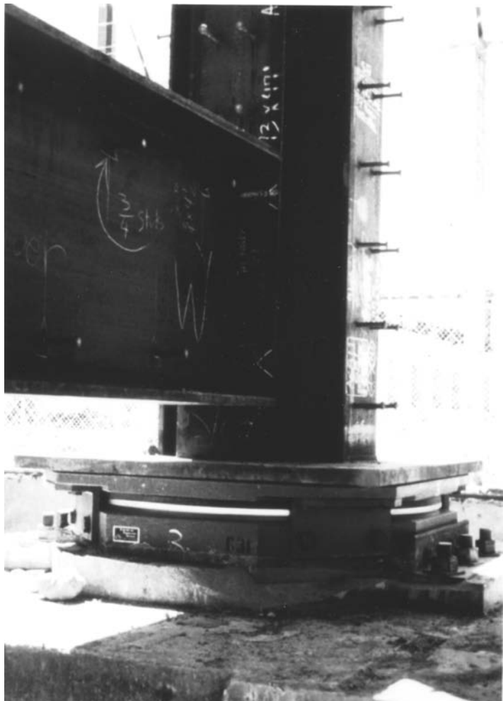
Figure 8.34j(3). FPS bearing in new construction.
