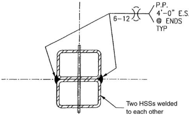
Figure 3.42. Built-up brace detail for use in an SCBF. (Courtesy of Louis Choi, S.E., John A. Martin & Assoc. Structural Engineers, Los Angeles, CA.)
