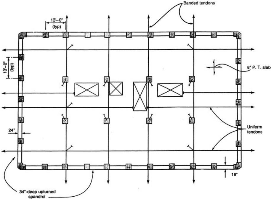
Figure 7.26 Two-way post-tensioned flat plate system for a residential tower, the Museum Tower, in Los Angeles, CA. (Structural engineers John A. Martin & Assoc., Inc., Los Angeles, CA.)
