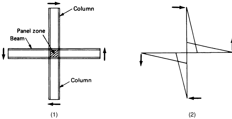
Figure 8.31a. Typical frame element: (1) free-body diagram; (2) bending moments due to shear in beam and columns.
