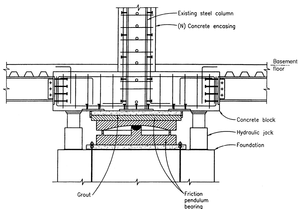
Figure 8.34j(1). Installation details of FPS bearing under existing interior columns.
