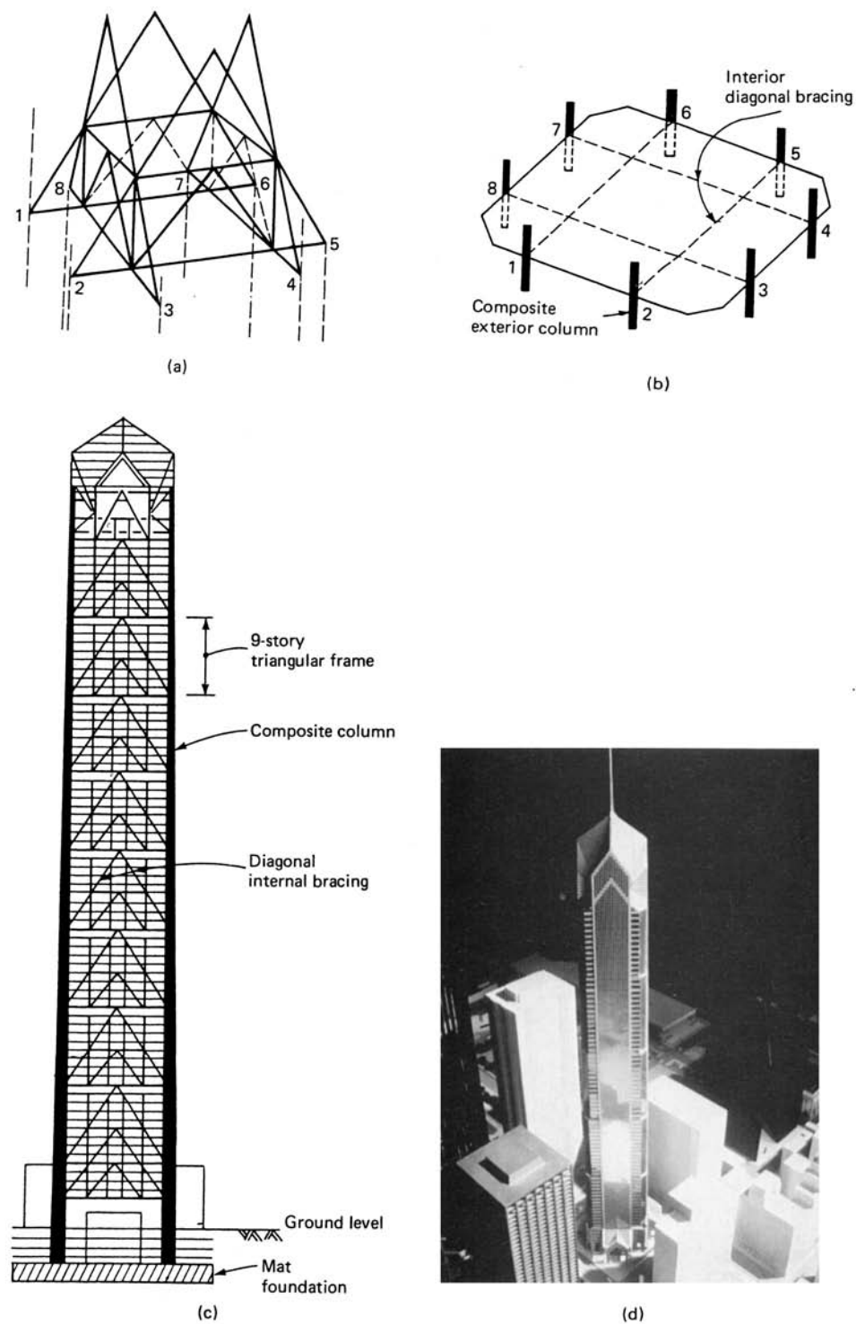
Figure 5.21. Bank of Southwest Tower (structural engineers: LeMessurier Associates and Walter P. Moore Associates; architects: Murphy/Jahn and Lloyd Jones and Fillpot). (a) Schematic representation of interior diagonal bracing; (b) schematic plan; (c) schematic section; (d) photograph of model. (Photo courtesy of Malcolm Stewart, Century Development Corporation.)
