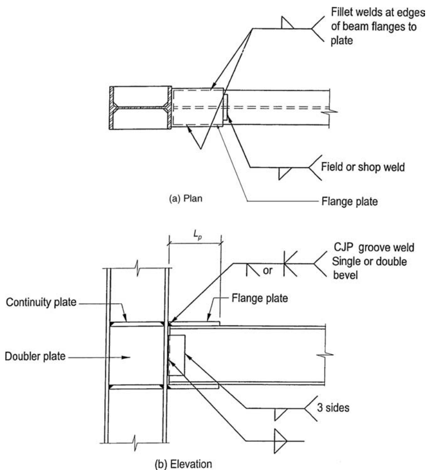
Figure 3.58. Prequalified welded flange plate (WFP) connection.
