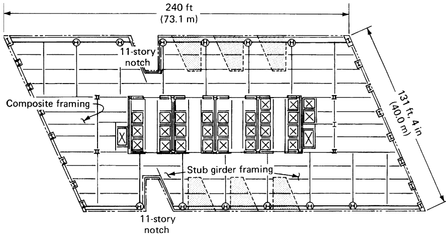
Figure 5.22. Composite floor-framing plan.
