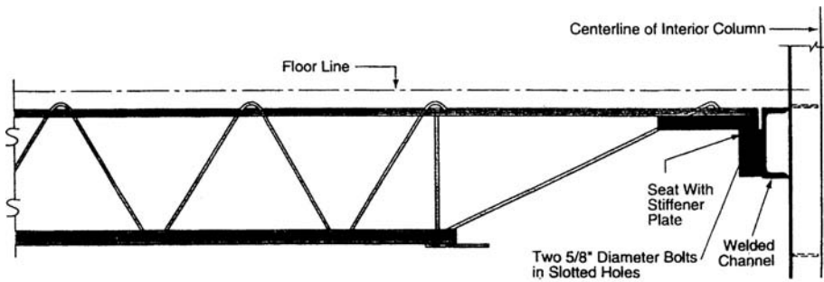
(j) Detail B - Interior Wall End Detail
