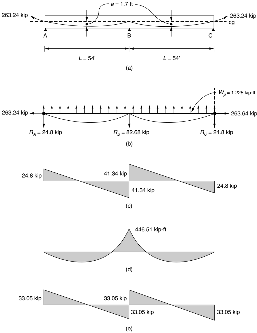
Figure 7.31A. Concept of secondary moments—example 2A: (a) two-span continuous prestressed beam; (b) equivalent loads due to prestress, consisting of upward UDL, horizontal compression due to prestress W_p , and downward loads at A, B, and C; (c) shear force diagram, statically indeterminate beam; (d) moment diagram, statically indeterminate beam; (e) primary shear force diagram; (f) primary moment diagram; (g) secondary shear forces; (h) secondary moments.
