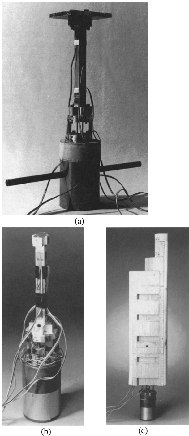
Figure 1.28. High-frequency force balance model: (a, b) Close-up views of base; (c) high-rise model at the base. (Photo courtesy of Dr. Peter Irwin, Rowan, Williams, Davis & Irwin, Inc.)
