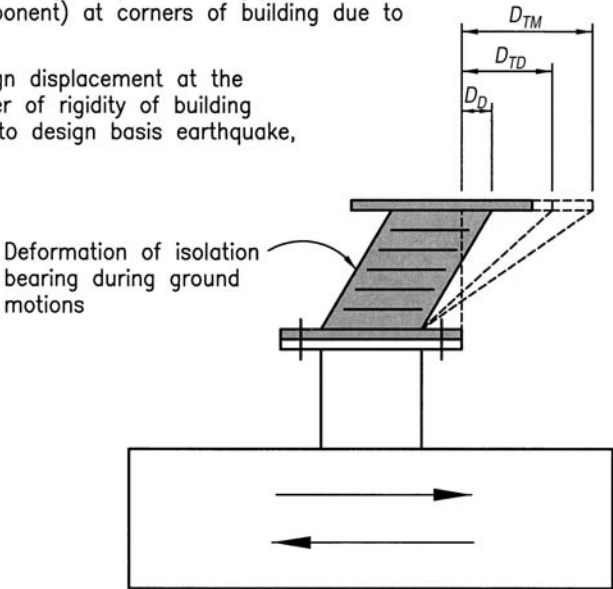
Figure 8.34I. Isolator displacement terminology. Note: MCE = earthquake corresponding to 2% probability of exceedence in a 50-year period (2500-year return period); DBE = earthquake corresponding to 10% probability of exceedence in a 50-year period (475-year return period).
