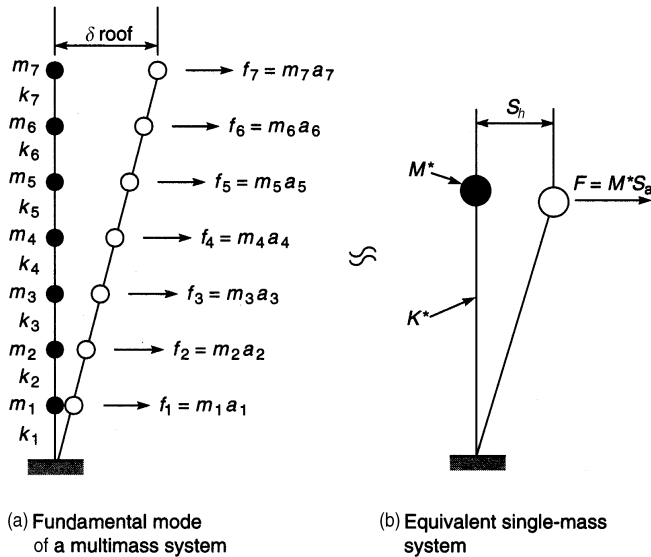
Figure 2.14. Representation of a multimass system by a single-mass system.
