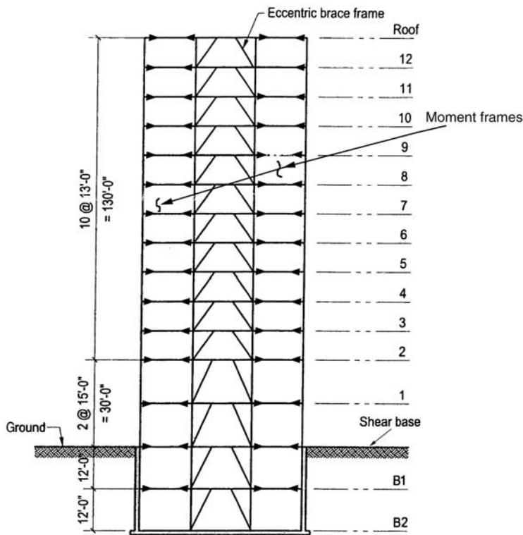
Figure 2.46. Design example; ASCE 7-02 (IBC-03), static force procedure.
