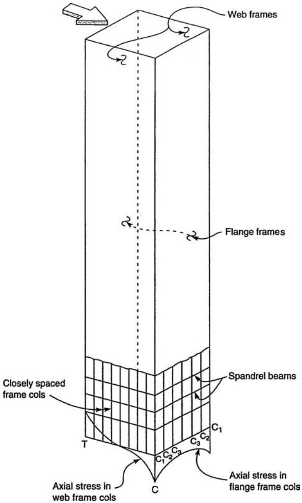
Figure 3.35. Shear lag in framed tube. Observe that the axial stresses are distributed quite differently from those predicted by engineer’s bending theory.
