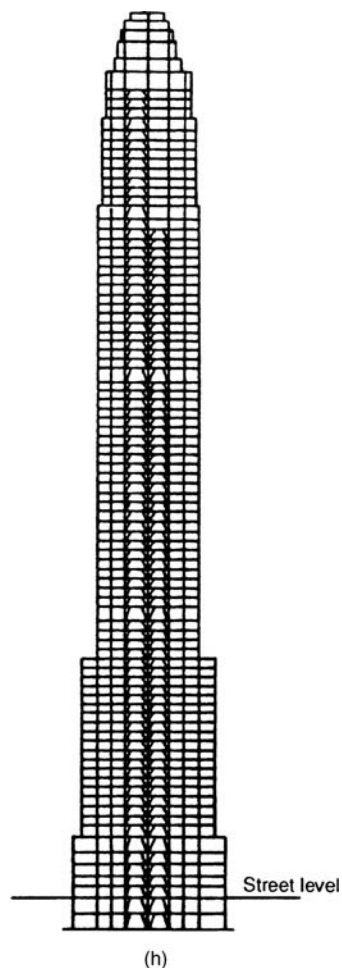
Figure 3.9h. Empire State Building bracing system; riveted structural steel frame encased in cinder concrete.
