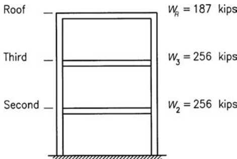
Figure 2.50. Three-story building example; dynamic analysis.
