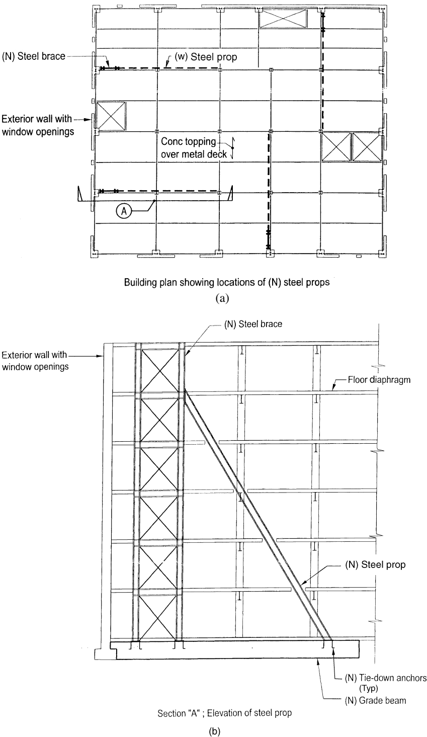
Figure 6.24. (a) Building plan showing location of (N) steel props; (b) section A; elevation of (N) steel prop.
