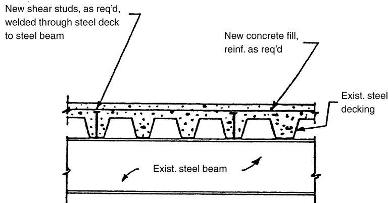
Figure 6.6. Strengthening of existing steel deck diaphragms.
