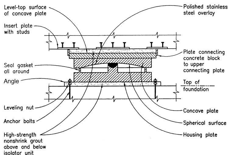
Figure 8.34i. Friction pendulum system details. The P\Delta effect in this arrangement, where \Delta = earthquake-induced displacement, is accounted for in the design of the superstructure. If the spherical plate is attached to the foundation, the P\Delta effect is accounted for in the design of the foundation.
