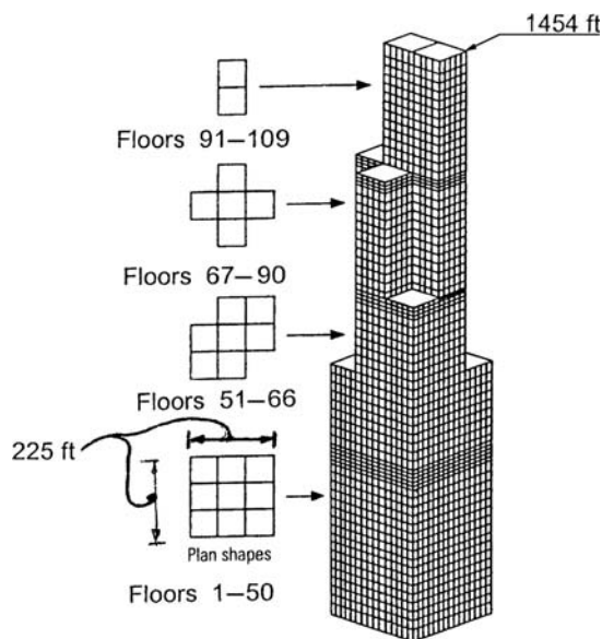
Figure 3.39. Bundled tube structural system; Sears Tower, Chicago. Building height: 1454 ft.
