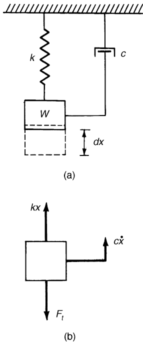
Figure 2.67. Damped oscillator: (a) analytical model; (b) forces in equilibrium.
