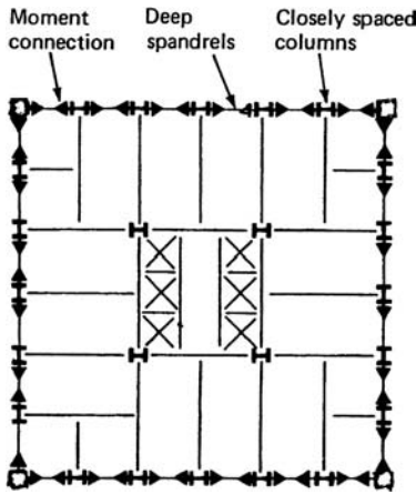
Figure 3.31. Schematic plan of framed tube.
