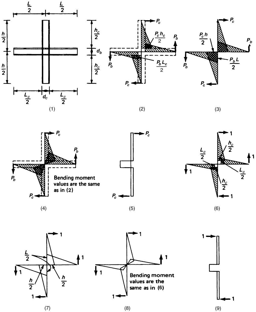
Figure 8.31c. Typical frame segment: (1) geometry; (2) bending moment diagram with rigid panel zone; (3) bending moment diagram without panel zone; (4) bending moment diagram with flexible panel zone; (5) shear force diagram; (6–9) unit load diagrams.
