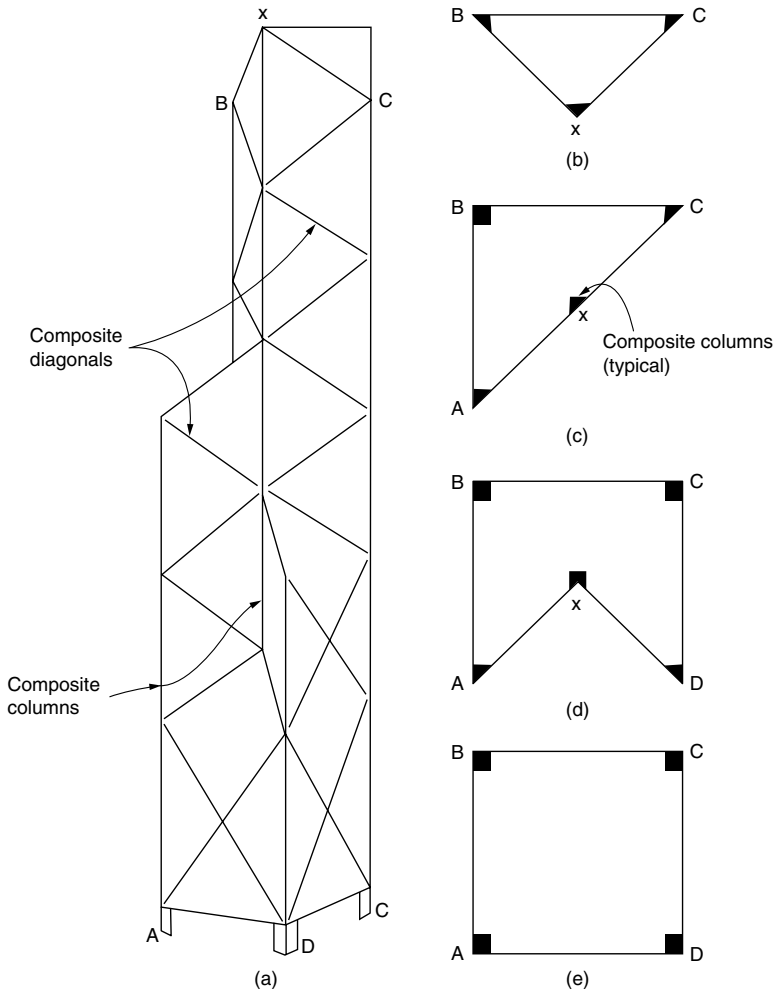
Figure 5.20. Bank of China Tower, Hong Kong.
