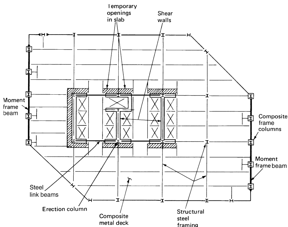
Figure 5.11. Typical floor plan of a composite building using shear wall-frame interaction.
