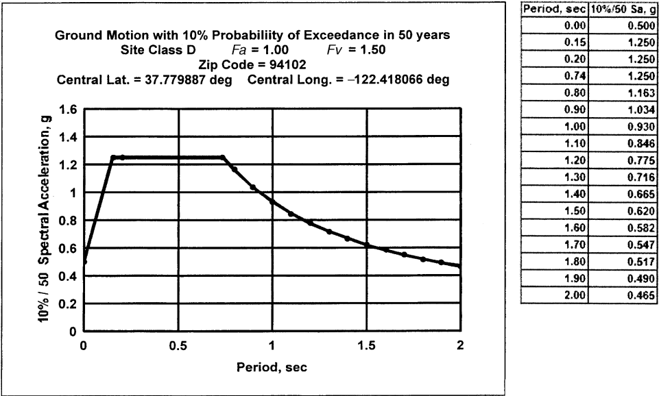
Figure 2.43. Design basis earthquake ground motions; 10% probability of exceedence in 50 years, corresponding to a return period of 474 years, typically rounded to 500 years.
