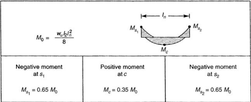
Figure 7.17. Assignment of moments at critical sections: interior span.
