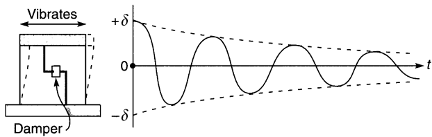
Figure 2.13. Damped free vibration of a single-degree-of-freedom system.
