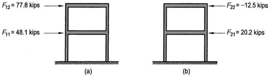
Figure 2.49. Distribution of modal shears: (a) first mode; (b) second mode.
