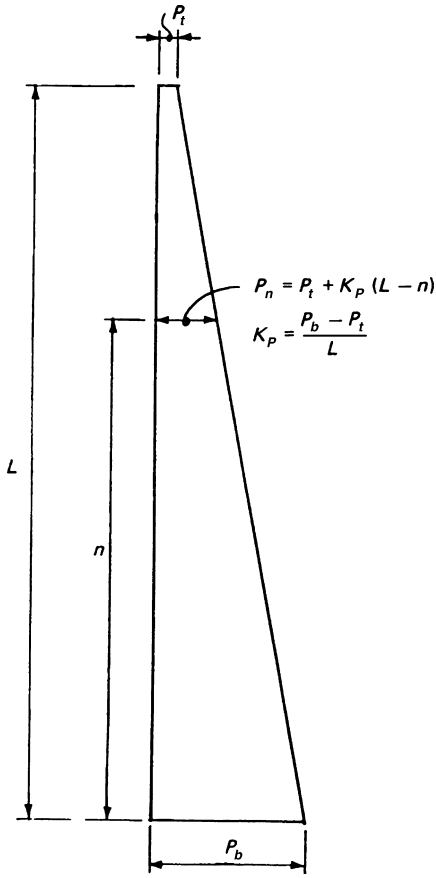
Figure 8.32d. Idealized gravity load distribution on a column.
