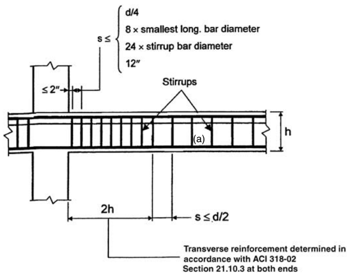
Figure 4.21. Intermediate moment-resisting frame (IMRF); transverse reinforcement requirements for frame beams.
