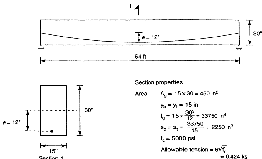
Figure 7.34. Preliminary design: simple span beam.
