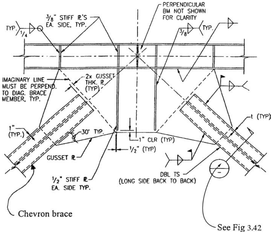
Figure 3.50. Chevron brace-to-beam connection.
