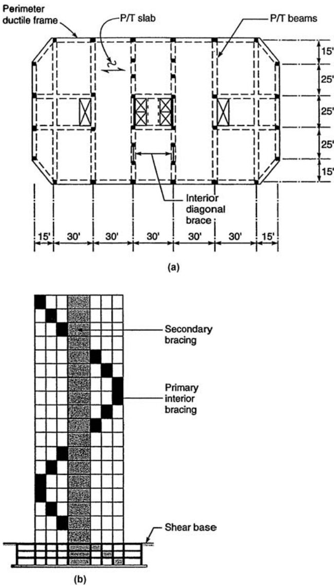
Figure 4.14. Full-depth interior brace: (a) plan; (b) schematic section.
