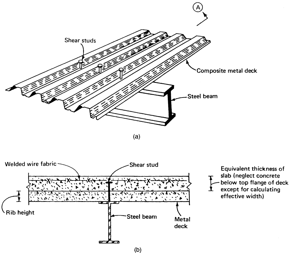
Figure 7.51. Composite beam with deck perpendicular to beam: (a) schematic view; (b) section A showing equivalent thickness of slab.
