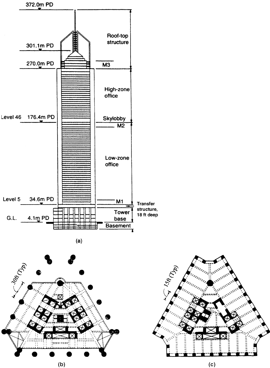
Figure 8.13. Central Plaza, Hong Kong: (a) elevation; (b, c) floor plans.
