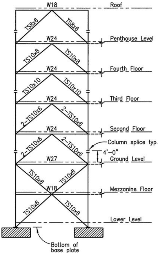
Figure 3.43. Braced frame with story-high chevron inverted-V braces. (Courtesy of Louis Choi, S.E., John A. Martin & Assoc. Structural Engineers, Los Angeles, CA.)
