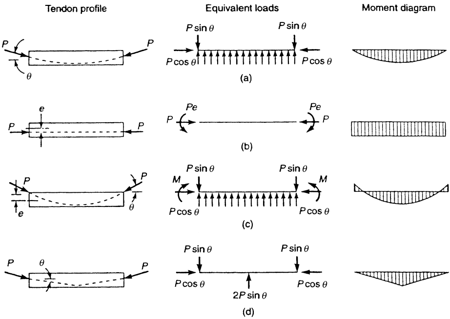
Figure 7.32. Equivalent loads and moments produced by prestressed tendons: (a) upward uniform load due to parabolic tendon; (b) constant moment due to straight tendon; (c) upward uniform load and end moments due to parabolic tendon not passing through the centroid at the ends; (d) vertical point-load due to sloped tendon.
