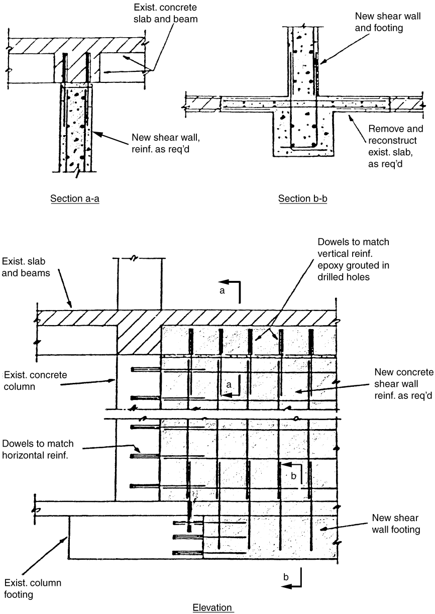
Figure 6.15. Strengthening of an existing concrete frame building with a reinforced concrete shear wall.
