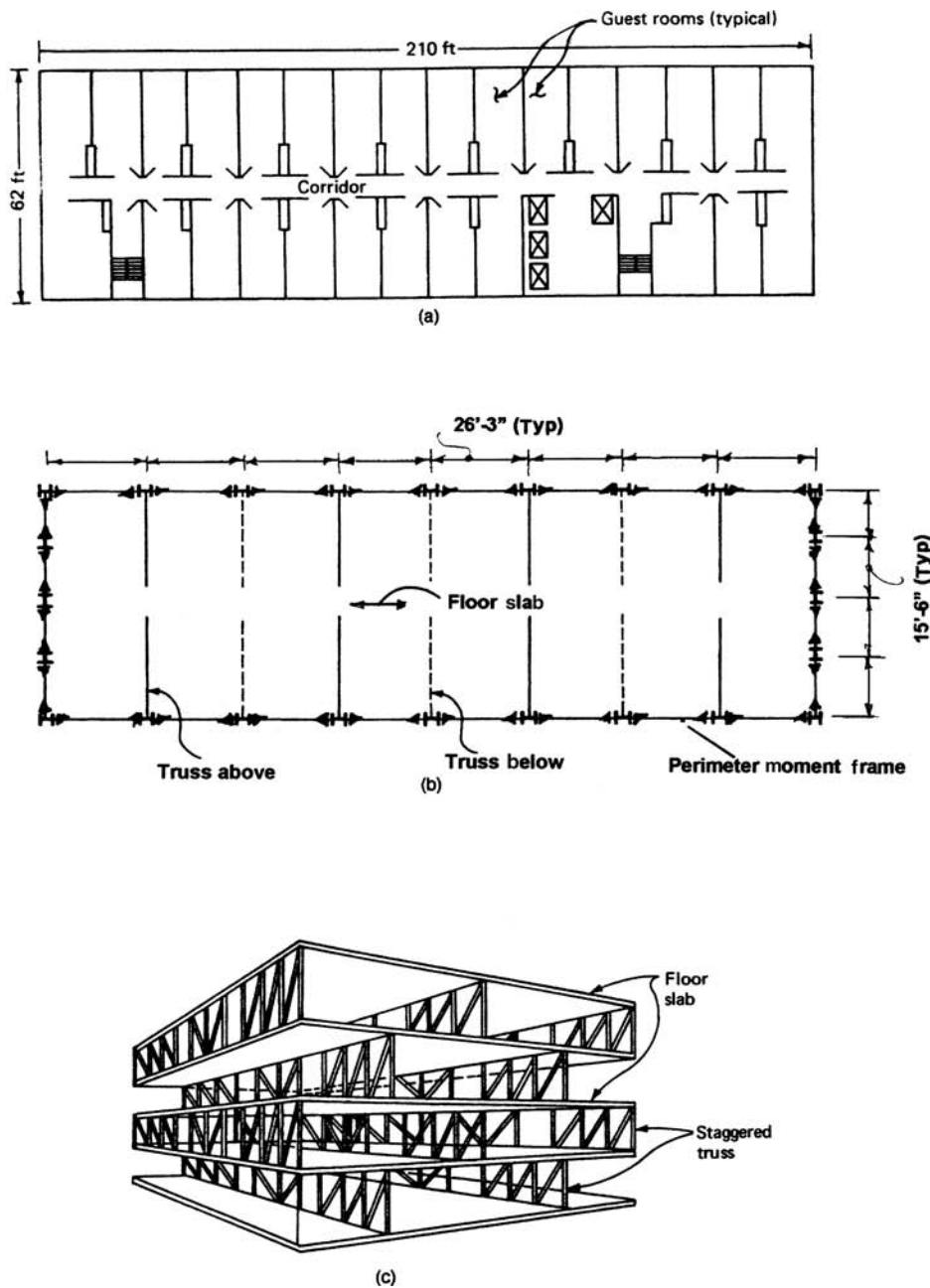
Figure 3.10. Staggered truss system: (a) hotel plan showing guest rooms; (b) arrangement of staggered trusses; (c) perspective view of truss arrangement.
