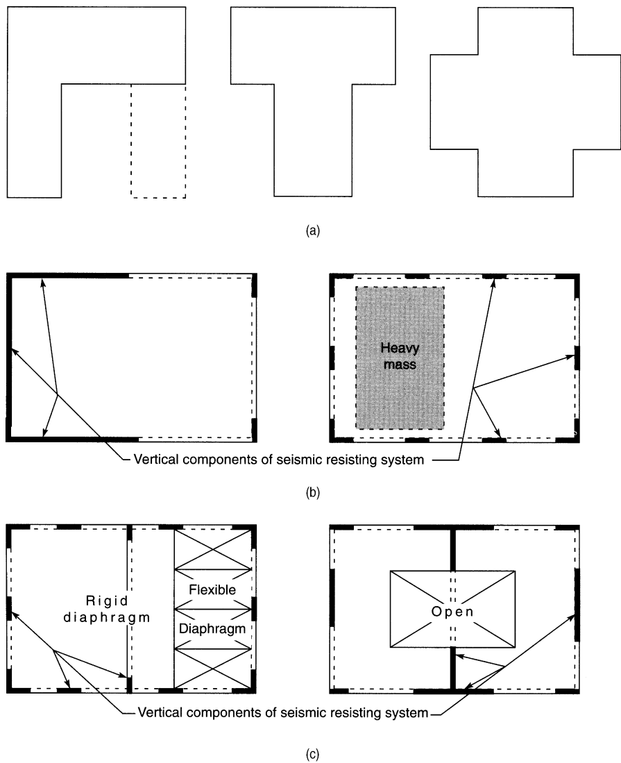
Figure 2.4. Plan irregularities: (a) geometric irregularities; (b) irregularity due to mass-resistance eccentricity; (c) irregularity due to discontinuity in diaphragm stiffness.
