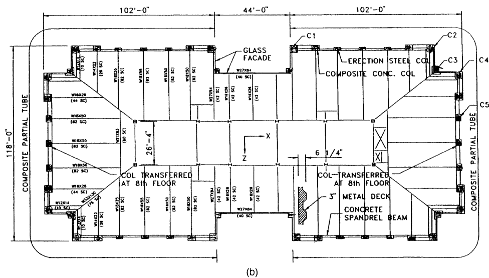
Figure 8.14. One-Ninety-One Peachtree, Atlanta: (a) building elevation; (b) typical floor framing plan.
