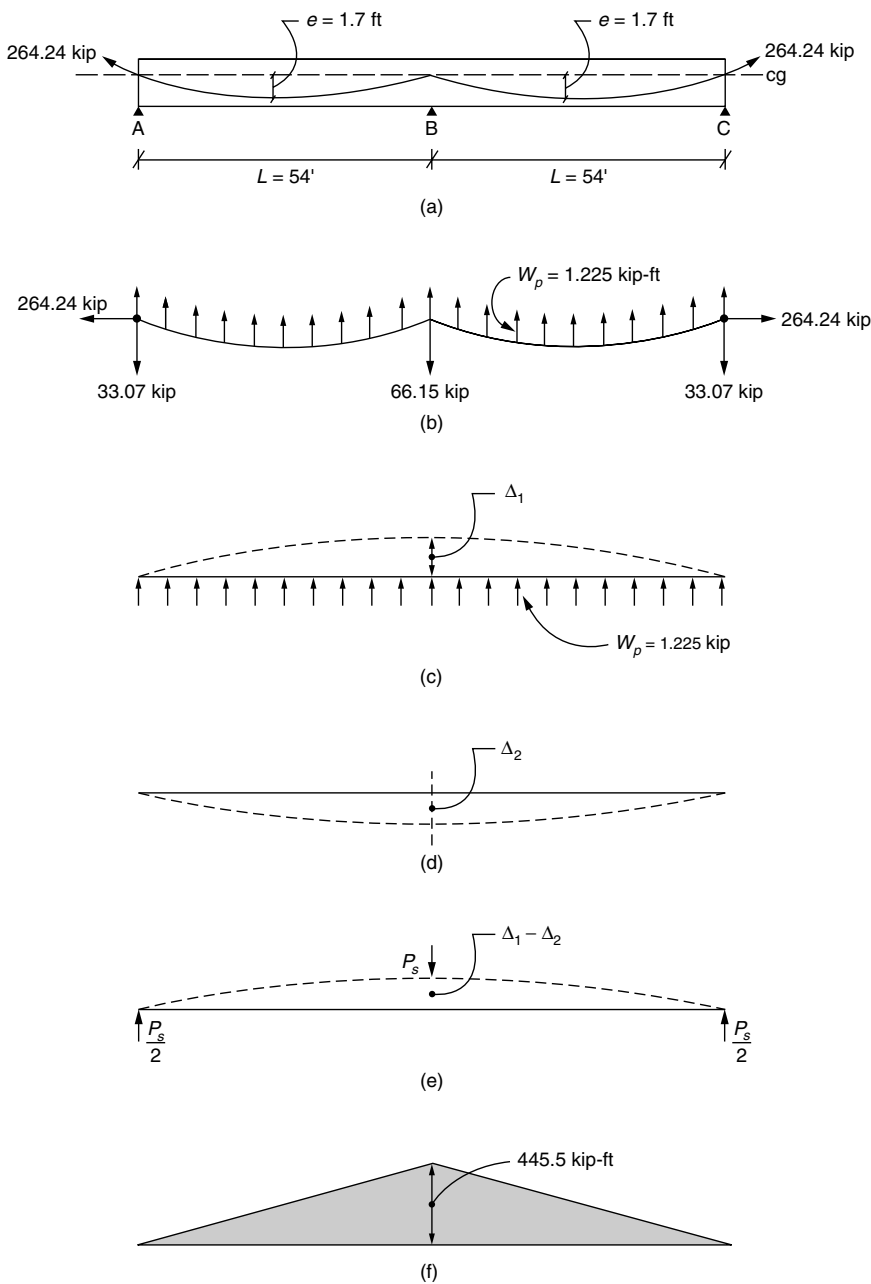
Figure 7.31B. Concept of secondary moments—example 2B, compatibility method: (a) two-span continuous beam; (b) equivalent loads; (c) upward deflection \Delta_1 due to W_p (d) downward deflection \Delta_2 due to a load of 66.15 kips at center span; (e) load P_s corresponding to \Delta_1 - \Delta_2 ; (f) secondary moments.
