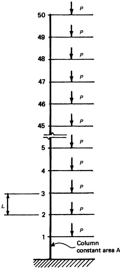
Figure 8.32b. Simplified column for calculation column shortening.
