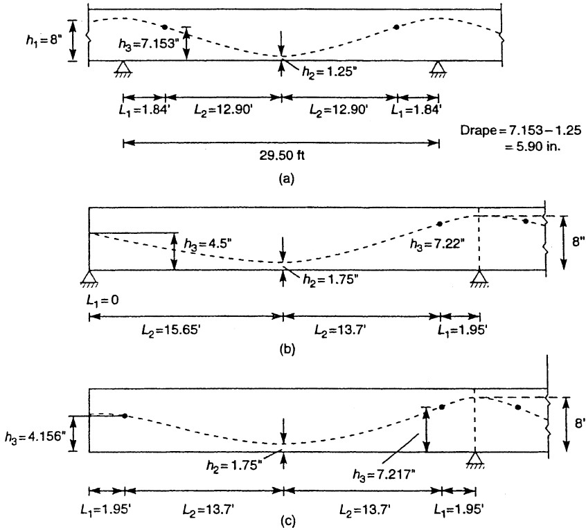
Figure 7.47. Example problem 3: flat plate, tendon profiles: (a) interior span; (b) exterior span, reverse curvature at right support; (c) exterior span, reverse curvature at both supports.
