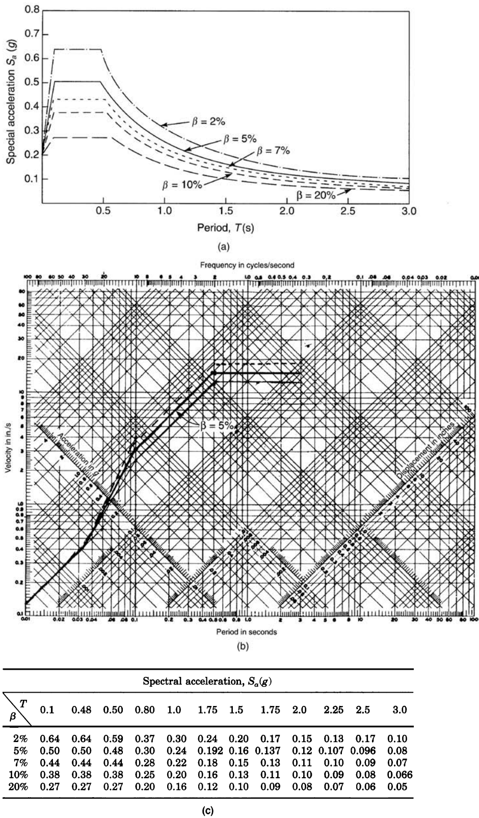
Figure 2.56. Response spectrum for seven-story building example: (a) acceleration spectrum; (b) tripartite diagram; (c) response spectra numerical representation.
