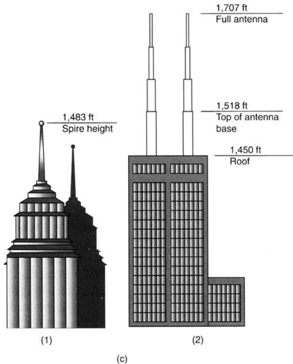
Figure 8.12. Height comparison: (1) Petronas Towers; (2) Sears Tower, Chicago.
