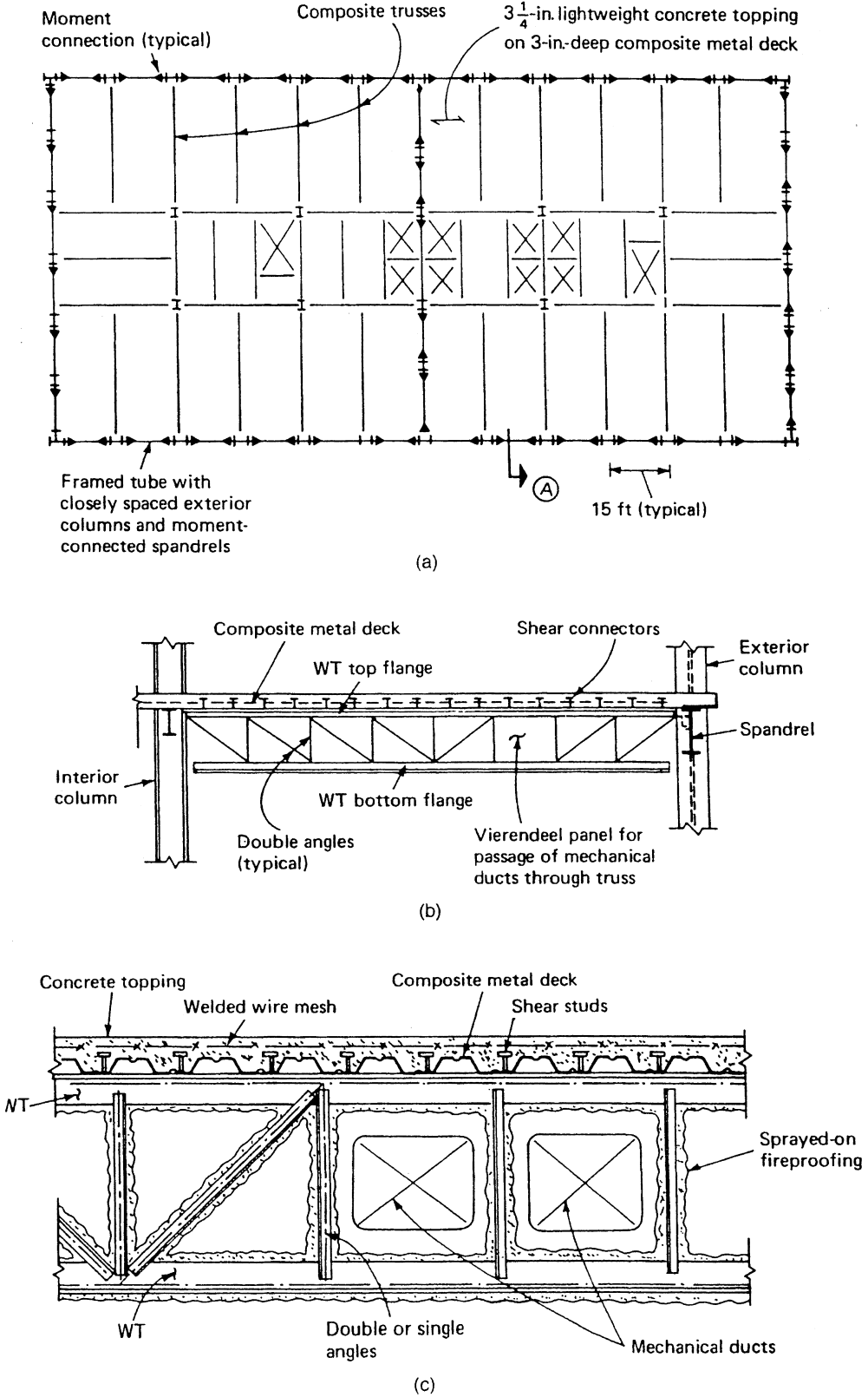
Figure 7.61. Composite truss: (a) framing plan; (b) elevation for truss, section A; (c) detail of truss.
