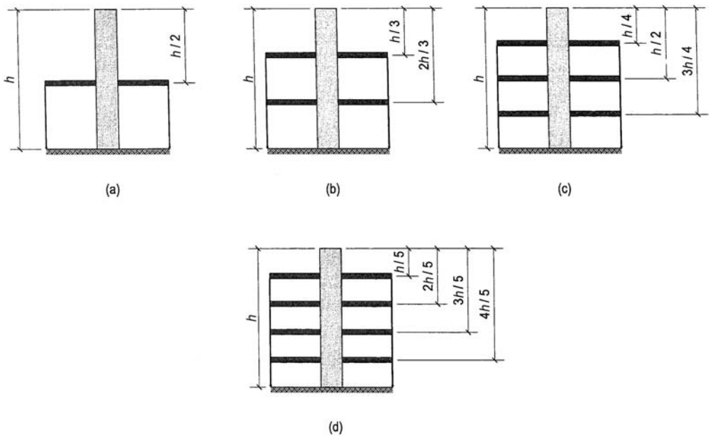
Figure 3.30. Optimum locations of outriggers: (a) single outrigger; (b) two outriggers; (c) three outriggers; (d) four outriggers.
