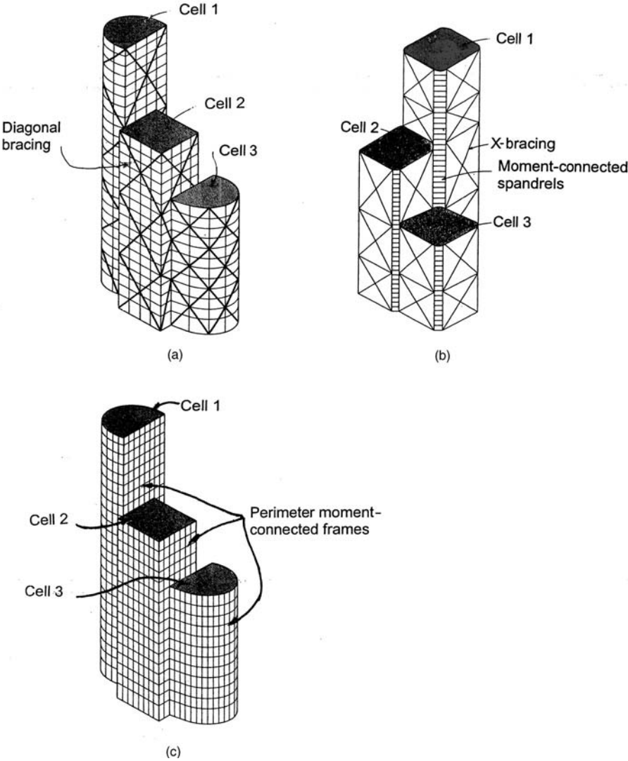
Figure 3.38B. Bundled tube concept: (a) perimeter diagonal bracing; (b) X-bracing with moment-connected spandrels; (c) perimeter moment frames.
