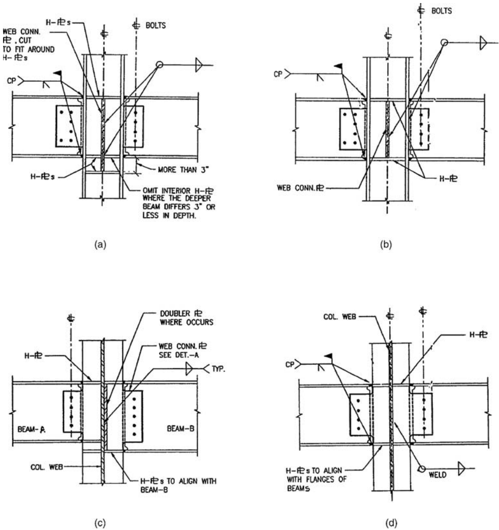
Figure 3.3. Pre-Northridge moment connections: (a) unequal-depth beams to column flange connection; (b) equal-depth beams to column flange connection; (c) unequal-depth beams to column web connection; (d) equal-depth beams to column web connection.
