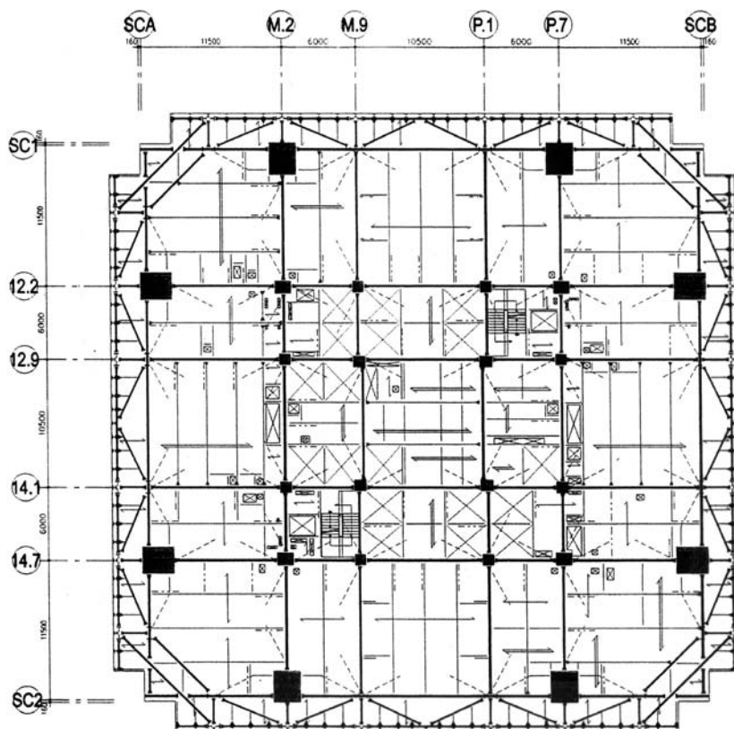
Figure 8.27b. Framing plan for level 50, Taipei Financial Center. The structure consists of a dual system of a braced core connecting to a perimeter sloping frame at each sloping face. The core diagonal and chevron braces are interconnected to vertical supercolumns via outrigger and belt trusses. The supercolumns at the base are 2.4 m \times 3.0 m (approximately 8 ft \times 10 ft).
