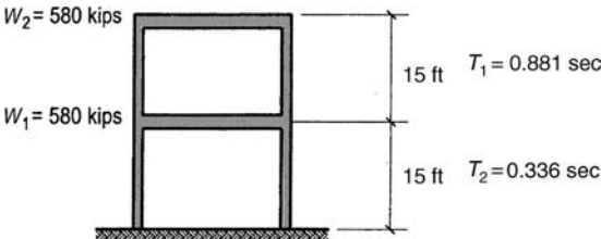
Figure 2.47. Two-story example; dynamic analysis hand calculations.
