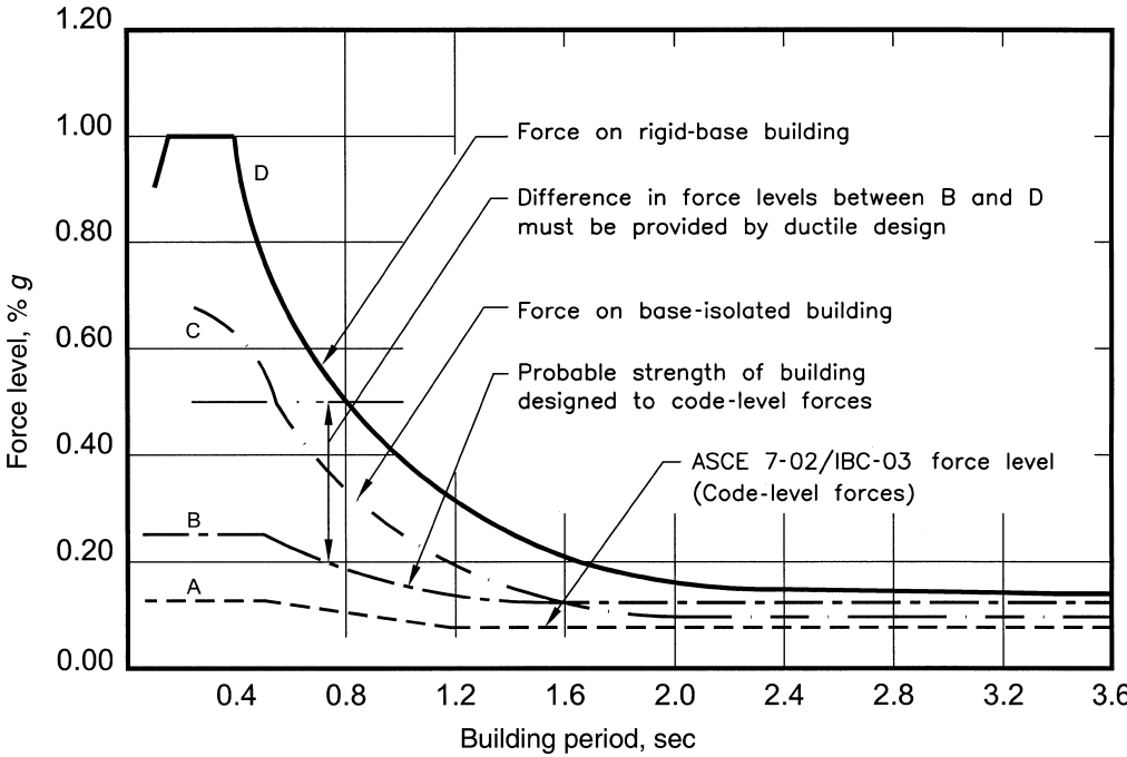
Figure 8.34a. Design concept for base-isolated buildings: Top curve D shows the forces in the structure if it were to remain elastic during an earthquake. The conventional design approach is to build ductility into the structure to absorb the difference in forces between B and D. By providing seismic isolation, the maximum force experienced by the building, curve C, is reduced to its probable strength, curve B.
