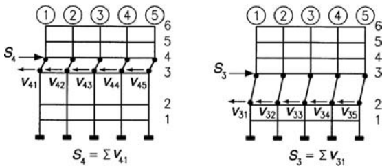
Figure 2.30. Discontinuity in capacity (weak story); story strength at levels 4 and 3. A weak story condition exists when the story strength is less than 80% of that of the story above:
