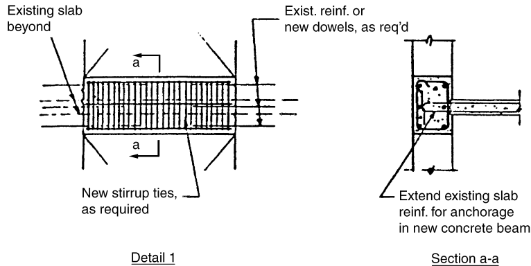
Figure 6.13. Strengthening of existing connecting beams in reinforced concrete walls.
