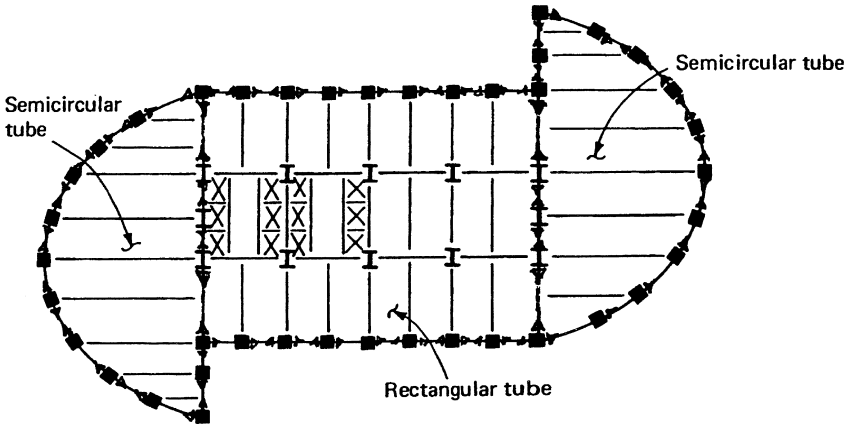
Figure 3.38A. Bundled tube, schematic plan.
