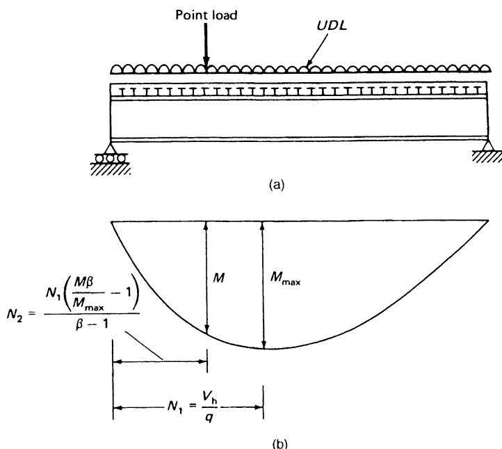
Figure 7.56. Shear connector requirements for composite beams subjected to concentrated loads: (a) schematic loading diagram; (b) shear connector requirements; (c) composite beam design example; (1) plan; (2) section.
