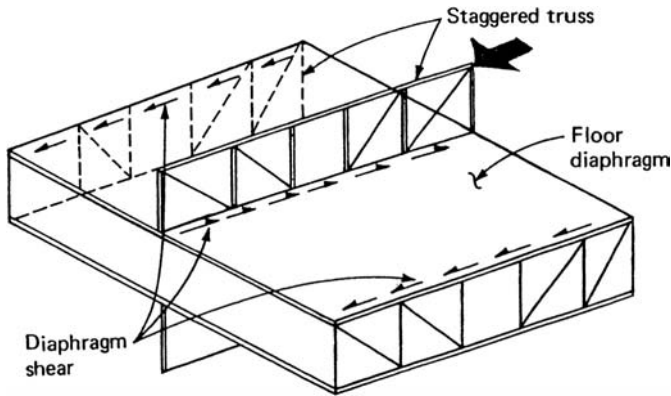
Figure 3.12. Load path in staggered truss system.
