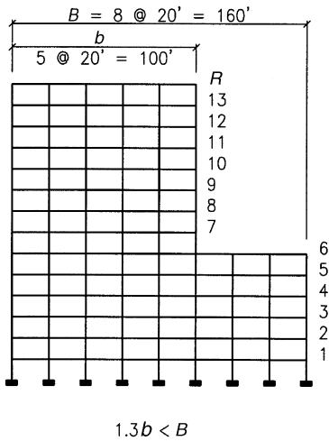
Figure 2.28. Vertical geometric irregularity. Vertical geometric irregularity exists if the horizontal dimension of the lateral-force-resisting system is more than 130% of that in the adjacent story: 1.3b < B . For example, the width of frame at level 6 = 160 ft, the width of frame at level 7 = 100 ft. 160 \text{ ft} > 1.3 \times 100 . Therefore, vertical geometric irregularity exists.
