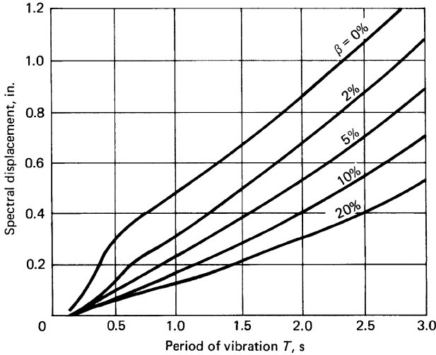
Figure 2.21. Smoothed displacement spectra for El Centro earthquake.
