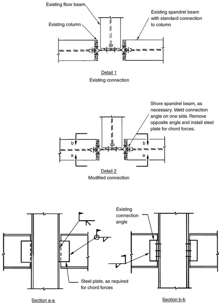
Figure 6.4. Modification of existing steel framing for diaphragm chord forces.
