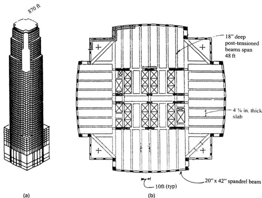
Figure 8.22. NCNB Tower, North Carolina: (a) schematic elevation; (b) typical floor framing plan.
