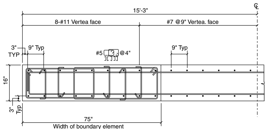
Figure 4.44. Shear wall example; schematic reinforcement.
