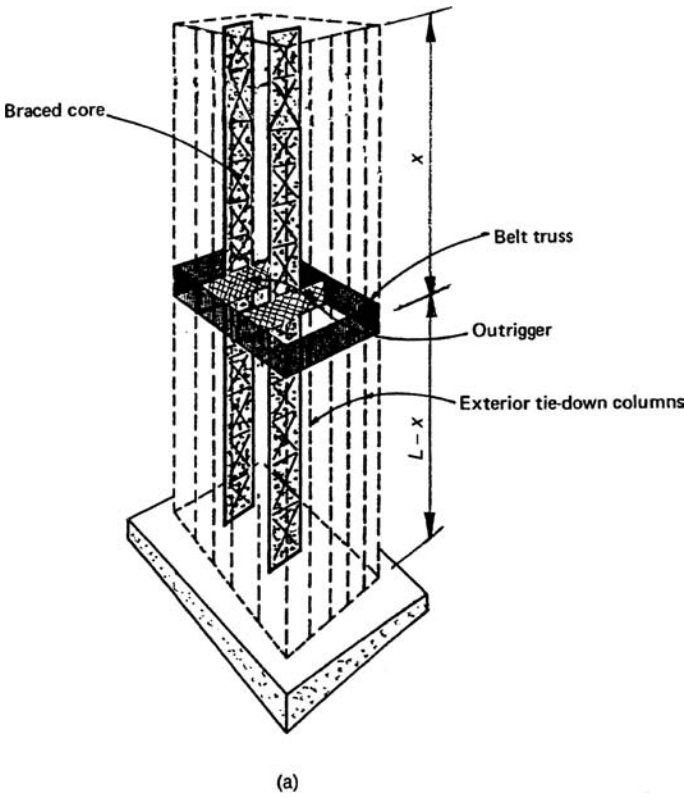
Figure 3.23a. Single outrigger and belt truss schematic elevation.
