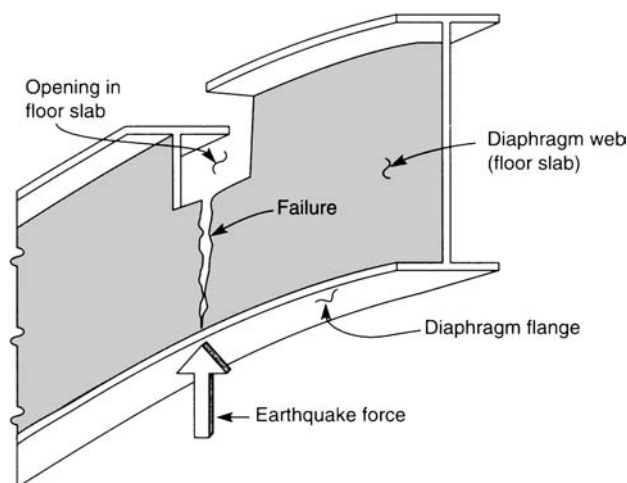
Figure 2.8. Diaphragm web failure due to large opening.
