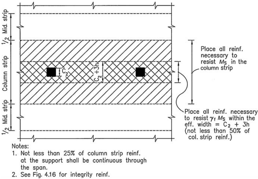
Figure 4.23. Seismic detailing requirements for two-way slabs in areas of moderate seismic risk; flat slab–beams not permitted in UBC zones 3 and 4, or for buildings assigned to SDC C, D, E, or F.
