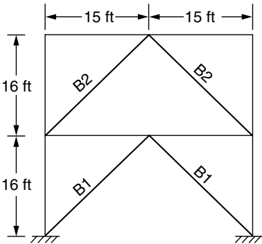
Figure 3.40c. Ordinary concentric brace frame (OCBF) example.
