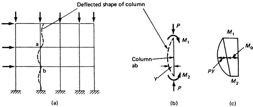
Figure 7.8. Behavior of building column: (a) building frame showing deflected shape of column; (b) column subjected to the simultaneous action of axial loads and moments; (c) moment diagram due to end moment and P\Delta effect.
