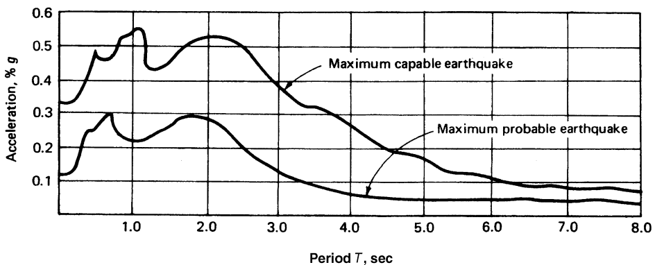
Figure 2.23. Unique site-specific design spectra.
