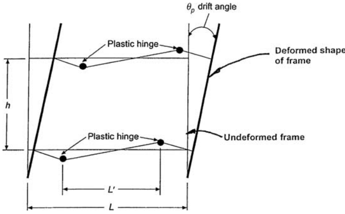
Figure 3.59. Inelastic drift of special moment frames with plastic hinges within beam span. A frame in which inelastic excursion occurs through the formation of plastic hinges within the beam span is capable of dissipating large amounts of energy. Such a behavior may be obtained by: 1) locally stiffening and strengthening fully restrained connections; or 2) locally reducing the beam section at desired locations.
