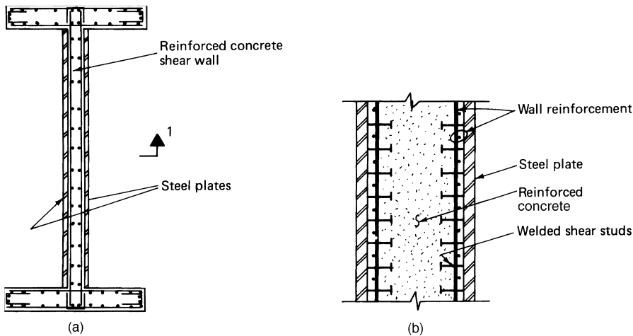
Figure 5.8. Composite shear walls with steel plates: (a) plan; (b) section.
