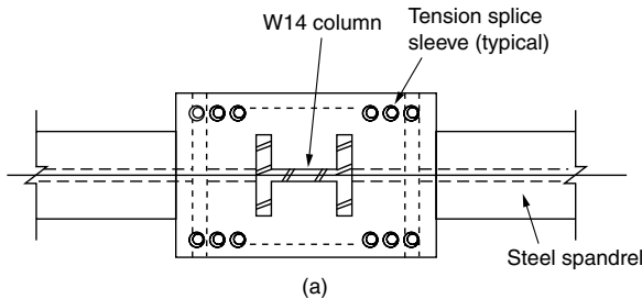
Figure 5.29. Composite column-to-steel column connection detail: (a) plan; (b) elevation; (c) section. America Tower, Houston, TX. Photograph of building under construction.
