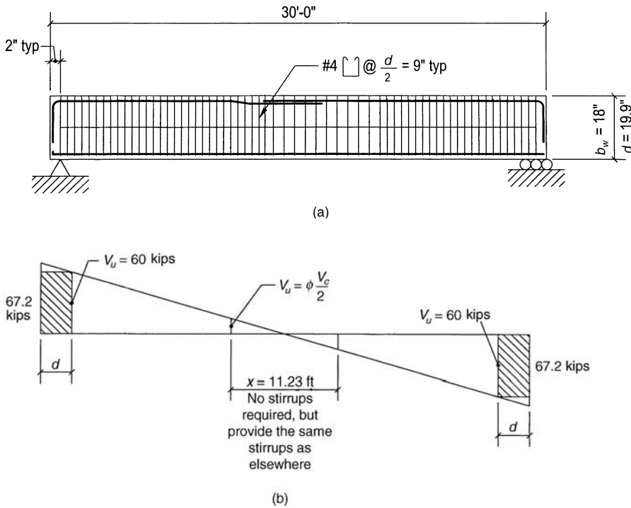
Figure 7.16. Schematic shear reinforcement.
