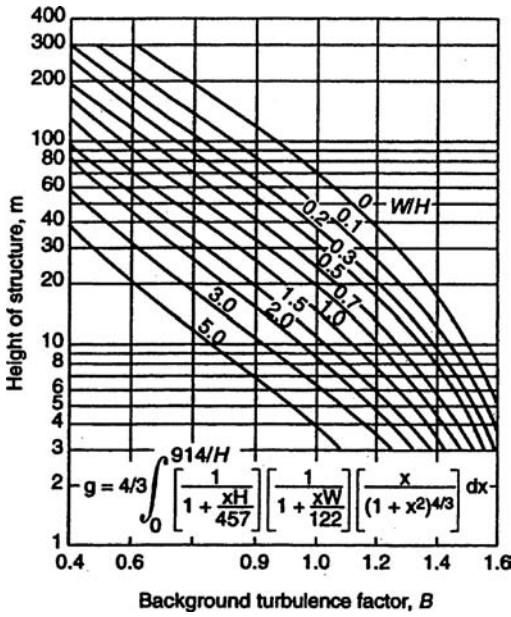
Figure 1.16. Background turbulence factor as a function of width and height of structure. (From NBCC 1995.)
