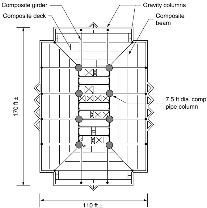
Figure 5.15. Pacific First Center; 44-story building.
