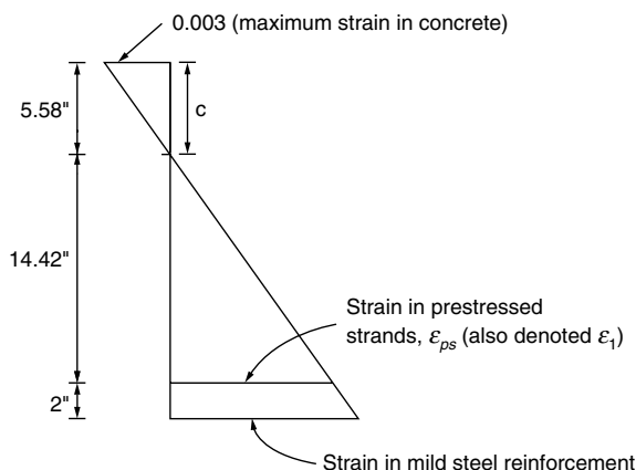
Figure 7.48b. Example 1: strain diagram, first trial.
