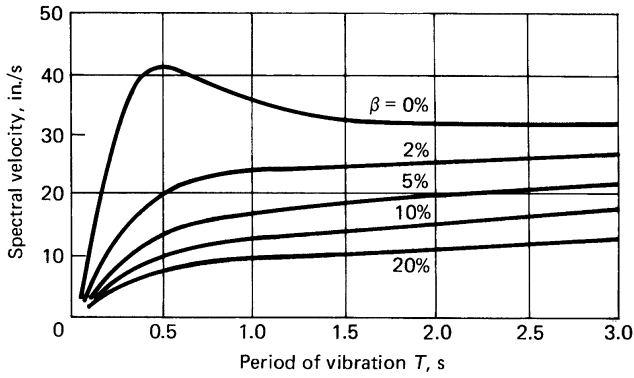
Figure 2.20. Smoothed velocity spectra for the El Centro earthquake.
