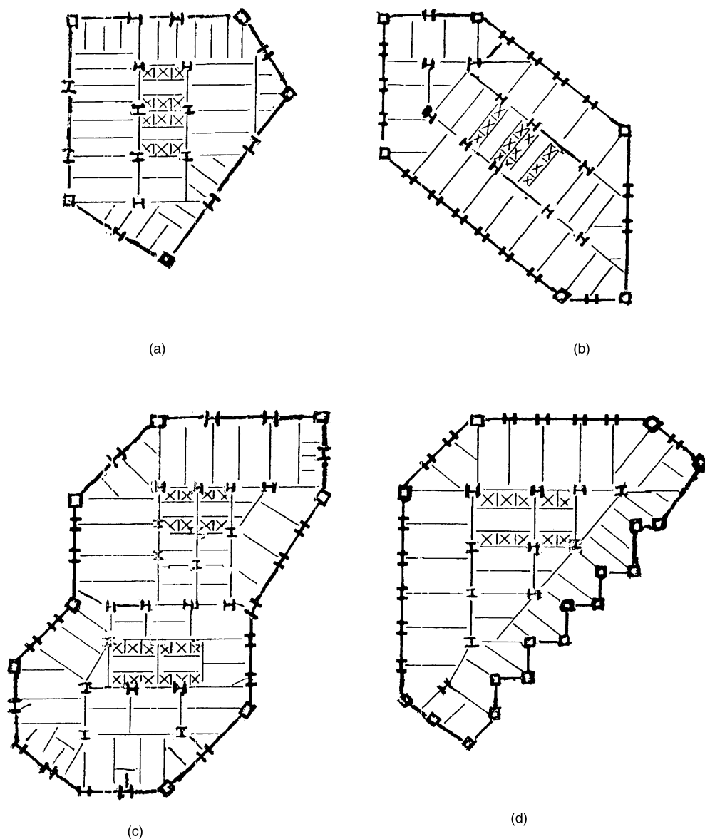
Figure 3.34. Free-form tubular configurations.
