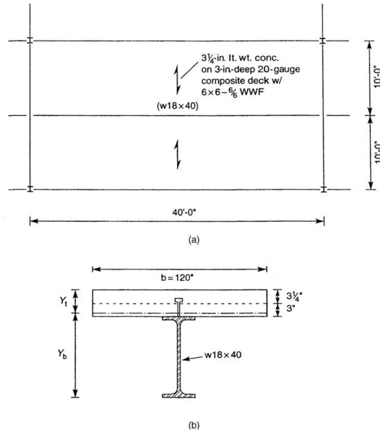
Figure 7.57. Composite beam, design example: (a) plan; (b) section.
