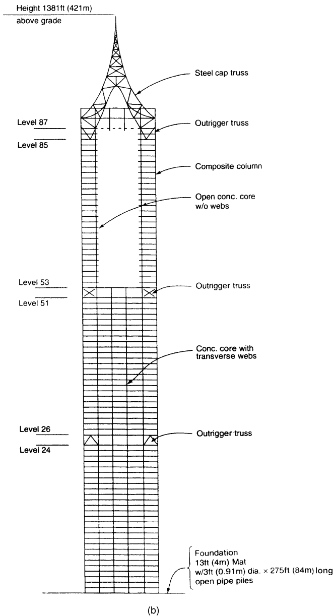
Figure 8.11. Jin Mao Tower, Shanghai, China: (b) structural system elevation.
