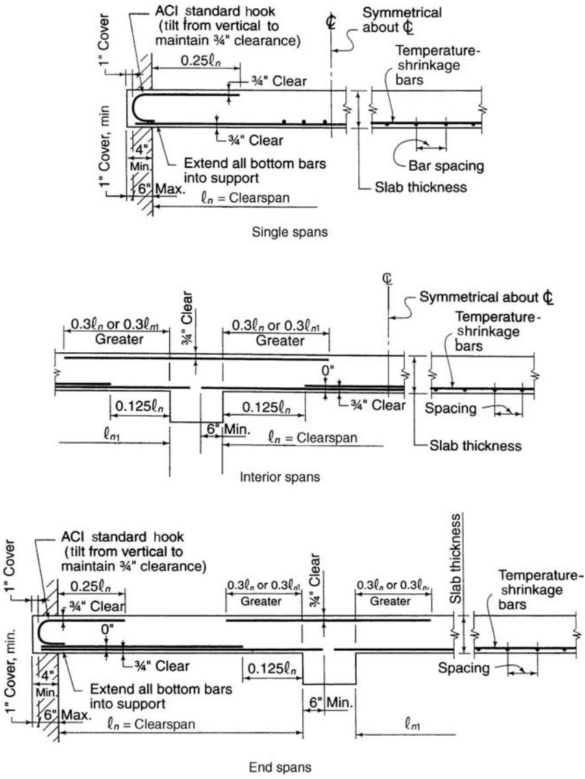
Figure 7.14. Recommended bar placement details, solid slabs. (Adapted from CRSI Design Handbook 2002.)
