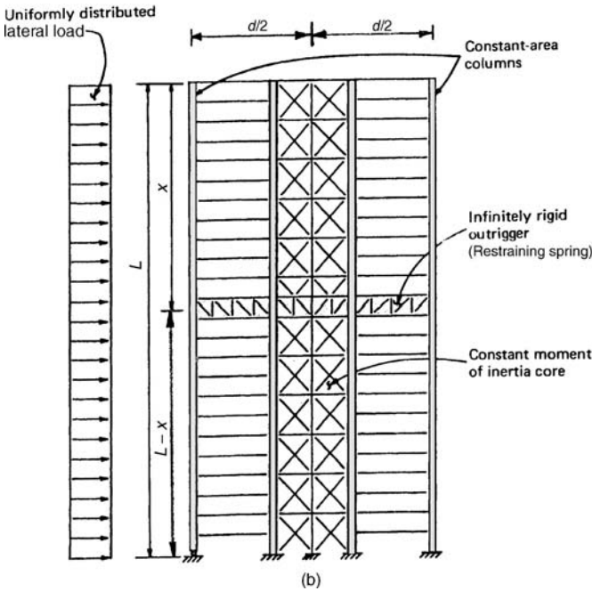
Figure 3.23b. Conceptual model for a single outrigger and belt truss model. Restraining “spring” occurs at a distance x from top.
