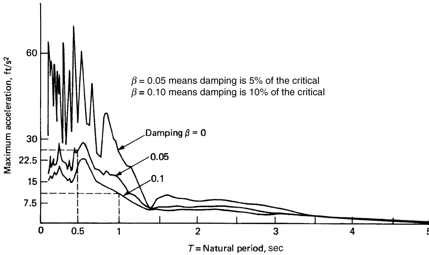
Figure 2.17. Acceleration spectrum: El Centro earthquake.
