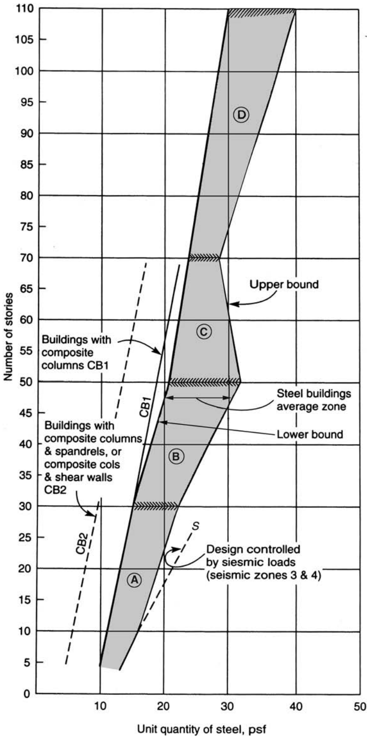
Figure 8.29. Structural steel unit quantities.
