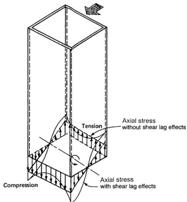
Figure 3.33. Axial stress distribution in square hollow tube with and without shear lag.
