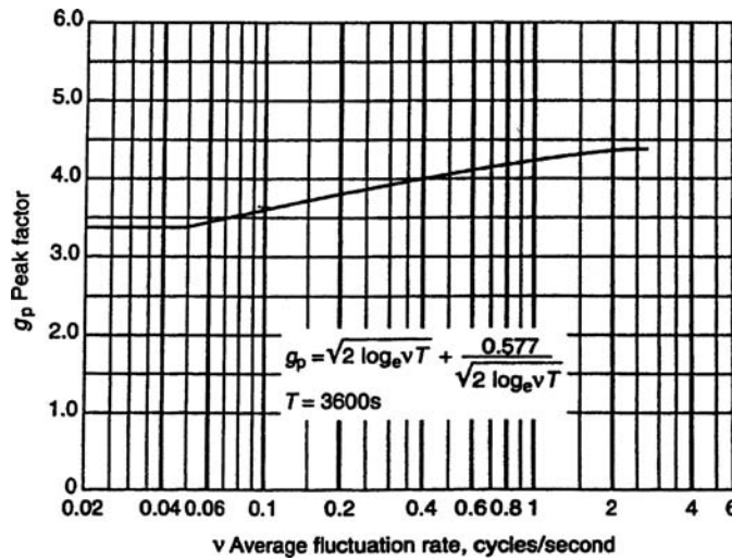
Figure 1.19. Peak factor g_p as a function of average fluctuation rate. (From NBCC 1995.)
