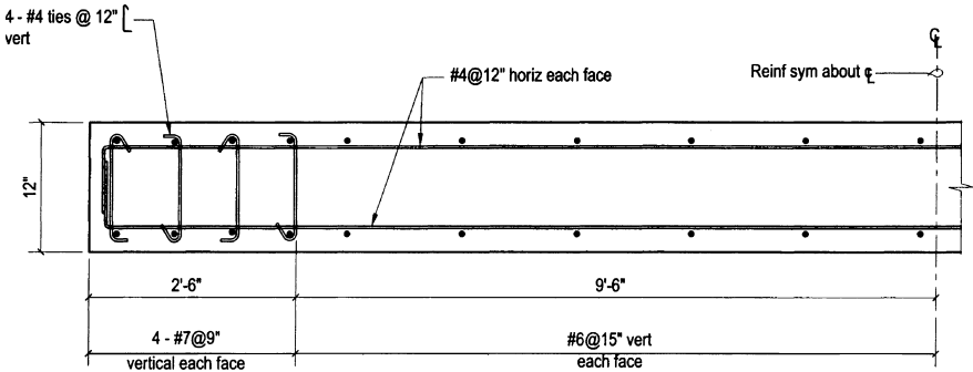
Figure 4.38. Shear wall; low to moderate seismic zones (SDC A, B, or C). Note: Vertical reinforcement of #7 @ 9" at each end is enclosed by lateral ties, since the reinforcement area of eight #7 vertical bars equal to 8 \times 0.6 = 4.8 \text{ in.}^2 is greater than 0.01 times the area of concrete = 12 \times 30 = 360 \text{ in.}^2 (See ACI 318-02 Sect. 14.3.6.)
