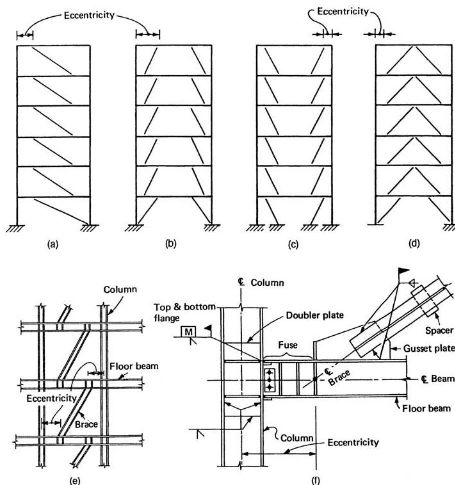
Figure 3.14. Eccentric bracing system: (a–d) common types of bracing; (e) elevation; (f) detail.
