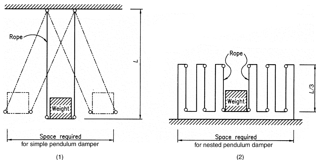
Figure 8.30j. (1) Simple pendulum damper; (2) nested pendulum damper.
