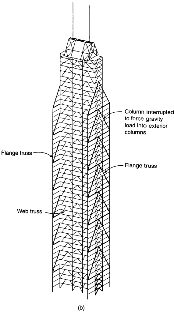
Figure 8.5. Bank One Center, Indianapolis: (a) plan; (b) lateral system.
