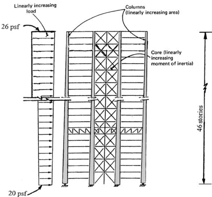
Figure 3.25. Single-outrigger building, schematic structural system.
