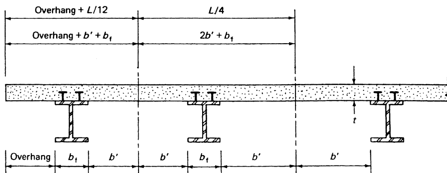
Figure 7.54. Effective width concept as defined in the AISC specifications.
