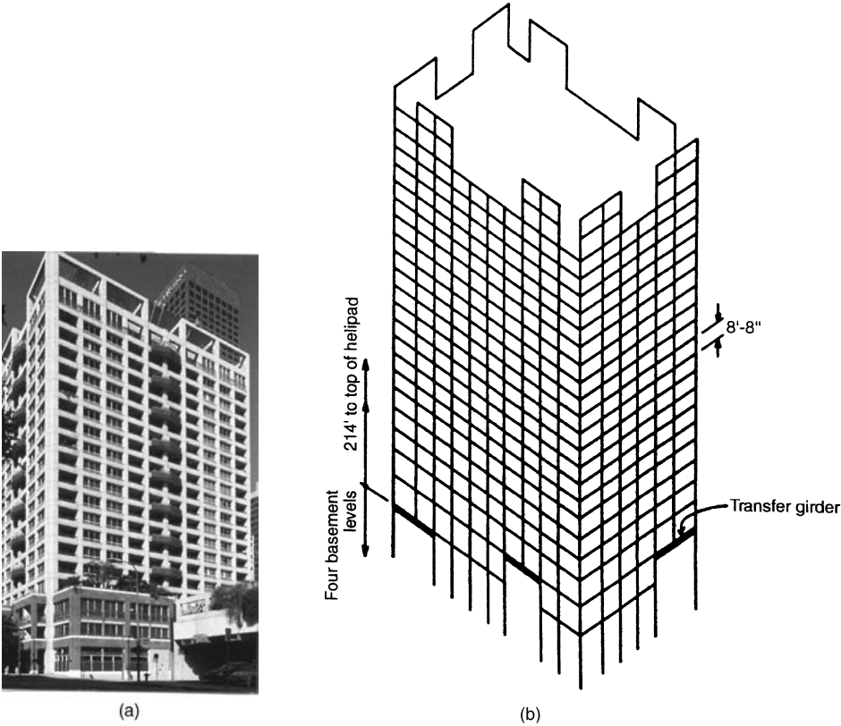
Figure 8.23. Museum Tower, Los Angeles: (a) building elevation; (b) lateral bracing system; (c) typical floor framing plan. Structural engineers: John A. Martin & Associates, Inc., Los Angeles.
