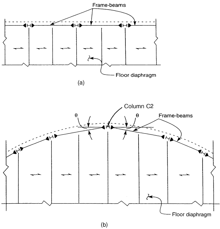
Figure 7.6. Beam framing conditions for evaluation of effective length factor, K : (a) beam framing into columns without skew; (b) skewed beamed framing into columns.
