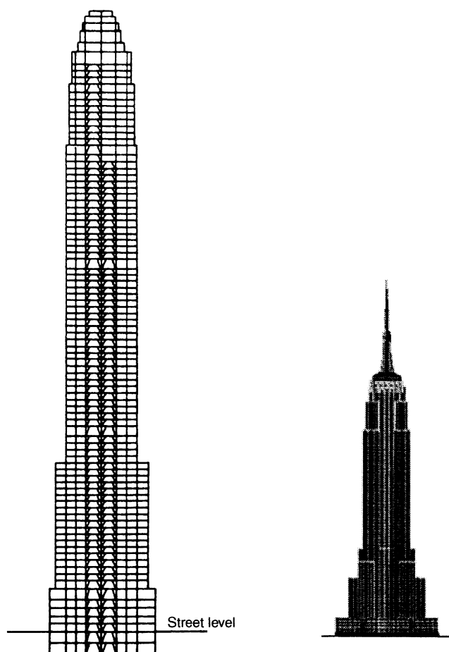
Figure 8.4. Empire State Building bracing system; riveted structural steel frame encased in cinder concrete.
