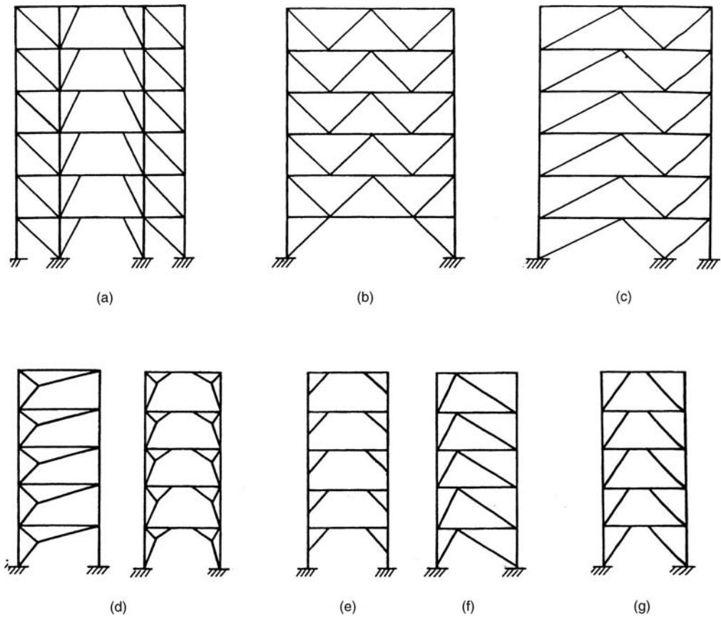
Figure 3.9a–g. Brace configurations that allow for door-size openings in interior space layouts. Note: Some configurations are not permitted in areas of high seismicity.
