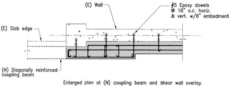
Figure 6.12b. Enlarged plan at (N) coupling beam and shear wall overlay.
