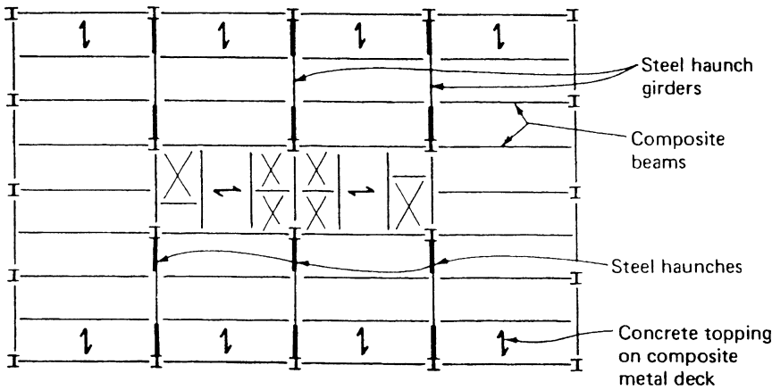
Figure 7.58. Schematic floor plan showing haunch girders.
