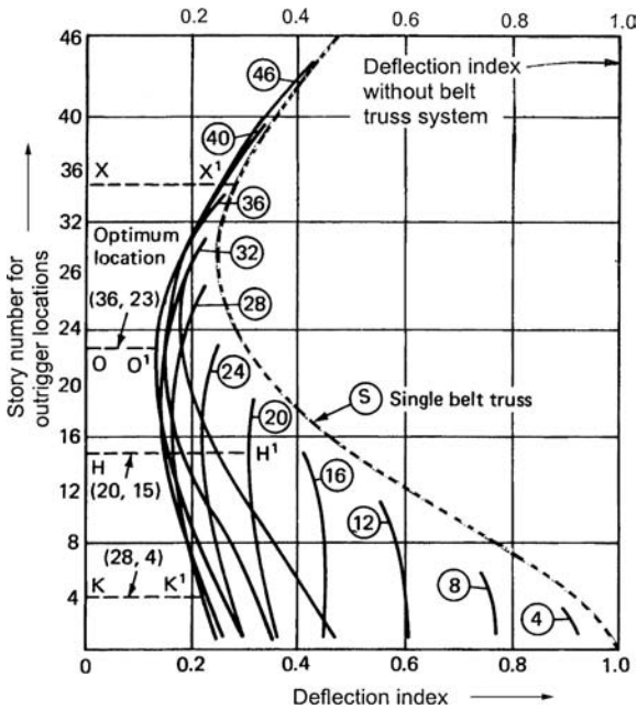
Figure 3.29. Deflection index versus level of outrigger locations.
