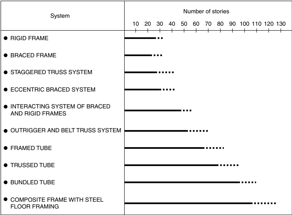
Figure 3.1. Height comparison of steel building systems.
