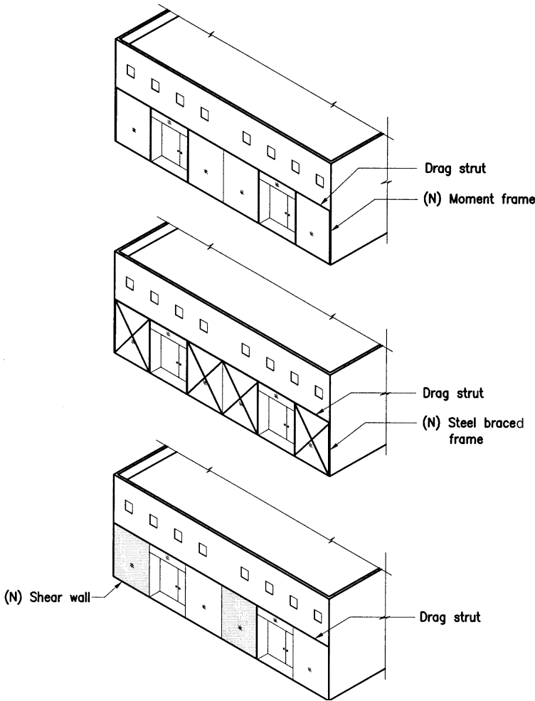
Figure 6.10. Common methods for upgrading buildings with open storefronts.
