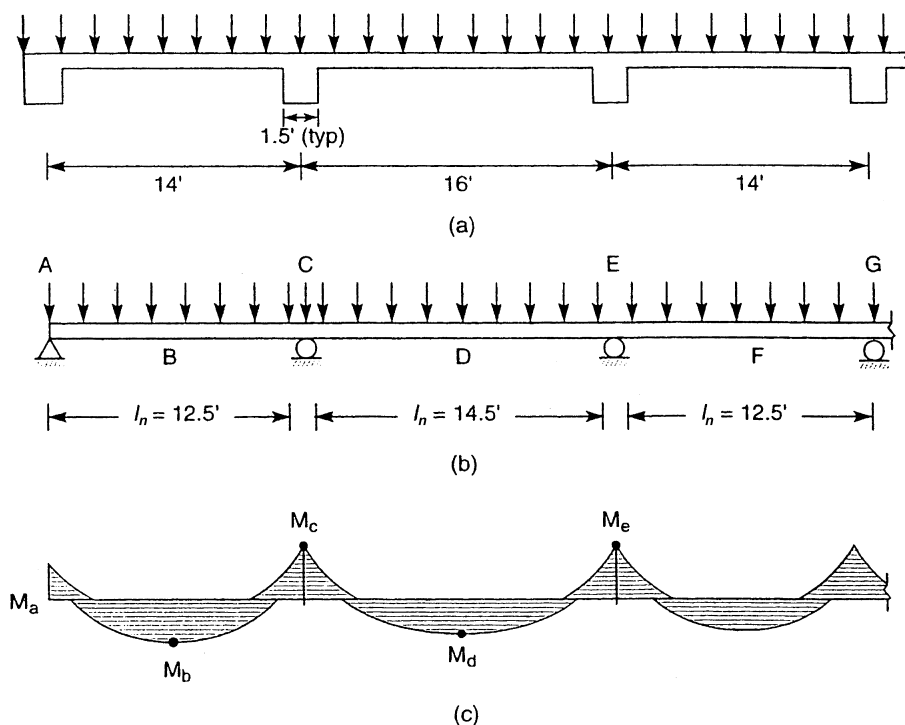
Figure 7.10. One-way slab example: (a) typical 1-ft strip; (b) slab modelled as a continuous beam; (c) design moments.
