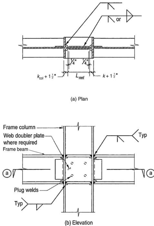
Figure 3.61. Typical continuity plates and doubler plates.
