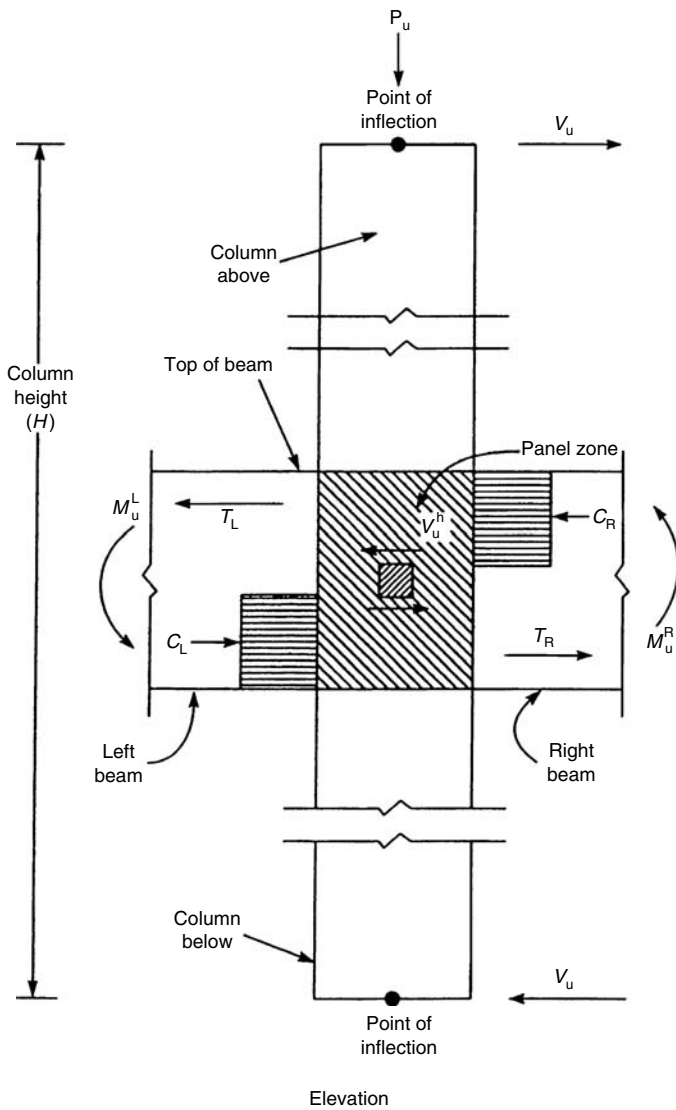
Figure 4.40a. Column panel shear forces.
