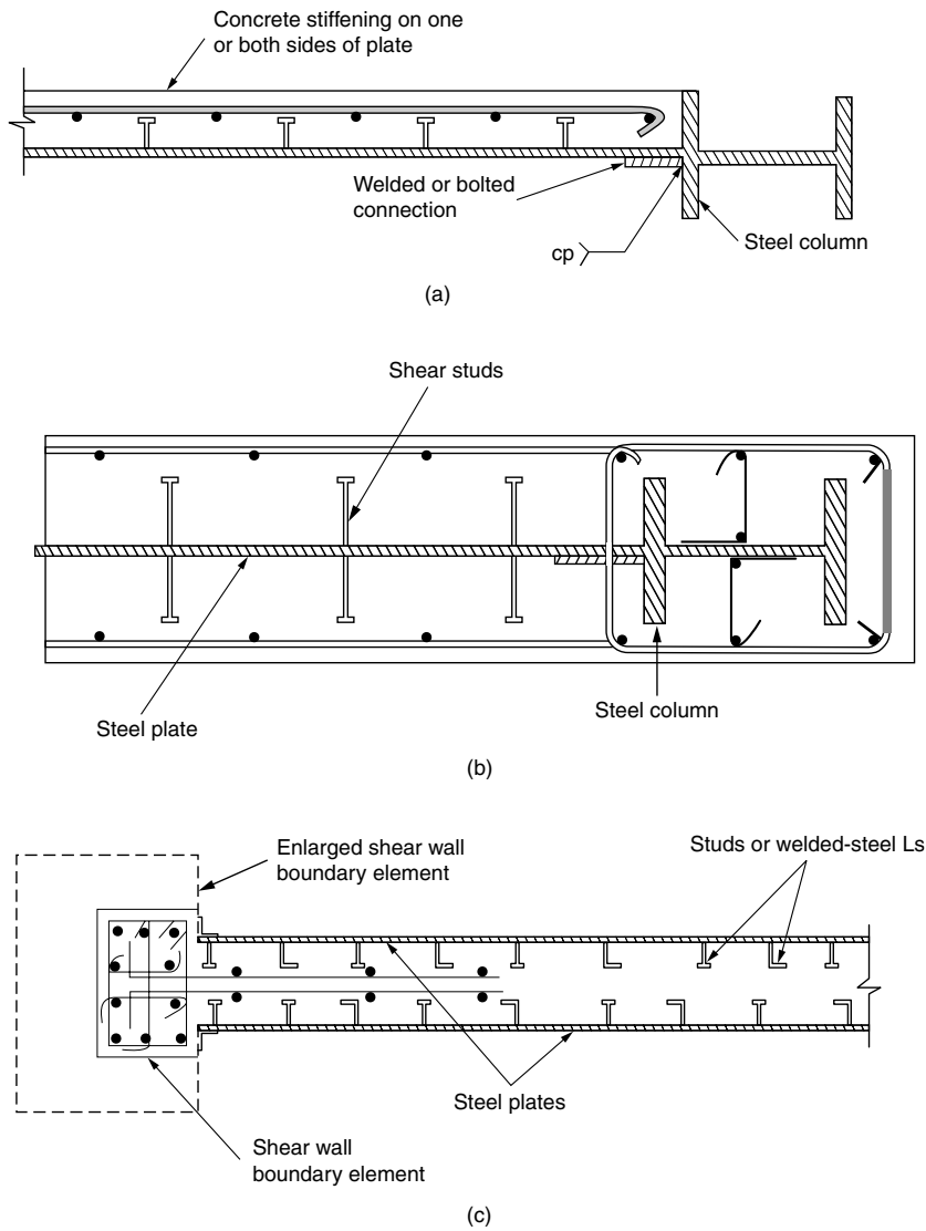
Figure 5.38. Composite steel plate shear walls.
