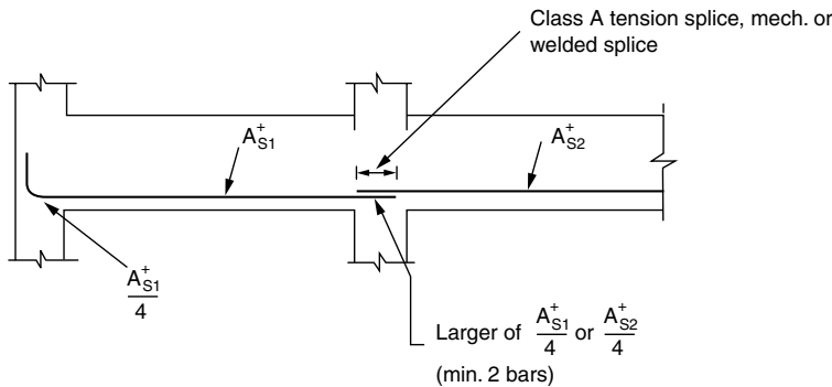
Figure 4.19. Integrity reinforcement in beams other than perimeter beams.
