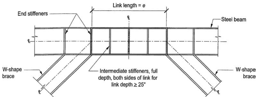
Figure 3.53. An EBF with W-shape bracing; stiffener requirements.
