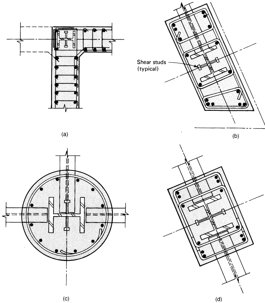
Figure 5.24. Composite vertical elements: (a) composite shear wall; (b) composite corner column; (c) typical circular column on long faces; (d) typical exterior column on short faces.
