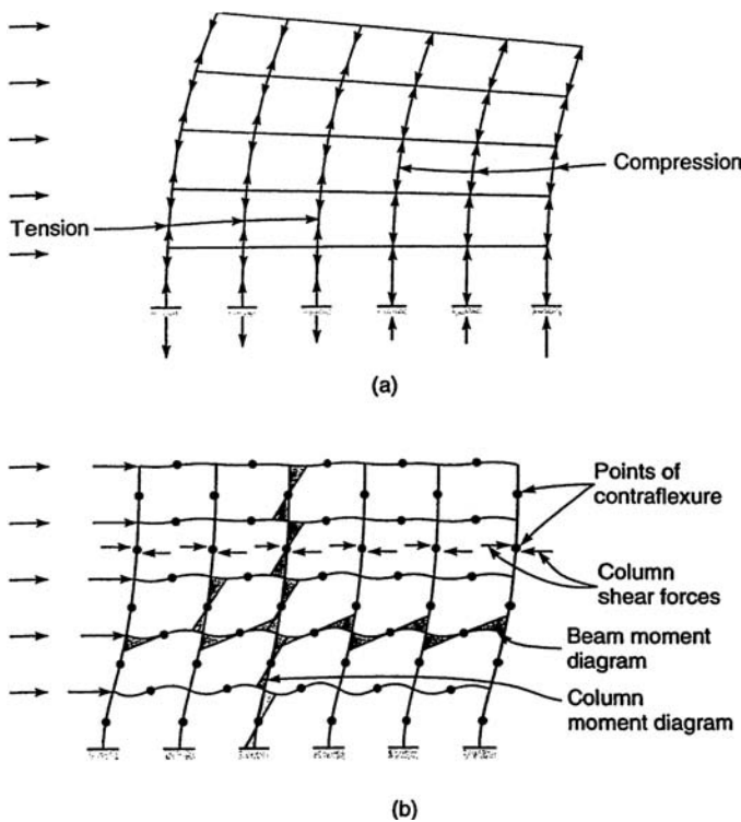
Figure 3.4. Rigid frame deflections: (a) forces and deformations caused by external overturning moment; (b) forces and deformations caused by external shear.
