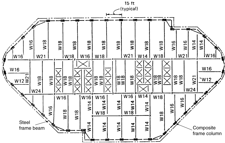
Figure 5.27. Structural floor framing plan; 42-story America Tower, Houston, TX.
