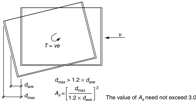
Figure 2.31. Torsional irregularity. Torsional irregularity exists when d_{\max} , the maximum story drift at a corner including accidental torsion, is more than 1.2 times the average of the drifts at the corresponding corners.
