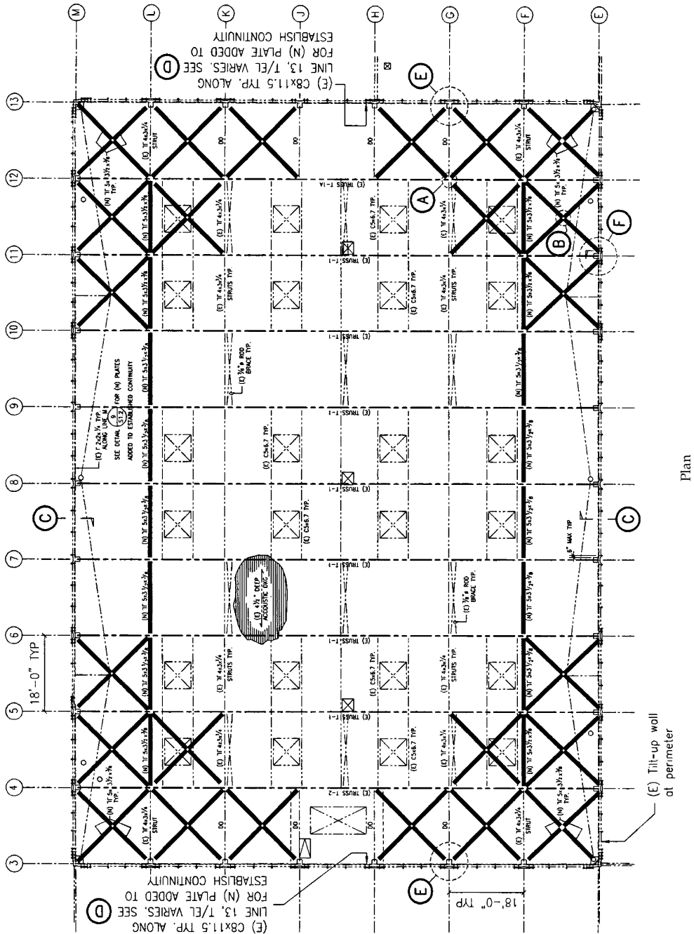
Figure 6.9. Diaphragm strengthening of an existing gymnasium roof with horizontal bracing.
