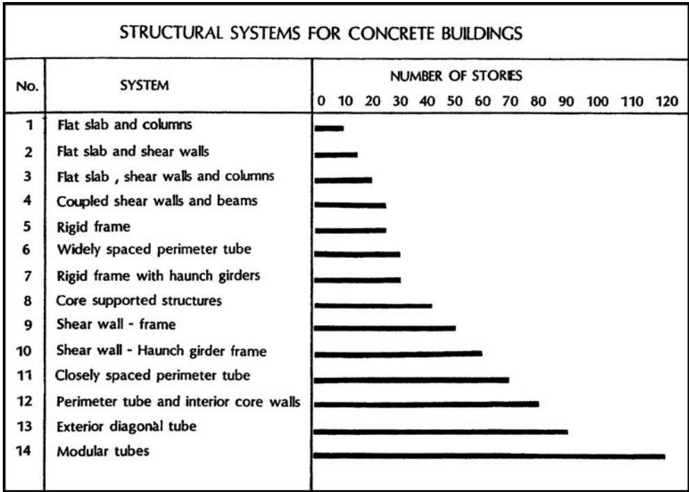
Figure 4.1. Structural systems for concrete buildings.
