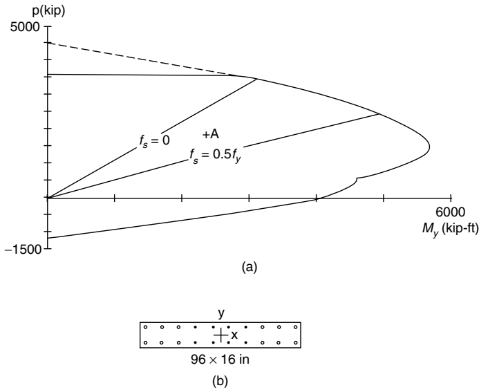
Figure 4.51. (a) Wall-pier W1 interaction diagram; (b) cross section of wall pier W1.
