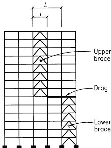
Figure 2.29. In-plane discontinuity; type-4 irregularity. A type 4-irregularity exists when there is an in-plane offset of the lateral system greater than the width of the system.
