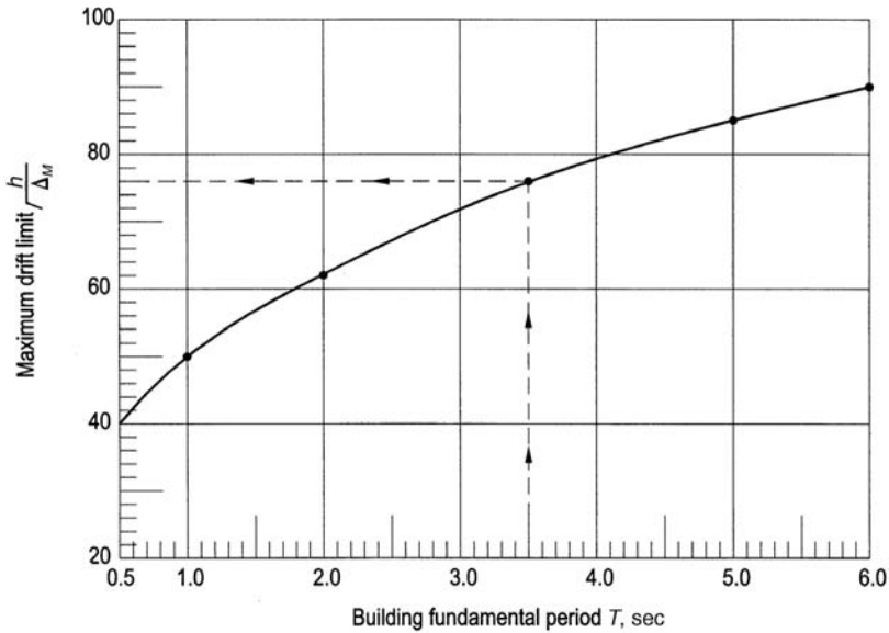
Figure 2.42a. Permissible drift ratio h/\Delta_M versus building fundamental period T . (LARUCP 2004.)
