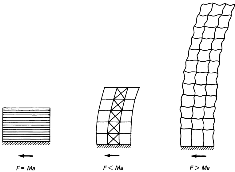
Figure 2.2. Schematic representation of seismic forces.
