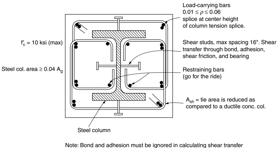
Figure 5.1. Concrete-encased composite column; design considerations.
