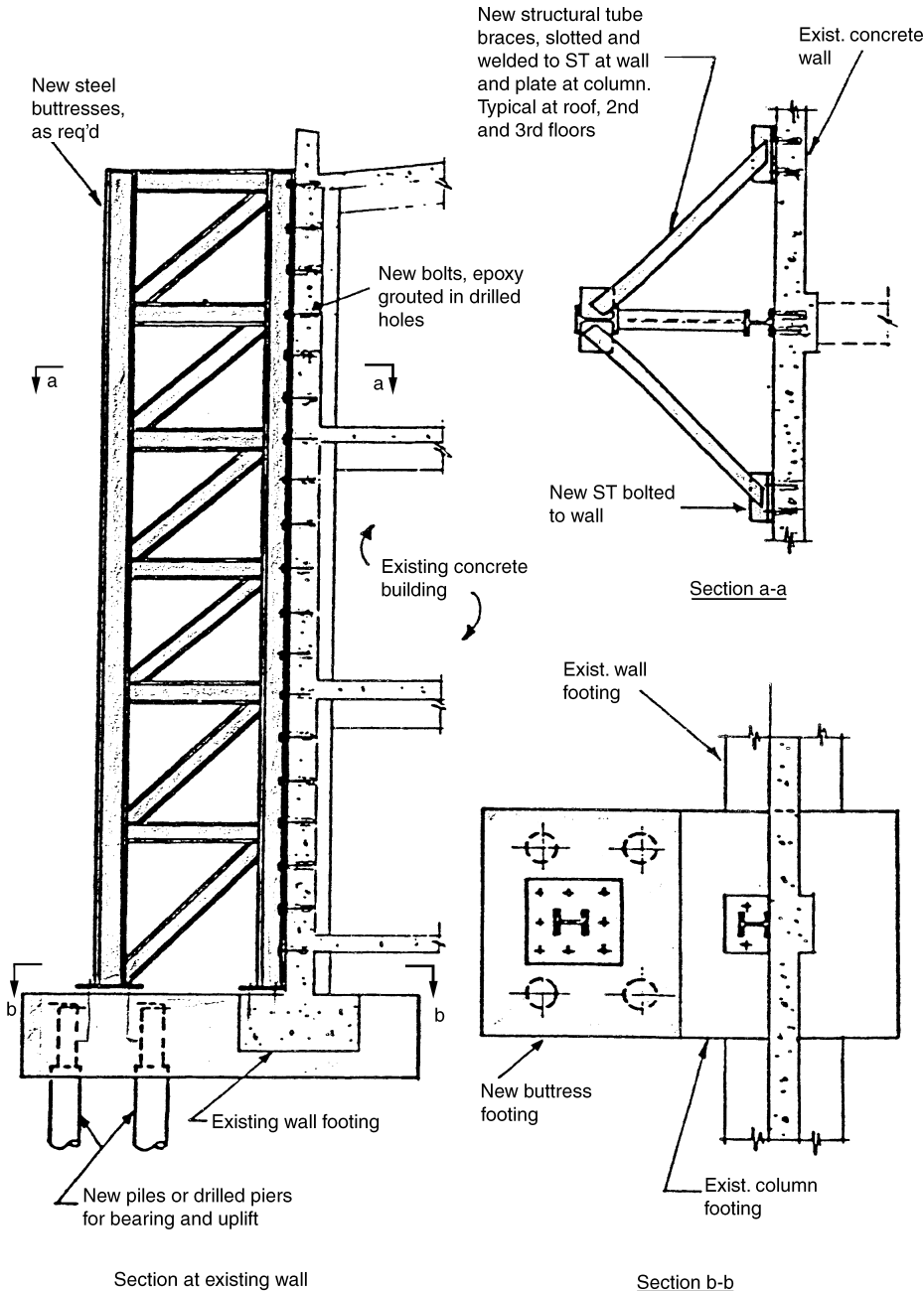
Figure 6.19. Braced structural steel buttresses to strengthen an existing reinforced concrete building.
