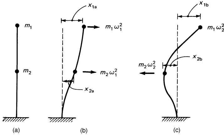
Figure 2.70. Two-story lumped-mass system illustrating Betti's reciprocal theorem: (a) lumped model; (b) forces acting during first mode of vibration; (c) forces acting during second mode of vibration.
