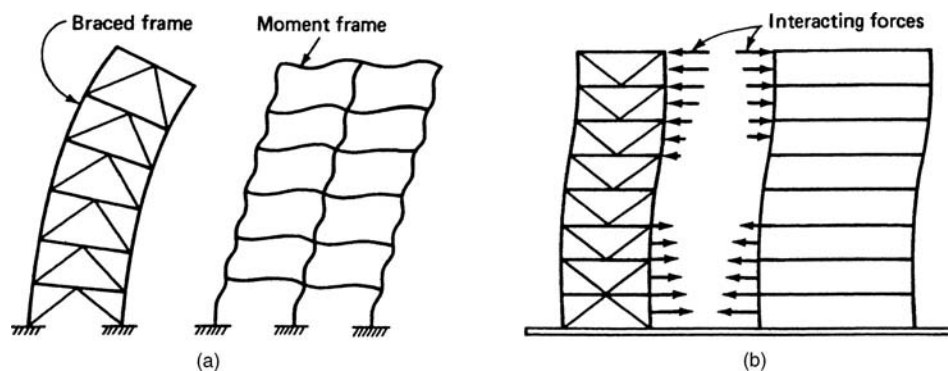
Figure 3.16. Interaction between braced and unbraced frames: (a) characteristic deformation shapes; (b) variation of shear forces resulting from interaction.
