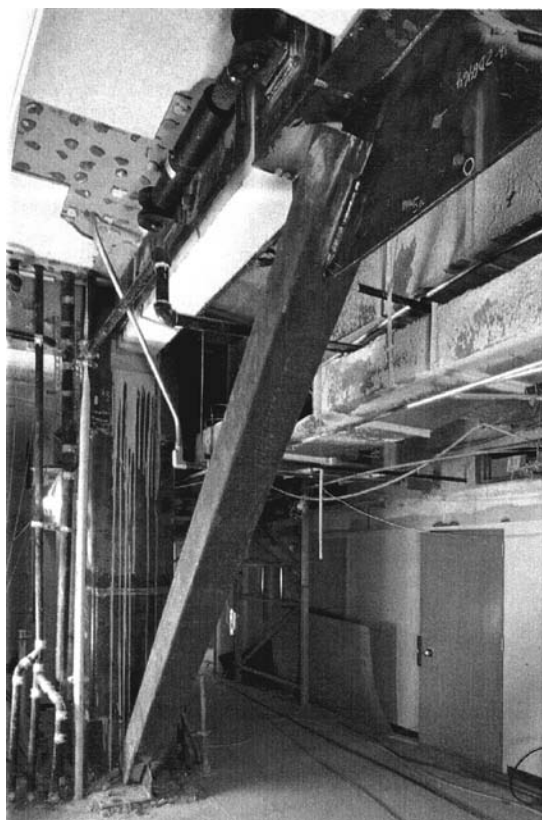
Figure 8.35c. Fluid viscous damper installed in an existing building.
