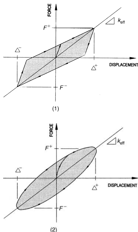
Figure 8.34m. Idealized force-displacement relationships for base-isolation systems: (1) hysteretic system; (2) viscous system. In seismic isolation, hysteretic behavior is a term that describes intrinsic damping due to inelastic deformation of base isolators. Energy is dissipated through work done by the inelastic actions in the isolators. Viscoelastic or viscous behavior, on the other hand, typifies damping action of external devices that use viscous liquids to absorb energy. No inelastic deformations are involved: Energy is dissipated as heat. Effective stiffness k_{\text{eff}} of an isolator is calculated from test data by measuring forces F^+ and F^- , and corresponding deformations \Delta^+ and \Delta^- . The area enclosed by the force-displacement loop is used to calculate effective damping \beta_{\text{eff}} .
