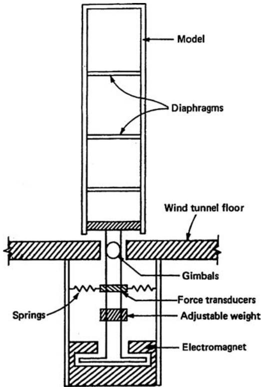
Figure 1.22. Rigid aeroelastic model with gimbal.
