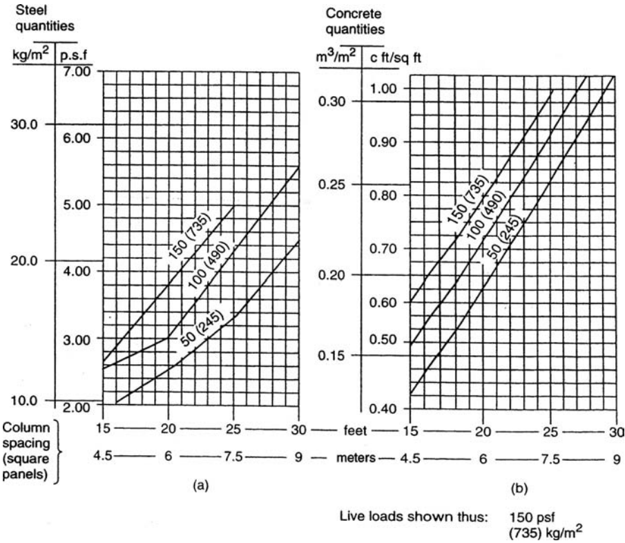
Figure 7.24. Flat plate, unit quantities: (a) reinforcement; (b) concrete.
