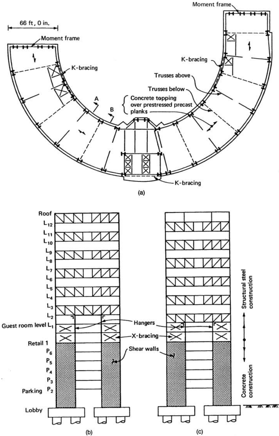
Figure 3.11. Staggered truss system for a semicircular building: (a) plan; (b) section A; (c) section B.
