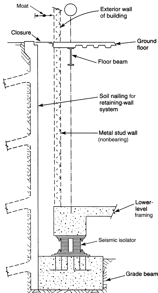
Figure 8.34c. Moat around base-isolated building.
