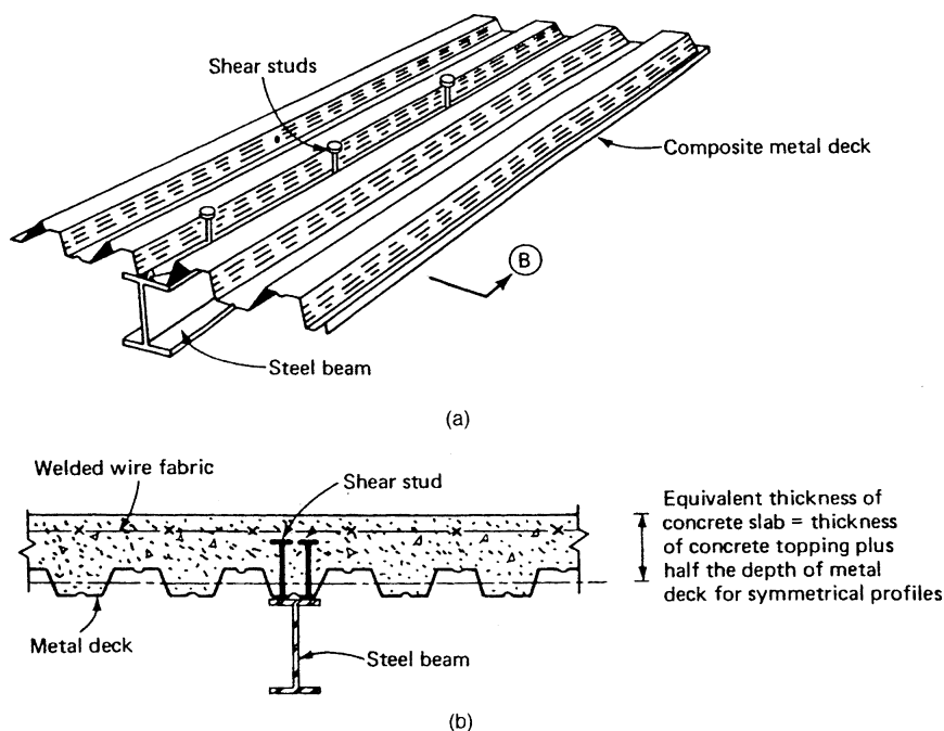
Figure 7.52. Composite beam with deck parallel to beam: (a) schematic view; (b) section B showing equivalent thickness of slab.
