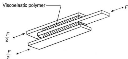
Figure 8.30a. Viscoelastic polymer damper. A building damping of about 4% can be attained using these dampers. Buildings equipped with viscoelastic dampers include the World Trade Center, New York, destroyed on Sept 11, 2001, and the Columbia Seafirst Center, Seattle.
