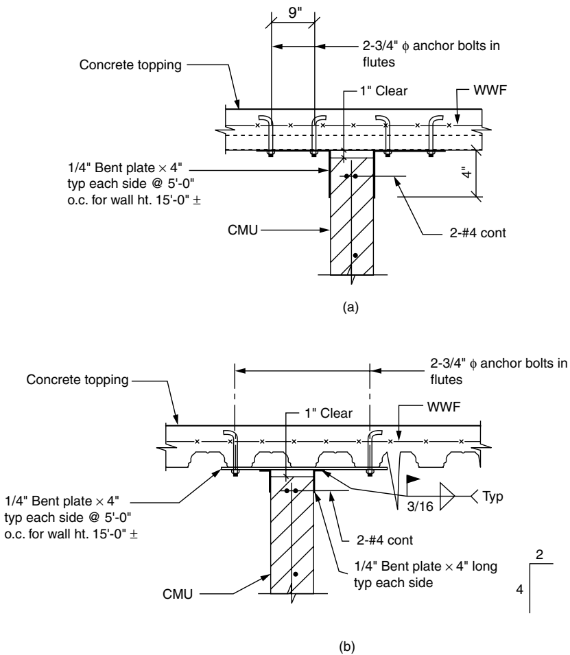
Figure 2.62. Slip joint in nonstructural masonry partition; connection at top provides out-of-plane support without restricting in-plane movement of wall. (a) Wall perpendicular to metal deck span; (b) wall parallel to metal deck span.
