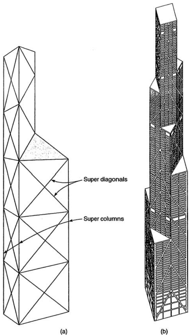
Figure 3.36. (a) Tube building with multistory diagonal bracing; (b) rotated square tube with super diagonals. (Adapted from an article by Mahjoub Elnimeiri, published in Civil Engineering Journal .)
