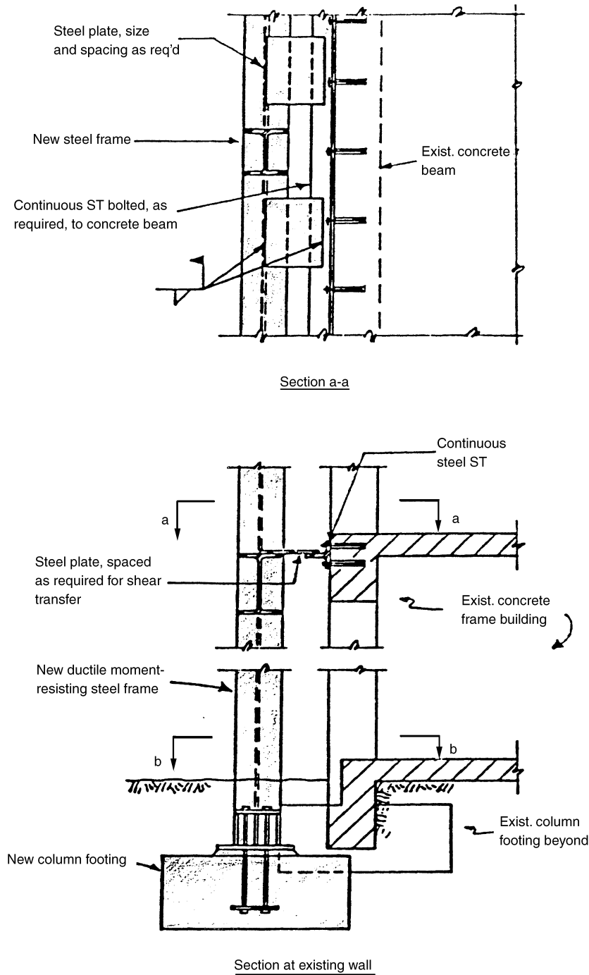
Figure 6.25. Upgrading an existing building with external frames.
