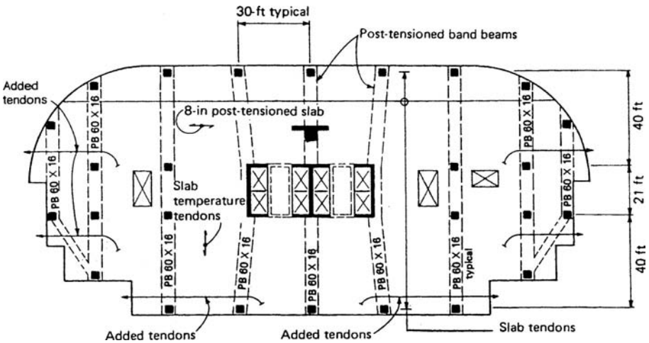
Figure 7.27. Typical floor plan of one-way post-tensioned slab system.
