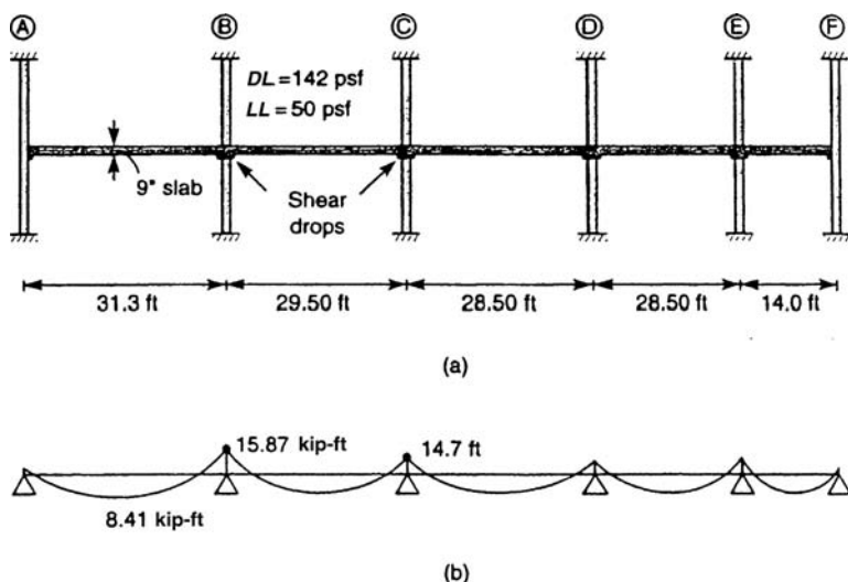
Figure 7.44. Example 3: flat plate: (a) span and loading; (b) elastic moments due to dead load plus live load.
