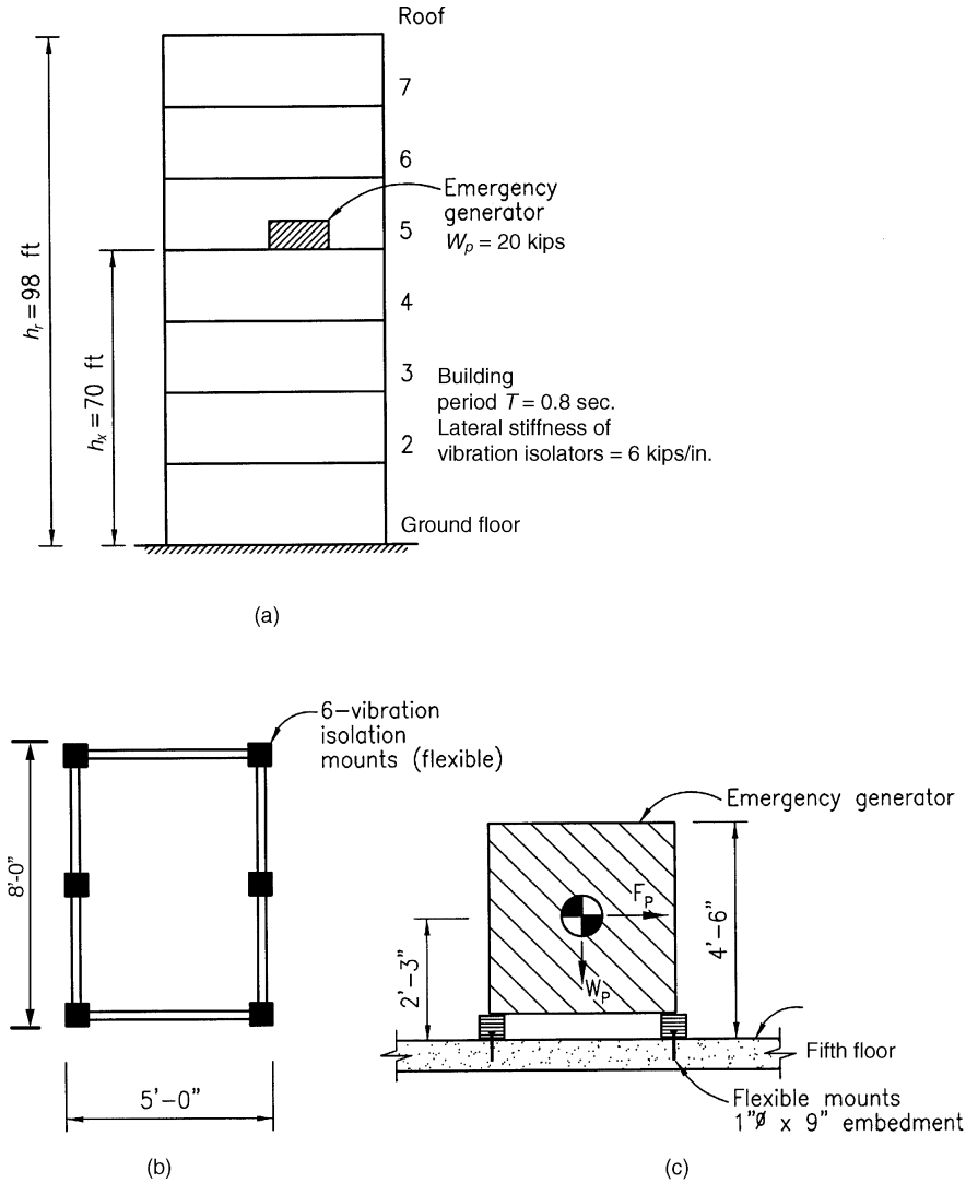
Figure 2.64. Example 2: Emergency generator: (a) building elevation; (b) equipment plan dimensions; (c) equipment elevation.
