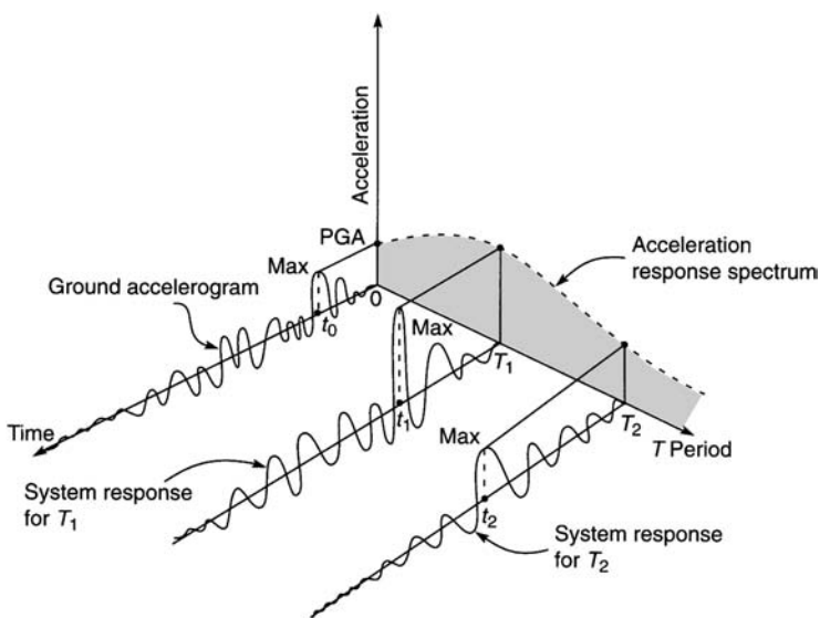
Figure 2.15. Graphical description of response spectrum.
