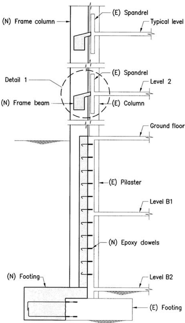
Figure 6.12c. Section through longitudinal frame.
