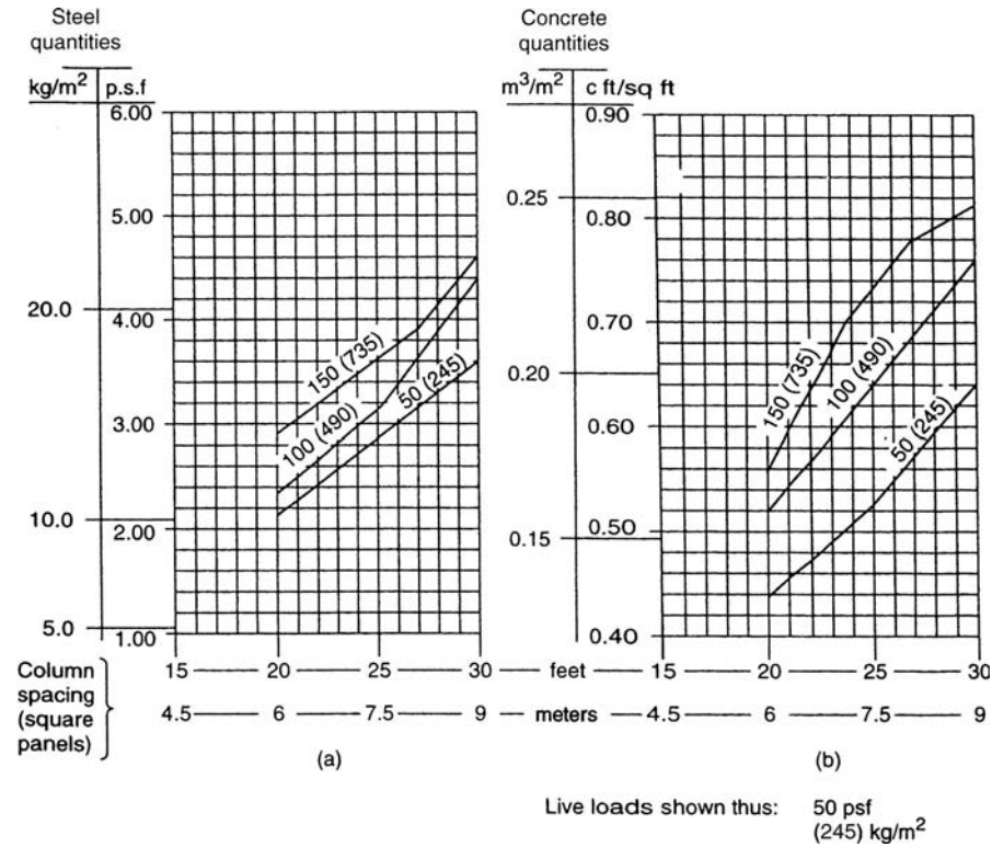
Figure 7.23. Waffle slab, unit quantities: (a) reinforcement; (b) concrete.
