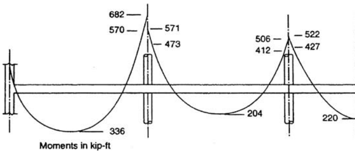
Figure 7.43. Example 2: post-tensioned continuous beam; service load moments.
