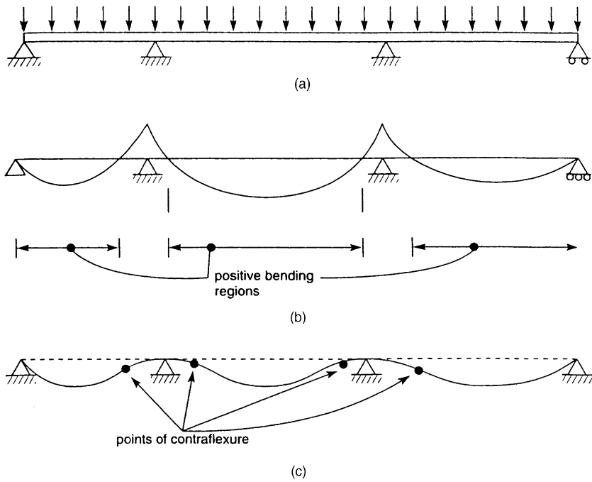
Figure 7.2. Lateral torsional buckling of beams: (a) continuous beam with uniformly distributed load; (b) bending moment diagram showing positive bending region; (c) points of contraflexure.
