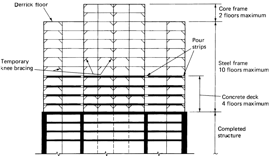
Figure 5.26. General construction sequence in composite structures.
