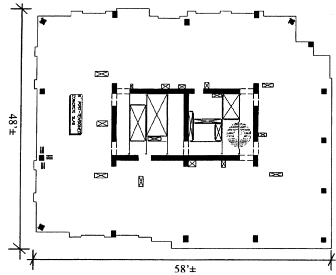
Figure 5.40. The Renaissance project, San Diego, CA; typical floor framing plan.
