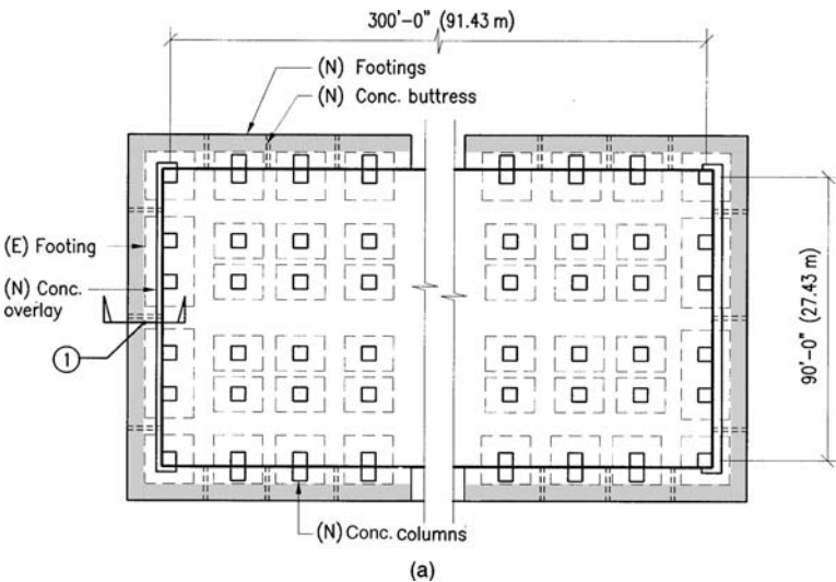
Figure 6.12. Seismic upgrade of a concrete hospital building with an external concrete moment frame. Modifications are restricted to the periphery of the building to keep the building operational with minimal interference to its functionality. (a) plan showing (N) foundations, (N) concrete overlay in the transverse direction, and (N) moment frames in the longitudinal direction.
