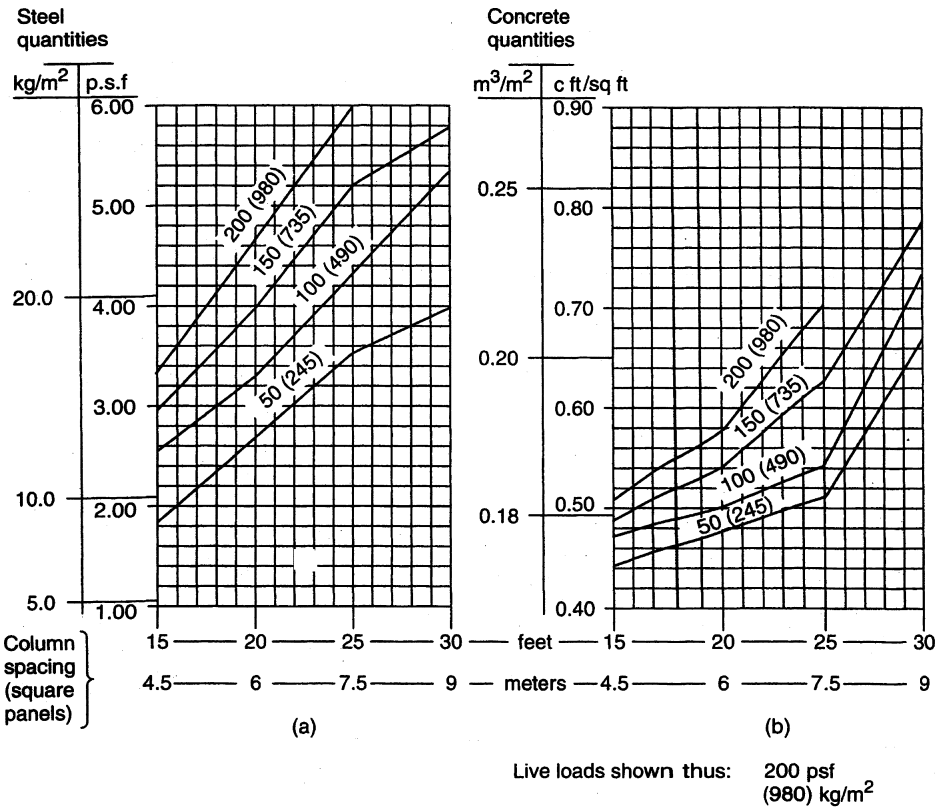
Figure 7.20. One-way solid slab, unit quantities: (a) reinforcement; (b) concrete.
