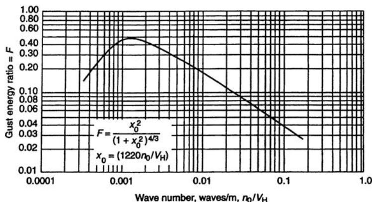
Figure 1.18. Gust energy ratio as a function of wave number. (From NBCC 1995).
