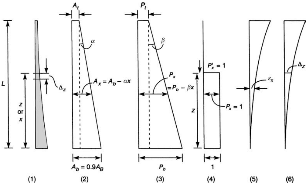
Figure 8.32f. Axial shortening of columns; closed-form solution: (1) axial shortening \Delta_z ; (2) column area; (3) column axial load; (4) unit load at height z ; (5) axial strain; (6) axial displacement.
