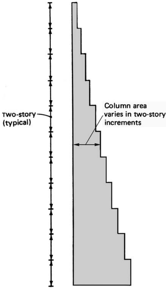
Figure 8.32c. Variation of cross-sectional area of a high-rise column.
