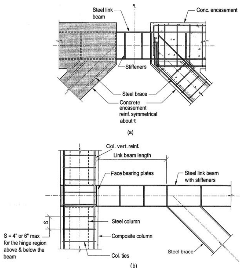
Figure 5.37. Schematic details of link beams: (a) link at center of beam; (b) link adjacent to column.
