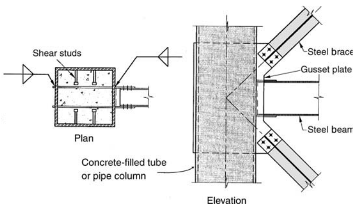
Figure 5.34. Concrete-filled composite column-to-steel concentric brace connection.
