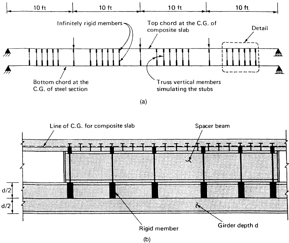
Figure 7.63. (a) Elevation of vierendeel truss analytical model; (b) partial detail of analytical model.
