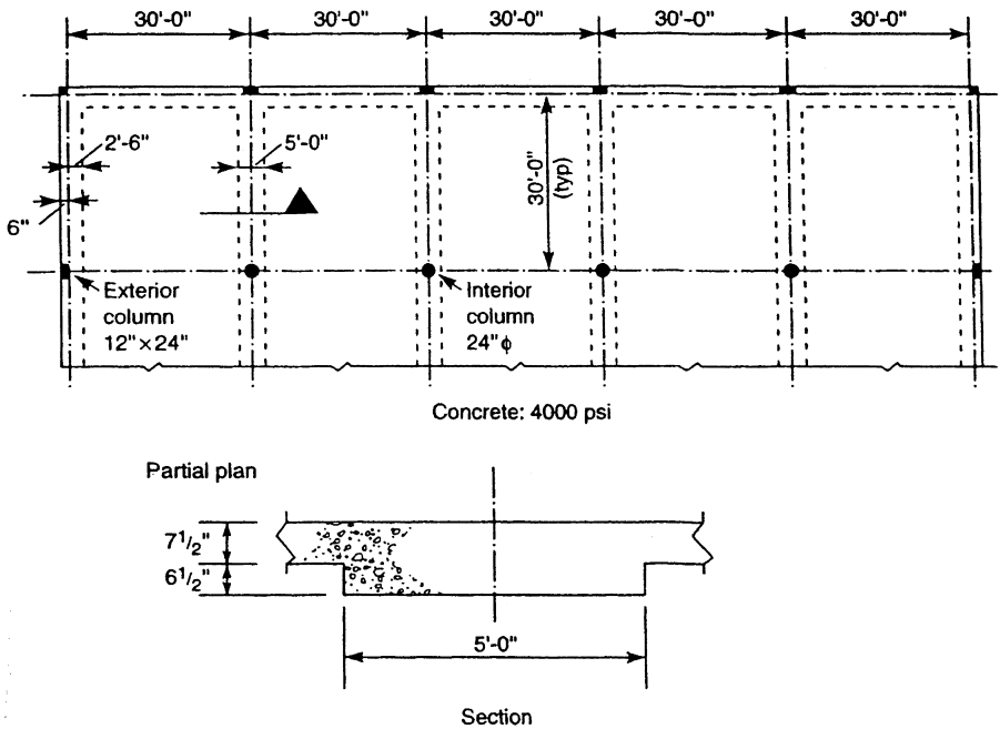
Figure 7.38. Example 1: one-way post-tensioned slab.
