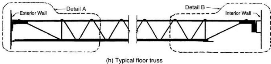
(h) Typical floor truss
