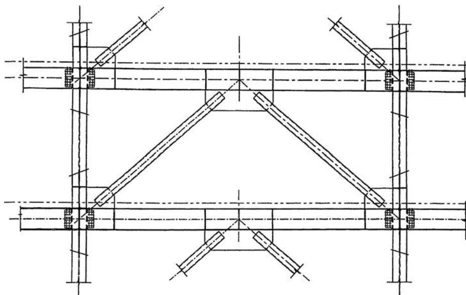
Figure 3.44. Schematic elevation of an OCBF showing gusset plates. (Courtesy of Louis Choi, S.E., John A. Martin & Associates Structural Engineers, Los Angeles, CA.)
