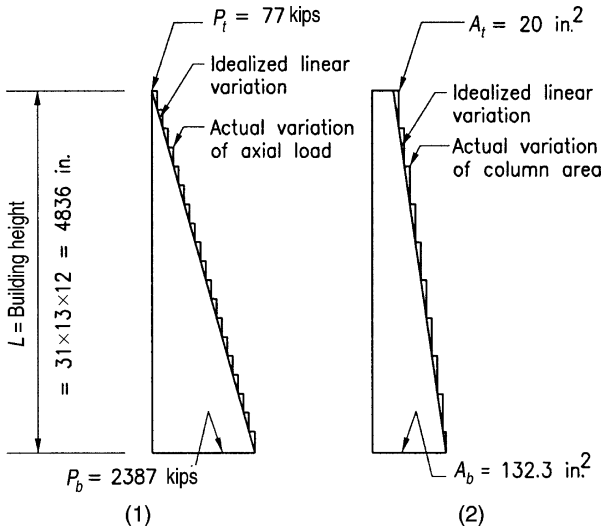
Figure 8.32i. Example 2, interior column G-6: (1) axial load variation; (2) variation of cross-sectional areas.
