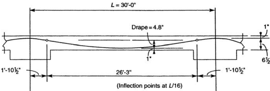
Figure 7.40. Example 1: one-way post-tensional slab tendon profile, interior bay.
