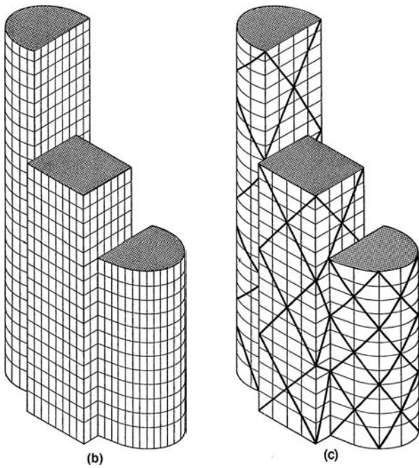
Figure 4.9. Bundled tube: (a) schematic plan; (b) framed bundled tube; (c) diagonally braced bundled tube.
