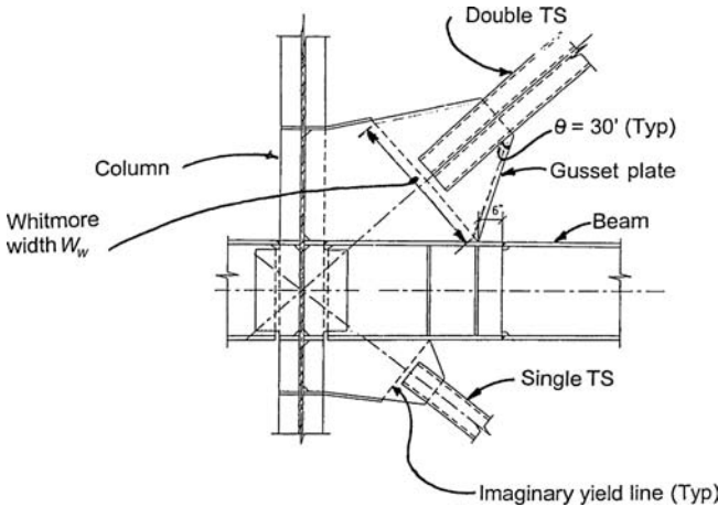
Figure 3.46. An SCBF connection detail at column. (Courtesy of Louis Choi, S.E., John A. Martin & Associates Structural Engineers, Los Angeles, CA.)
