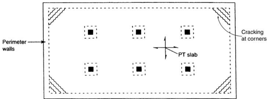
Figure 7.28. Cracking in post-tensioned slab caused by restraint of perimeter walls.
