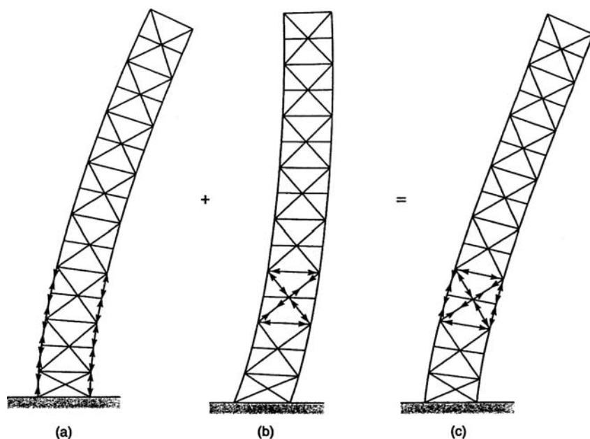
Figure 3.5. Braced frame deformation: (a) flexural deformation; (b) shear deformation; (c) combined configuration.
