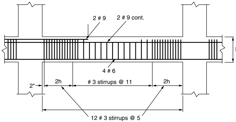
Figure 4.36. Design example, frame beam; intermediate moment frame.
