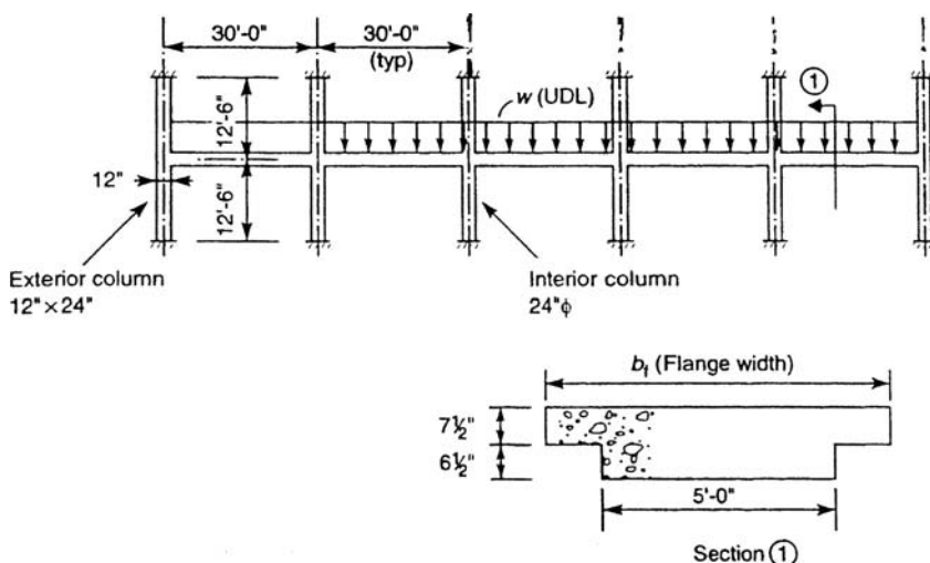
Figure 7.42. Example 2: post-tensioned beam, dimensions and loading.
