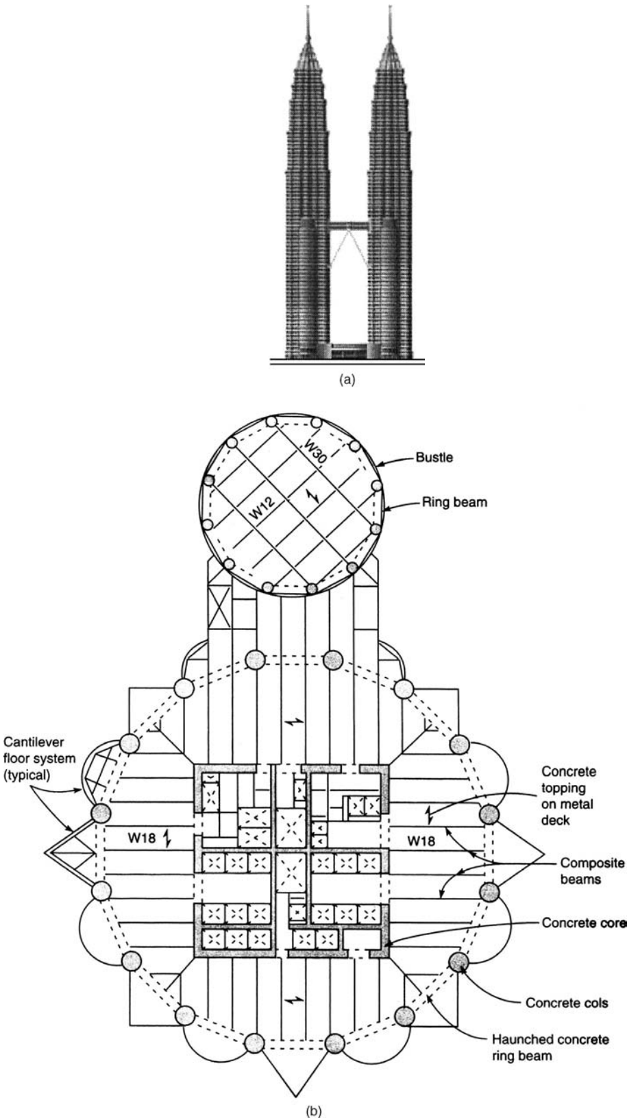
Figure 8.12. Petronas Twin Towers, Kuala Lumpur, Malaysia: (a) elevation; (b) structural system plan.
