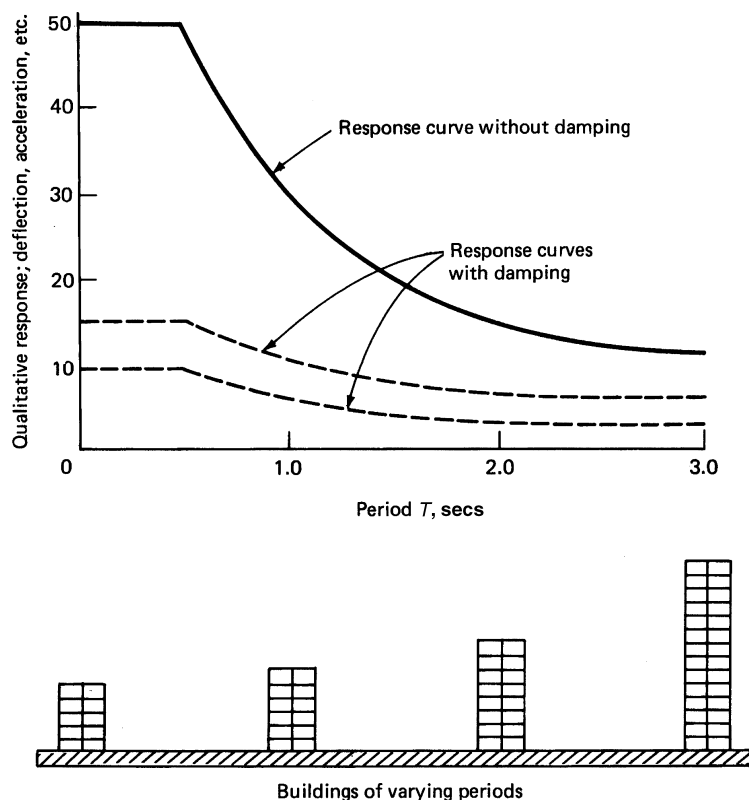
Figure 2.16. Concept of response spectrum.
