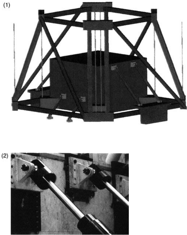
Figure 8.30h. (1) Simple pendulum damper; (2) Hydraulic dampers attached to mass block. (Photograph courtesy of Dr. Peter Irwin of Rowan, Williams, Davis, & Irwin, Inc., Guelph, Ontario, Canada.)
