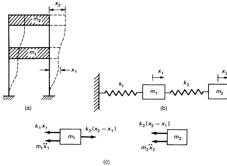
Figure 2.71. Two-story shear building; free vibrations: (a) building with d masses; (b) mathematical model; (c) free-body diagram with d masses.
