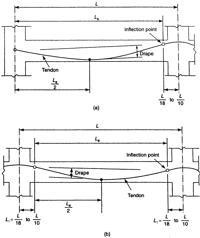
Figure 7.36. Tendon profile: (a) typical exterior span; (b) typical interior span.
