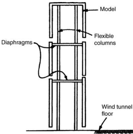
Figure 1.26. Flexible aeroelastic model (schematic cross section).
