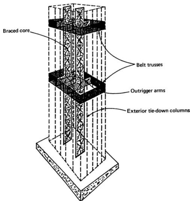
Figure 3.27. Schematic structural system for a building with two outriggers and belt trusses.
