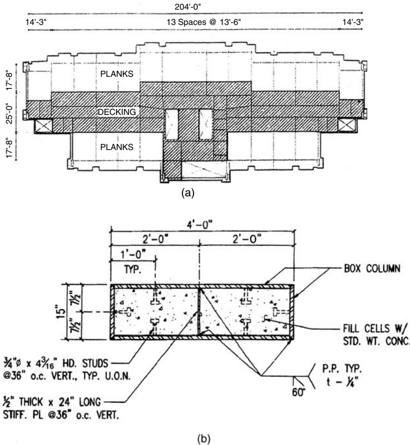
Figure 5.44. Kalia Towers, Waikiki, HI; (a) Typical floor plan; (b) box column plan section; (c) brace-to-box column connection; (d) construction photo. (The tower utilized a composite system composed of steel beams with a 6"-thick precast, prestressed concrete plank in the guest rooms, and metal deck with steel beams in the corridors. The lateral system was a braced frame with composite box columns filled with concrete.) Photograph and figures courtesy of Gary Y. K. Chock, S.E., Martin & Chock Inc., Honolulu, HI.
