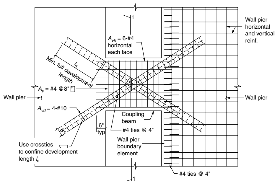
Figure 4.49. Coupling beam with diagonal reinforcement. Each diagonal reinforcement must consist of at least four bars with closely spaced ties. Use wider closed ties or crossties at central intersection. Use crossties to confine development length \ell_d .
