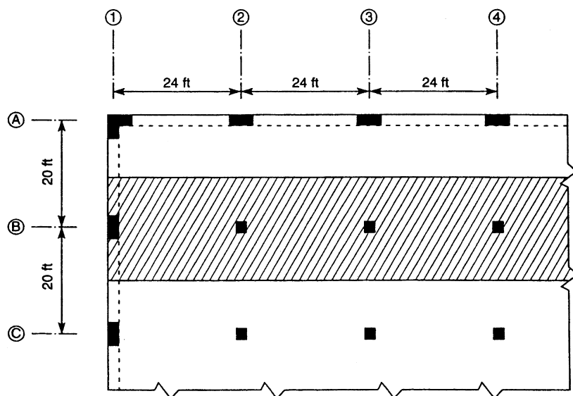
Figure 7.19. Design example, two-way slab.
