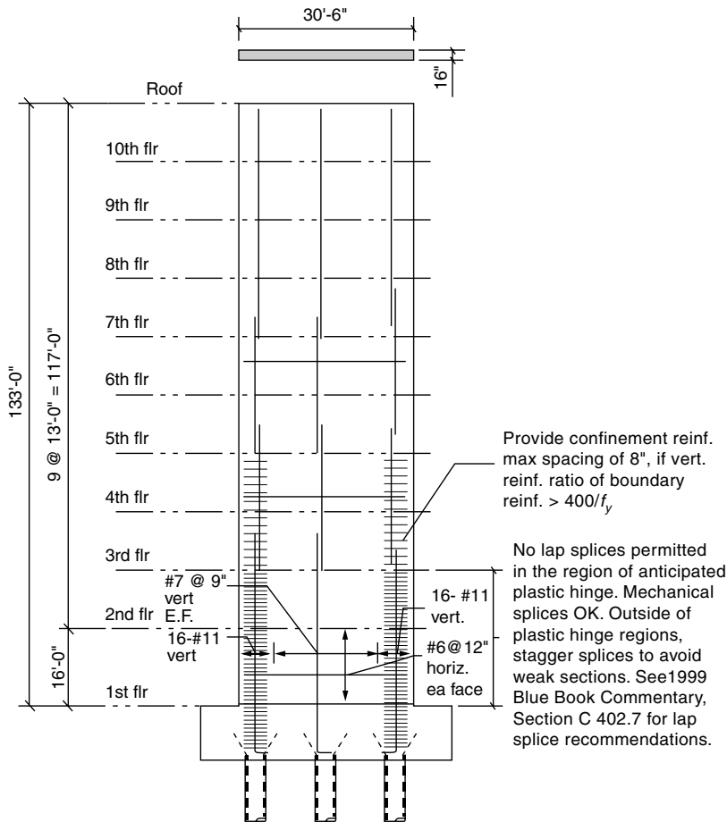
Figure 4.45. Wall elevation showing schematic placement of reinforcement.
