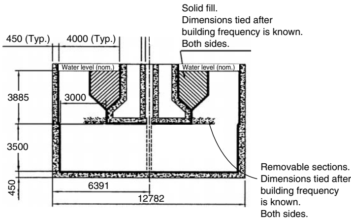
Figure 8.30f. TLCD for Wall Center, Vancouver, British Columbia. The motions of the tower were primarily in one direction only. Therefore only one direction needed to be damped. Two TLCDs extend nearly the full width of the tower. Within each tank is a long horizontal chamber at the bottom and two columns of water at each end. The dampers work by allowing the water to move back and forth along the bottom chamber of the tank and up into the columns of water.
