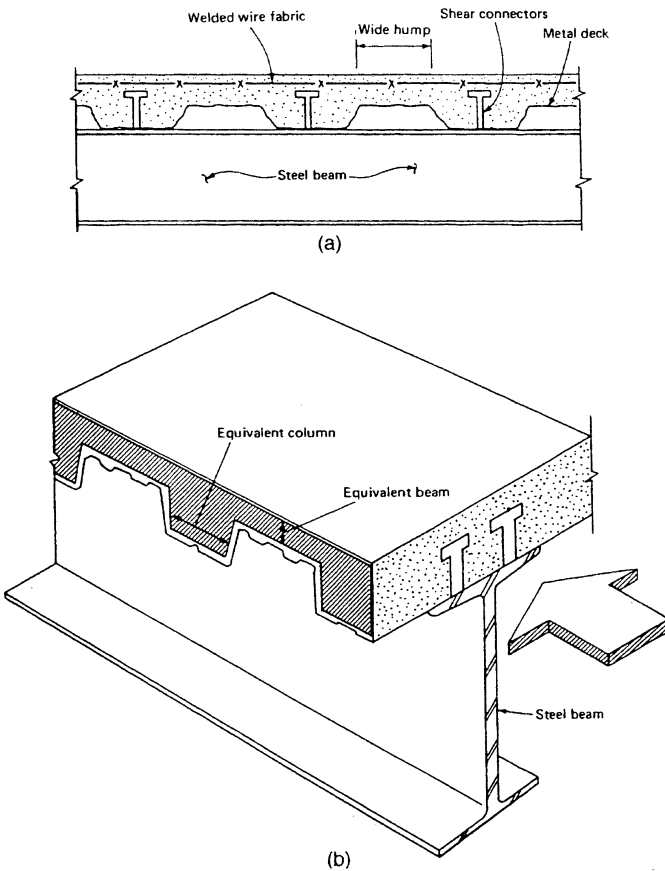
Figure 7.50. (a) Composite beam with wide hump metal deck; (b) simplified analytical model of composite metal deck subjected to horizontal shear.
