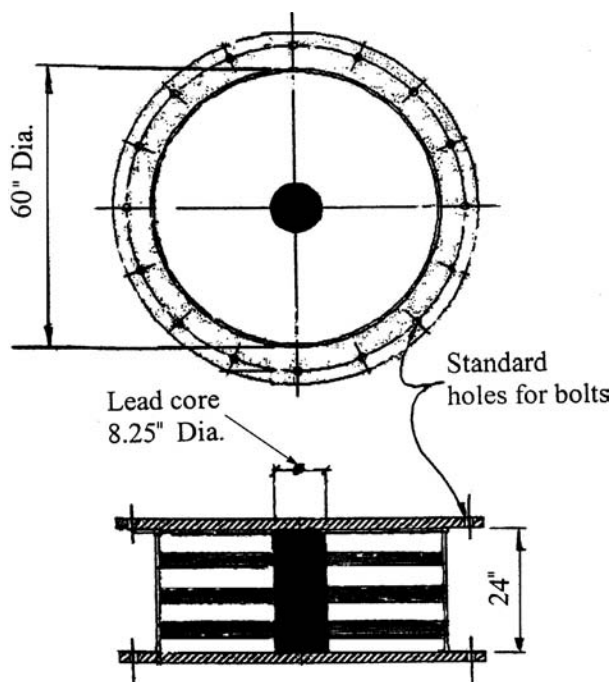
Figure 8.34g. Lead-rubber bearing (LRB) for an interior column of a five-story steel framed building; approximate dimensions.
