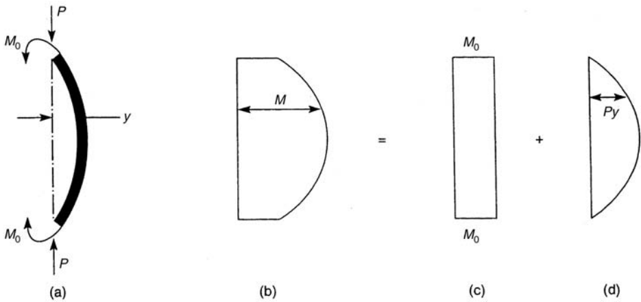
Figure 7.7. Moments in beam–columns: (a) column subjected to simultaneous axial load and bending moments; (b) combined moment diagram; (c) moment diagram due to equal end moments M_0 ; (d) moment due to P\Delta effect.
