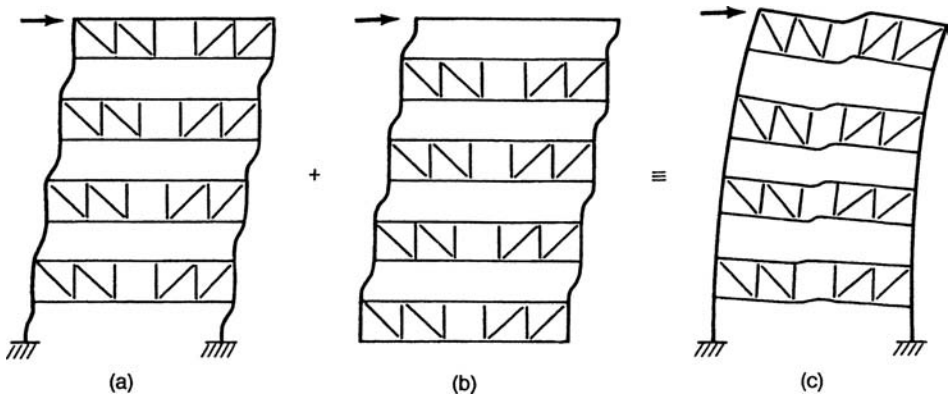
Figure 3.13. Conceptual two-dimensional model for staggered truss system: (a, b) lateral deformation of adjacent bays; (c) overall behavior. Note the absence of local bending of columns.
