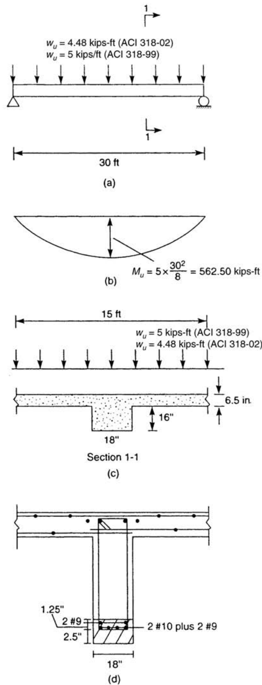
Figure 7.15. Design example, simply supported T-beam.
