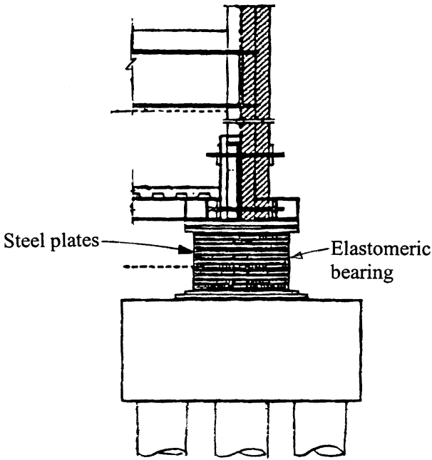
Figure 8.34e. High-damping rubber bearing, made by bonding sheets of rubber to thin steel plates. The steel plate increases vertical compressive stiffness of the unit while maintaining the desired low lateral stiffness.
