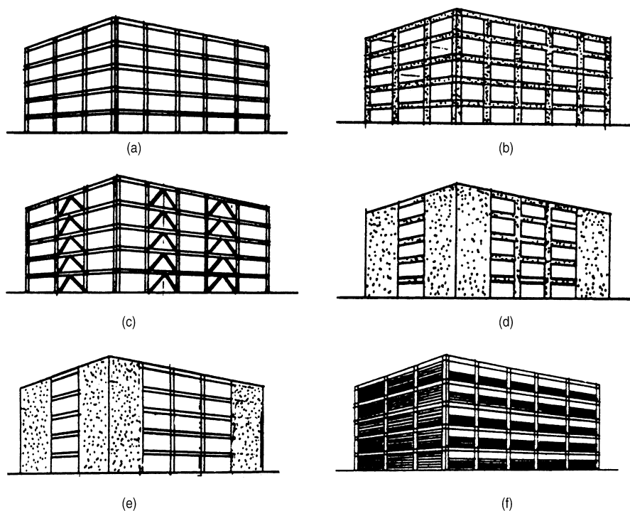
Figure 2.6. Lateral-force-resisting systems: (a) steel moment-resisting frame; (b) reinforced concrete moment-resisting frame; (c) braced steel frame; (d) reinforced concrete shear walls; (e) steel frame building with cast-in-place concrete shear walls; (f) steel frame building with in-filled walls of nonreinforced masonry.
