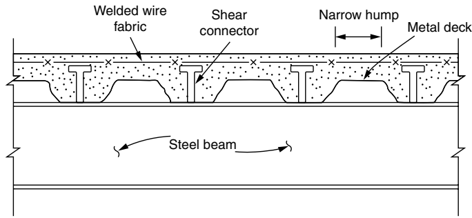
Figure 7.49f. Composite beam with narrow hump metal deck.
