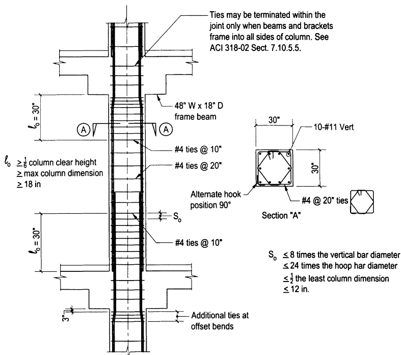
Figure 4.37. Design example, frame column; ordinary moment frame. Note: \ell_o is the same as for columns of SMRF. There is no requirement to splice the column bars at mid-height.
