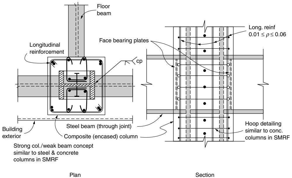
Figure 5.32. Composite special moment-resisting frames; composite perimeter frame column-to-frame beam connection detail.
