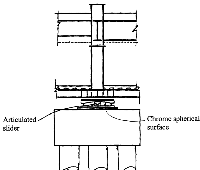
Figure 8.34h. Sliding bearing; friction-pendulum system (FPS). An FPS consists of an articulated slider that glides on a polished spherical concave chrome surface. Whereas in elastomeric base-isolated buildings P\Delta effects are equally distributed between superstructure and foundation, in sliding base-isolated buildings the entire P\Delta effect can be accommodated in either the superstructure or the foundation, depending on whether the spherical surface is attached to the foundation or the superstructure.
