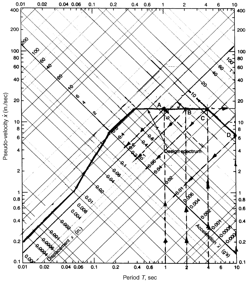
Figure 2.25. Velocity, displacement, and acceleration readout from response spectra.
