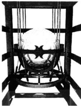
Figure 8.30i. Spherical damper, Taipei Financial Center, Taiwan. A 20-ft (6-m)-diameter steel ball assembled on site in layers of 5-in. (12-cm)-thick steel plate is suspended from level 92 by four sets of cables. Eight hydraulic pistons, each 6.5 ft (2 m) long, attached to the ball, dissipate dynamic energy as heat.
