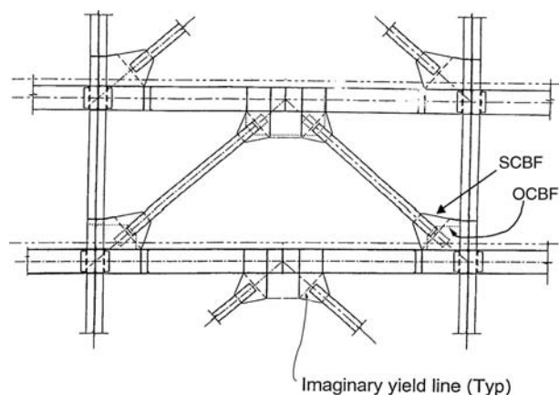
Figure 3.45. Schematic elevation of an SCBF showing imaginary yield lines in gusset plates. Also shown are the gusset plates for an OCBF. Observe the substantial increase in gusset plate sizes required for the SCBF. (Courtesy of Louis Choi, S.E., John A. Martin & Assoc. Structural Engineers, Los Angeles, CA.)
